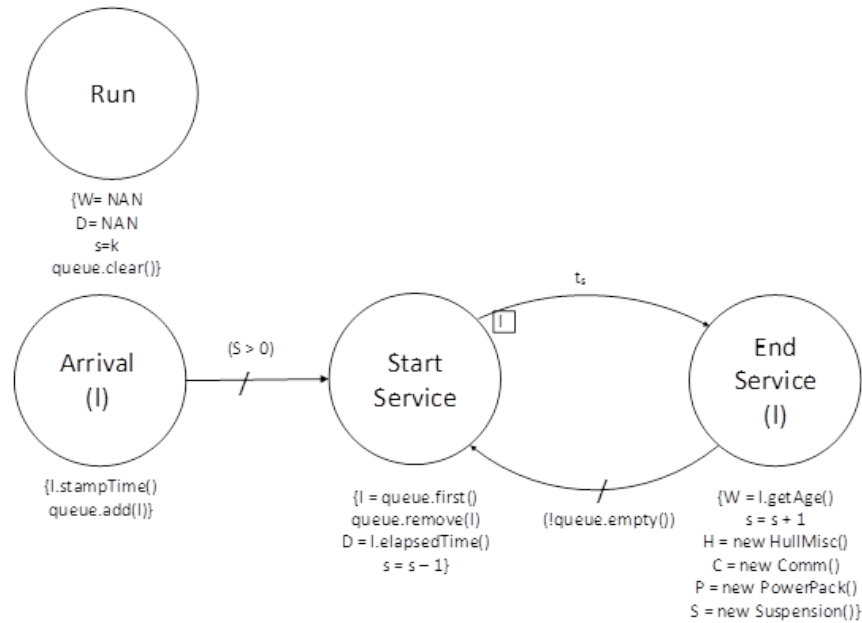
Figure 6. LAVDisassemblyServer Event Graph
