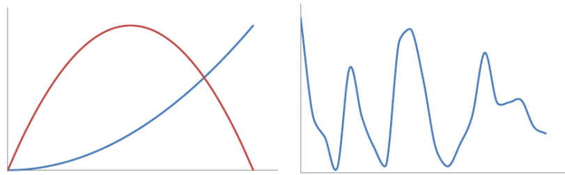
Figure 2. Continuous/Time-Step State Trajectory. Source: Buss (2017).
