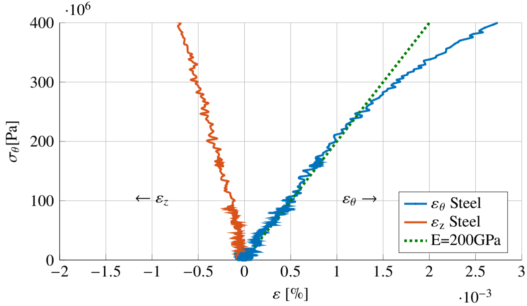
Figure 7.5. Steel cylinder experimental results
