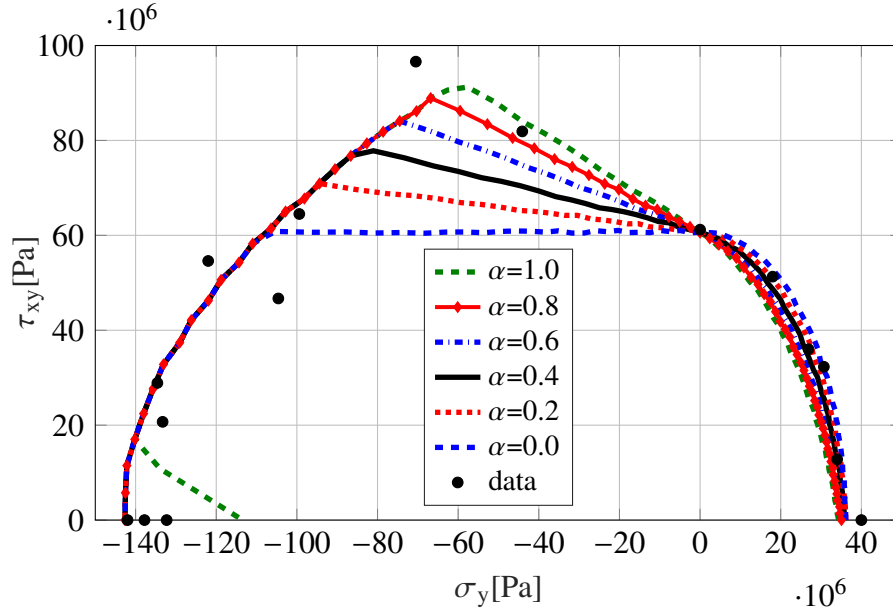
Figure 6.3. Effect of choice of \alpha_1 for E-Glass/LY556 under \sigma_y and \tau_{xy}
