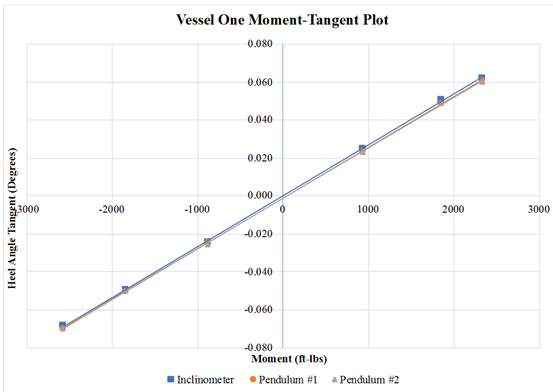
Figure 8. Moment-Tangent Plot of Vessel One Raw Data
