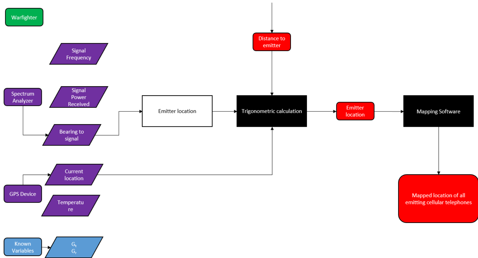
Figure 24. Location mapping and output section of algorithm
