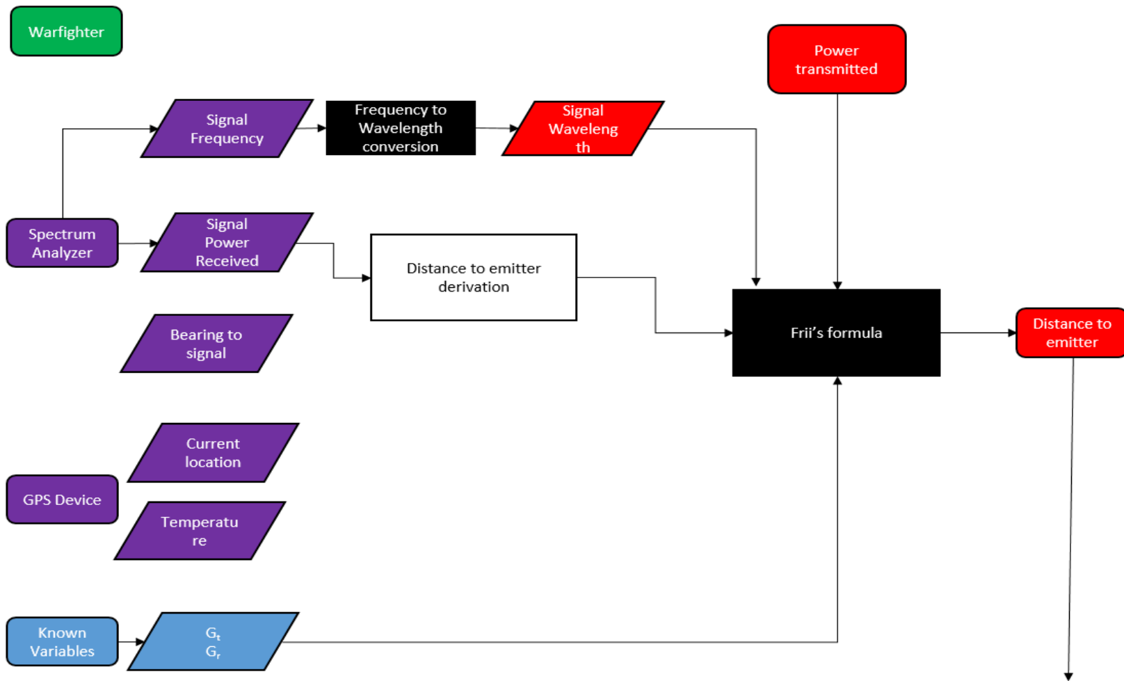
Figure 23. Distance to emitter section of algorithm
