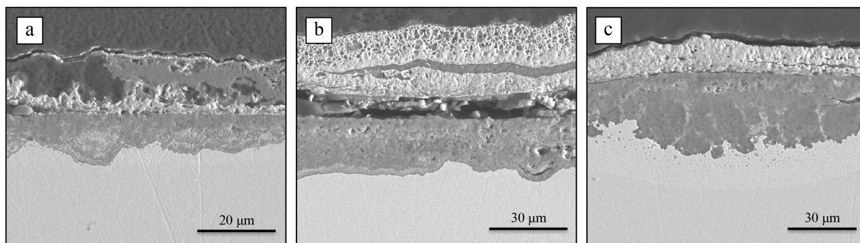
Figure 14: Ni-36Al-5Cr after 20 h exposure to Na 2 SO 4 in O 2 -SO 2 at 700°C, SEM (BSE) images. (a) to (c) represent the different corrosion product thicknesses observed on the same sample.
