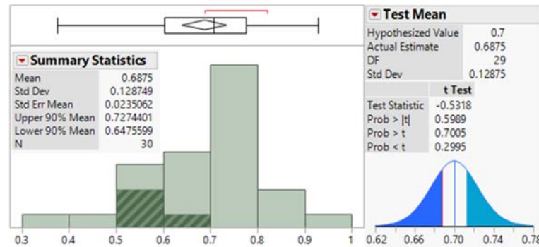
Figure 14. Descriptive statistics on the percent of optimal decisions and t -test results
