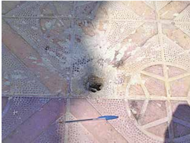
Image 8. M Series DPICM impact pattern on a tiled hard surface, showing the central hole made by the shaped charge, southern Lebanon, August 2006. Note that the fragmentation pattern is broadly similar to a fin-stabilized submunition, but the shaped charge will likely produce a larger hole at the base of the pattern. Photo courtesy of Steve Priestley.
