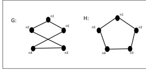
Figure 2.5. Isomorphic Graph Examples. Adapted from: [17].
