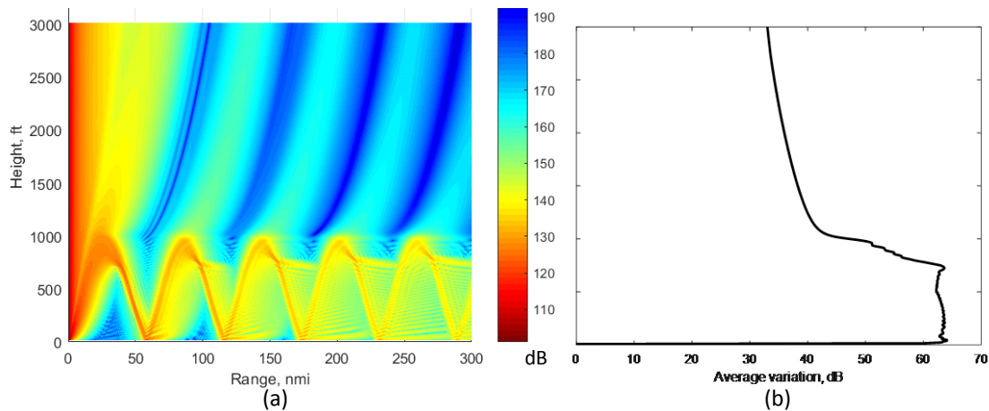
Figure 7. (a) Atmospheric loss data with ducting and (b) result of simulated measurements showing evidence of a duct.
