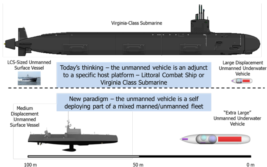
Figure 14. Current paradigm ( top ) envisions unmanned vehicles as adjunct to a specific host platform such as an LCS or Virginia Class submarine. The new paradigm ( bottom ) envisions self-deploying fully autonomous unmanned vehicles teaming with diverse manned platforms.
