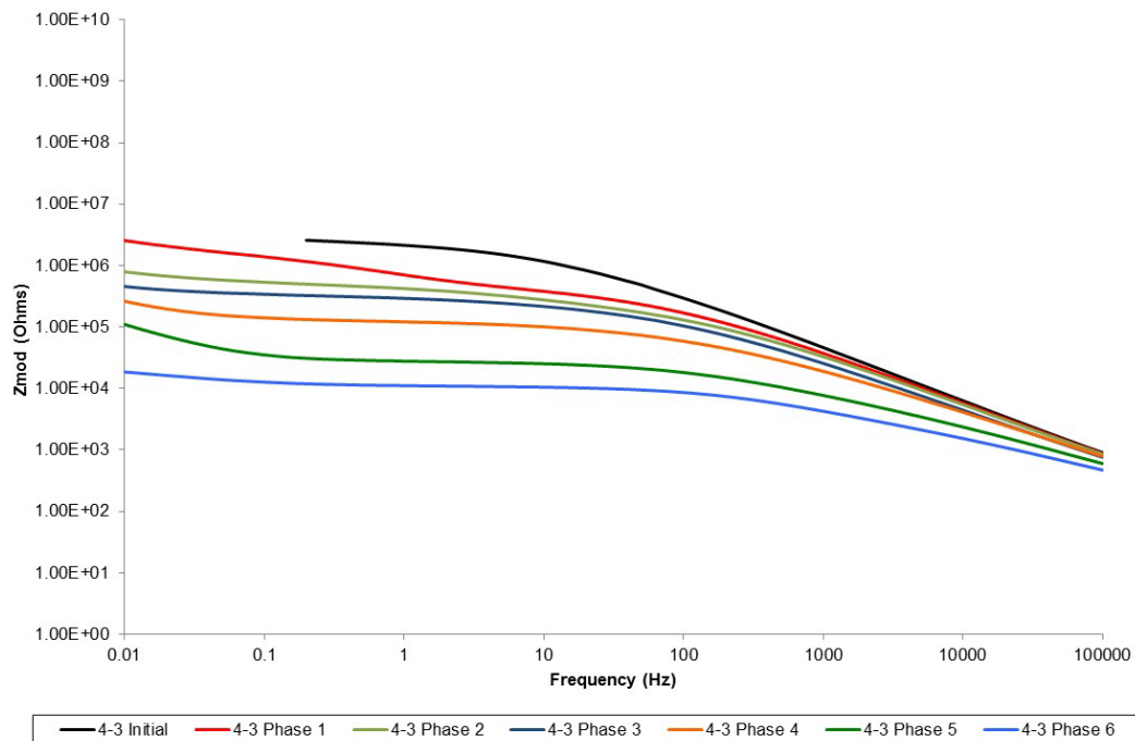
Fig. 30 EIS Bode plots for steel with MIL-DTL-53030 and MIL-DTL-64159 (System D) following modified ASTM B117 exposure
