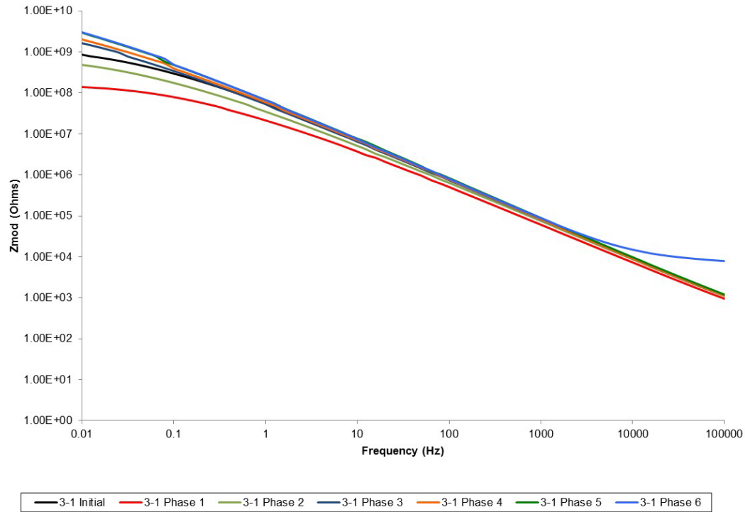
Fig. 26 EIS Bode plots for steel with MIL-DTL-53022 and MIL-DTL-64159 (System C) following modified GMW14872 exposure
