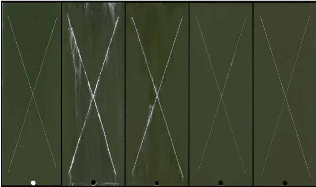
Fig. A-7 Aluminum panels with coating System C following 24 months Florida outdoor, 4032 h ASTM B117, 14 phases modified ASTM B117, 12 phases modified ASTM G85, and 12 phases modified SAE J2334
