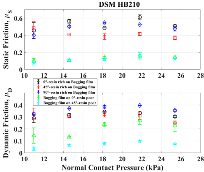
Fig. 18 Static and dynamic coefficients of friction vs. normal contact pressure for Dyneema HB 210 on Stretchlon 800 bagging film
