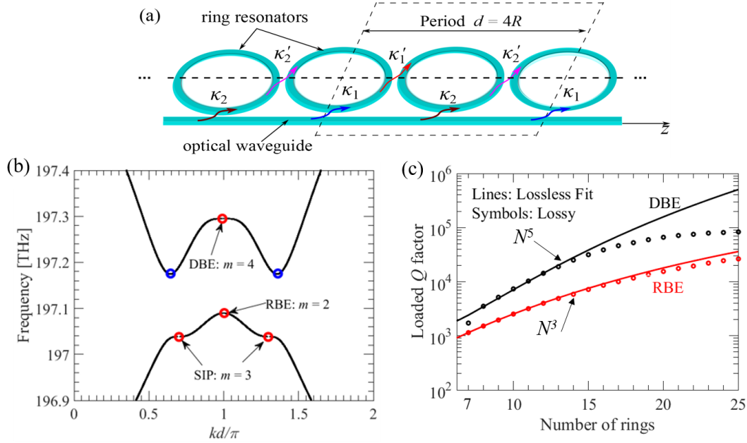
Fig. 12. (a) The proposed CROW is consisting of a chain of coupled ring resonators optical waveguides of radius R side coupled to a rectangular straight waveguide. (b) The Floquet-Bloch wavenumber dispersion diagram of the CROW unit cell shown in (a), viewing three different kinds of EPDs within a narrow frequency band: an RBE, a DBE; and an SIP. (c) The calculated loaded quality factor ( Q ) of a finite CROW plotted versus the number of rings for the lossless and lossy CROW.
