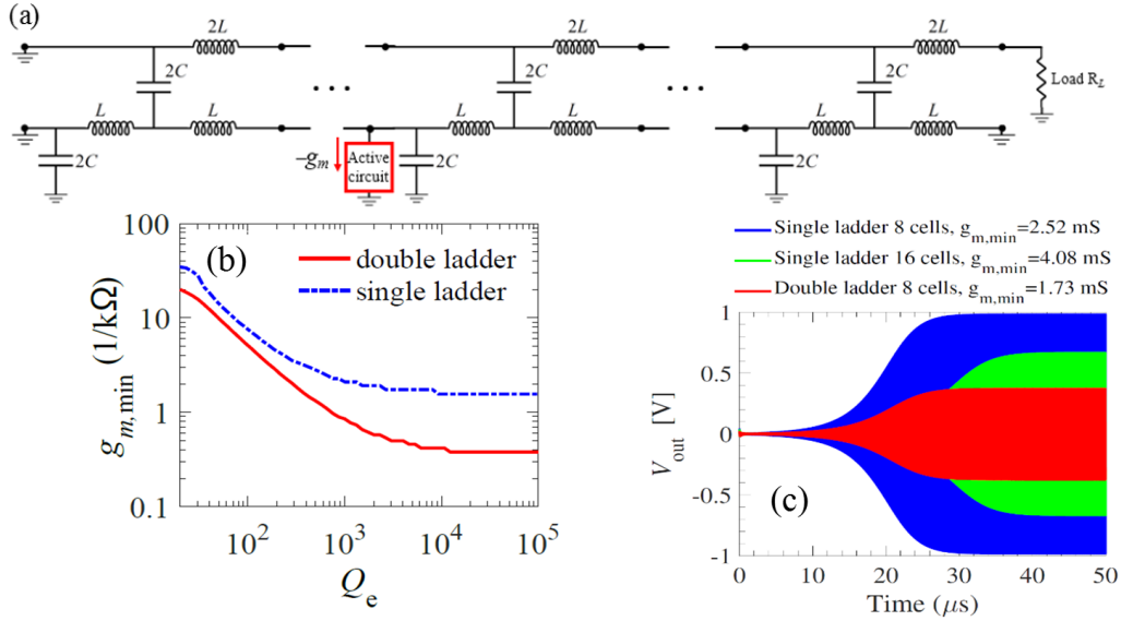
Fig. 10. (a) Double ladder periodic oscillator structure that supports a DBE. It has 8 unit cells with terminations and negative resistance ( -g_m ) acting as the active device (b) Minimum g_m needed start oscillations versus different values for quality factor of elements ( Q_e ) for double and single ladder structures. The double ladder needs lower g_m to start oscillation. (c) Oscillation behavior for three different cases of single-ladder and double-ladder circuits in comparison and the minimum g_m needed to start oscillation. All data is reported in [15].
