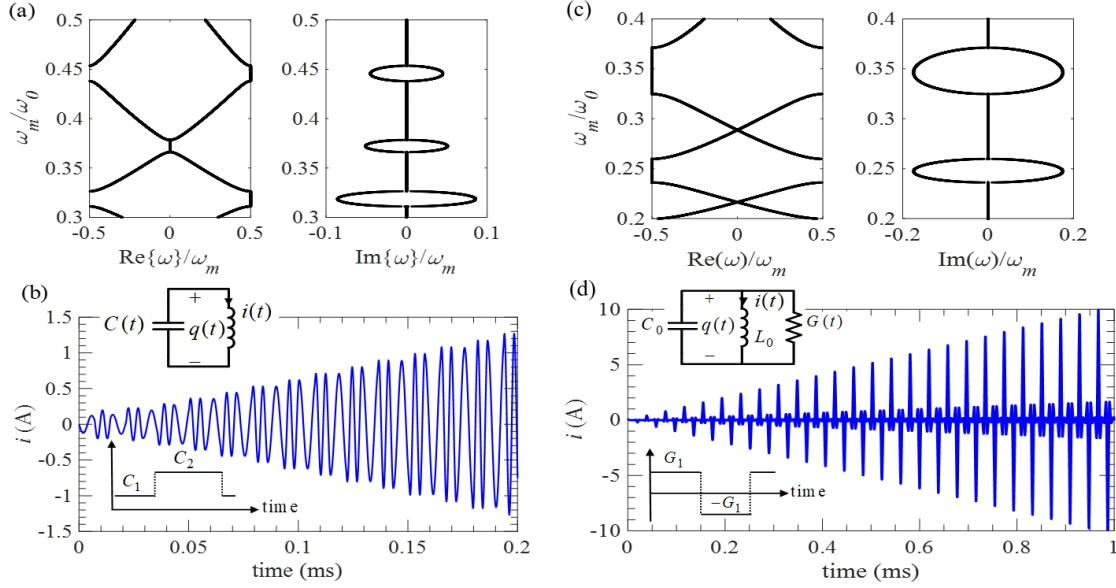
Fig. 16. (a) and (c) Real and imaginary parts of dispersion diagram of the eigenfrequencies versus the normalized angular modulation frequency of the resonators depicted in (b) and (d), respectively. (b) and (d) The linear algebraic growth of the inductor current at an EPD for an LC resonator with time-varying capacitor and for an RLC resonator with time-varying conductance, respectively.
