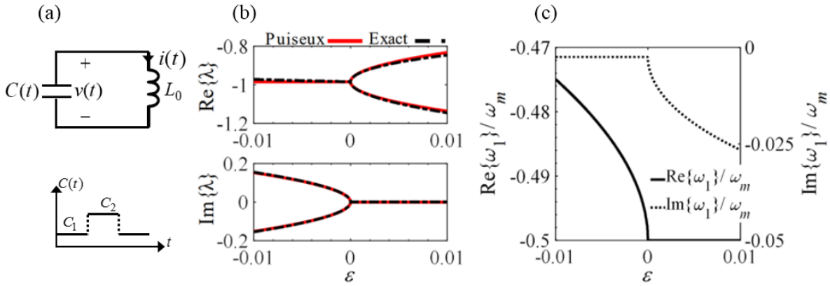
Fig. 17. (a) LC resonator with a periodic time varying capacitor exhibits a 2 nd order EPD; (b) change of the eigenvalues due to perturbation in the capacitor value C_2 and (c) change in the complex resonance frequency \omega_1 corresponding to the change in the eigenvalue in (b). A +0.1% perturbation in the dielectric permittivity of the capacitor C_2 implies a 76% change in the quality factor of the resonator, demonstrating the exceptional sensitivity.
