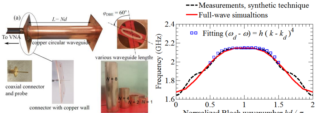
Fig. 11. (Left) Fabricated waveguide that develops a DBE at S-band. (Right) Dispersion relation showing good agreement between both measurement and full-wave simulations using CST microwave studio.
