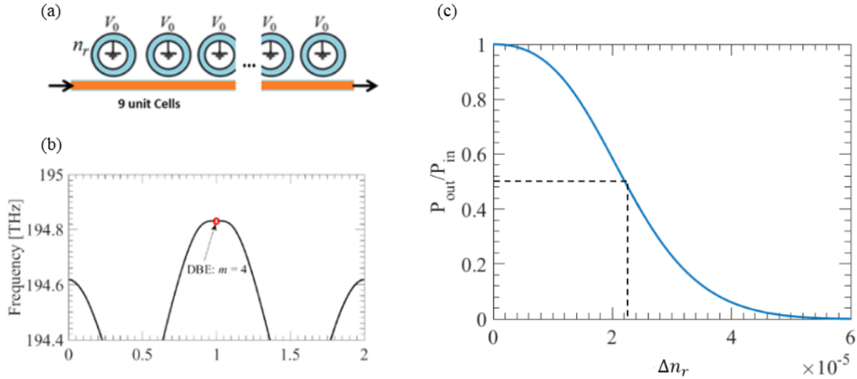
Fig. 19. (a) The proposed CROW is consisting of a chain of coupled ring resonators that are side-coupled to a uniform optical waveguide. (b) The dispersion diagram of the CROW unit cell showing a 4 th order EPD f_e = 194.8 THz and (c) power transfer function of the proposed structure in (a) versus change in the refractive index of the rings.
