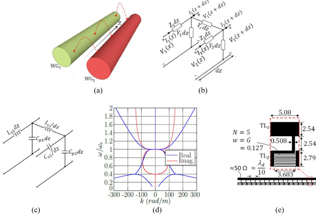
Fig. 4. (a) Two uniform coupled waveguides. (b) Generalized distributed circuit model for infinitesimal section of the two coupled transmission line (CTL) structure. (c) The per unit length parameters of two uniform coupled transmission lines (CTLs) where one supports forward propagating mode and the other supports evanescent mode. (d) The dispersion diagram of the CTLs showing both the real and imaginary parts of the wavenumbers of the four supported eigenmodes where the DBE can be seen at k = 0 . (e) A microstrip sub-wavelength implementation of the CTLs in (c) with period d=5.08\text{mm} and EPD frequency f_e = 5\text{GHz} . All the given dimensions in (e) are in mm.
