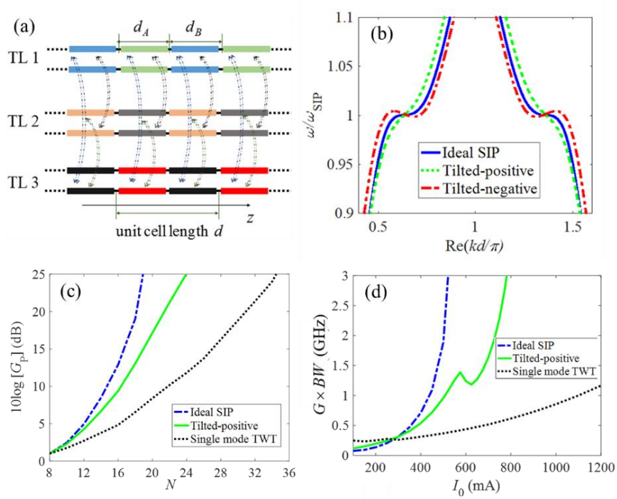
Fig. 23. (a) Schematic of a periodic coupled transmission line (CTL) consisting of three lines and two segments A and B in each unit cell having internal coupling through distributed inductance and/or capacitances (b) Dispersion relation of an infinitely long periodic coupled transmission line having SIP at angular frequency \omega_{SIP} for three different cases of: ideal (zero slope), positive slope, and negative slope at SIP region. (c) Power gain (in dB) of the proposed ideal SIP and tilted-positive regimes of TWT operation, compared with a standard regime of amplification based on a finite, periodic TL, modeling a single mode TWT, having the same characteristic impedance and loading plotted versus the number of SWS unit cells, N . (d) Comparison of the gain-bandwidth product ( G \times BW ) of TWT amplifiers based on SWS regimes based on ideal SIP and tilted-positive dispersion, versus electron beam current I_0 . Results are also compared with a TWT made of a SWS with only one periodic TL (single mode TWT) having the same length and average characteristic impedance.
