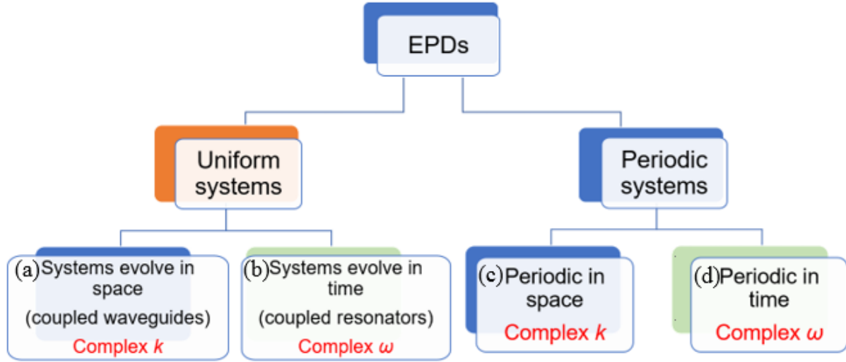
Fig. 1. Classification of the different structure-topologies that can exhibit exceptional points of degeneracy (EPDs). (a,b) Uniform electromagnetic systems means two kind of systems: those invariant in space (i.e., waveguides) and systems that are invariant in time (resonators). Box (c) is about periodic waveguides. Box (d) is about EM systems that are periodically time modulated. During this project new EM structures expressing EPDs under each of these cases have been found.
