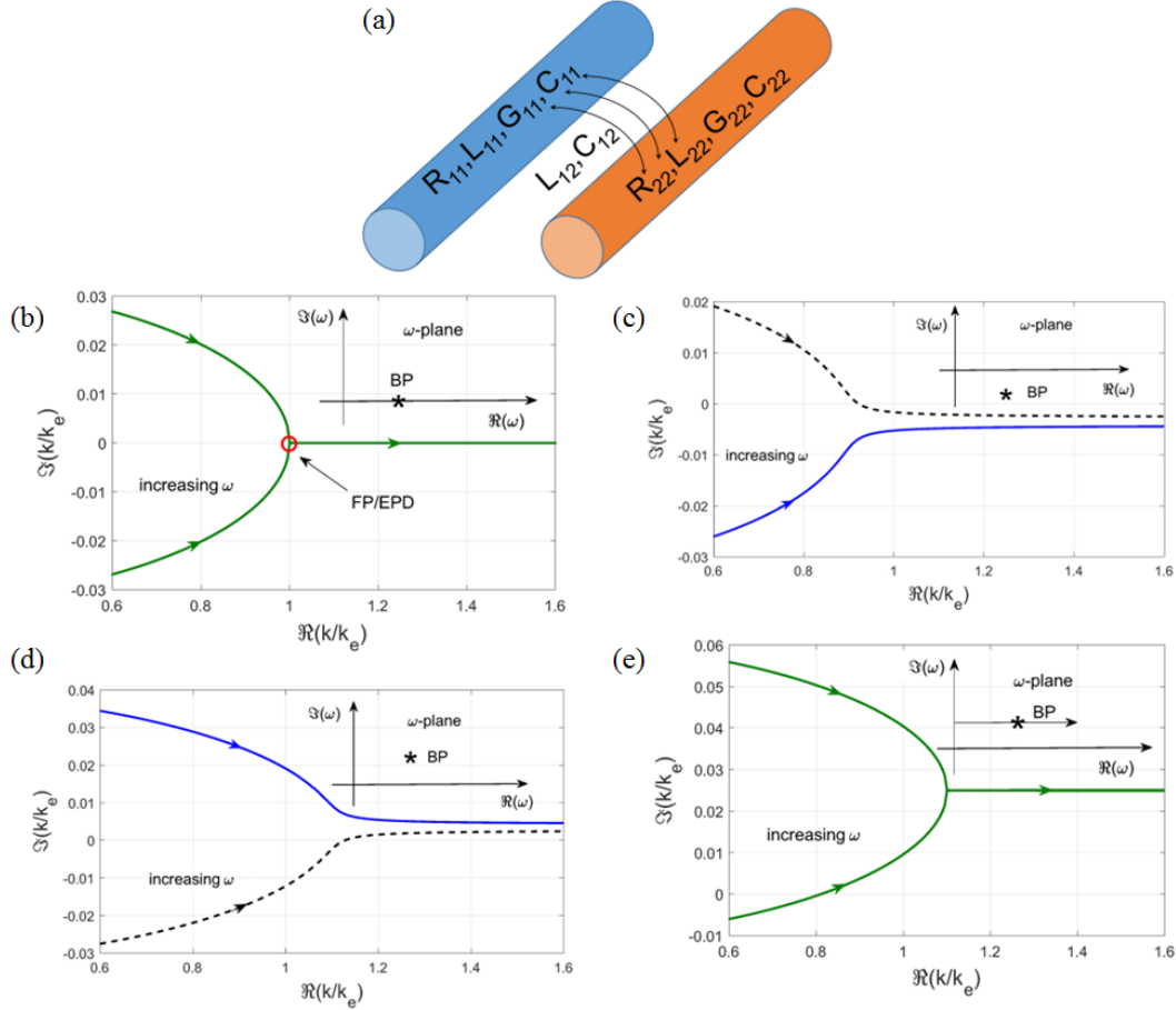
Fig. 3. (a) Two coupled transmission lines with mutual capacitive and inductive coupling, invariant along- z . Dispersion behavior near an EPD for coupled transmission lines in (a) with (b) R_{11} = -R_{22} = -73.172 ohms (PT-symmetric case), as \omega varies from 0.5 \omega_e to 1.5 \omega_e along the real- \omega axis. (c) Same as (b) but for R_{11} = -1.2 R_{22} , where the EPD lies above the real-frequency axis. (d) Same as (b) but for R_{11} = -0.8 R_{22} , such that the EPD is below the real-frequency axis. (e) Same as (a) but for \text{Re}(\omega) varying from 0.5 \omega_e to 1.5 \omega_e at a constant value \text{Im}(\omega) = \text{Im}(\omega_s) = (0.022 \omega_e) . In all cases the pair (k_e; \omega_e) are the values at PT-symmetry, (k_e; \omega_e) = (28.649 \text{ m}^{-1}; 2\pi 10^9 \text{ s}^{-1}) , R_{22} = 73.172 ohms, and the star indicates the BP/EPD.
