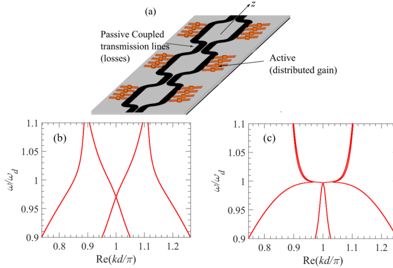
Fig. 8. (a) Example geometry of coupled microstrip lines with distributed gain and “loss” (loss is actually a distributed radiation, that is seen as a loss from the circuit point of view). (b) The dispersion diagram for the “lossy” structure (i.e. before introducing gain) where losses are modeled as series resistance R_n such that all TLs have Q_{TL} = 100 (see [18]). (c) The corresponding dispersion diagram after introducing the appropriate gain associated to the minimum hyperdistance (i.e. gain is modeled by introducing negative shunt conductance in all TLs) to achieve balanced gain and loss condition, showing the flatness of 4 th order EPD. This microwave circuit may be used as an efficient high intensity radiator, generating high spectral purity with high power efficiency.
