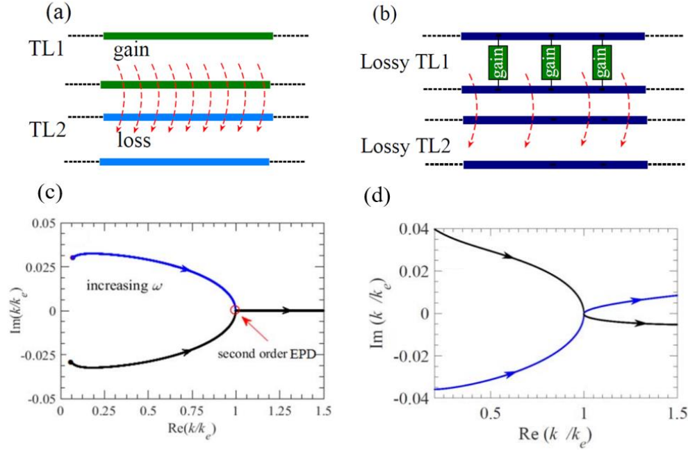
Fig.2. Configurations of uniform CTLs that may exhibit EPD. (a) Uniform CTL with distributed and symmetric gain and loss (PT-symmetric). (b) Uniform CTL with distributed loss in both TLs and gain in only one (non PT-symmetric). (c) and (d) Trajectory of complex k in the \text{Re}(k) - \text{Im}(k) plane varying as a function of \omega near a second-order EPD for the two configurations in (a) and (b), respectively (see [7]).
