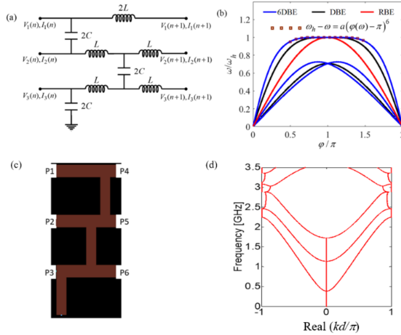
Fig. 14. (a) Unit cell of a periodic triple-ladder lumped circuit that develops a sixth order degeneracy at an angular frequency \omega_h = 1/\sqrt{LC} (b) Dispersion diagram of the infinitely long periodic triple-ladder circuit exhibiting a 6DBE at angular frequency \omega_h . (c) Microstrip implementation unit cell of a periodic CTL in (a) that develops a sixth order degeneracy (d) Dispersion diagram showing the real part of the dispersion of the infinitely long periodic structure of unit cell in (c) exhibiting 6 th order EPD at frequency = 2.85 GHz.
