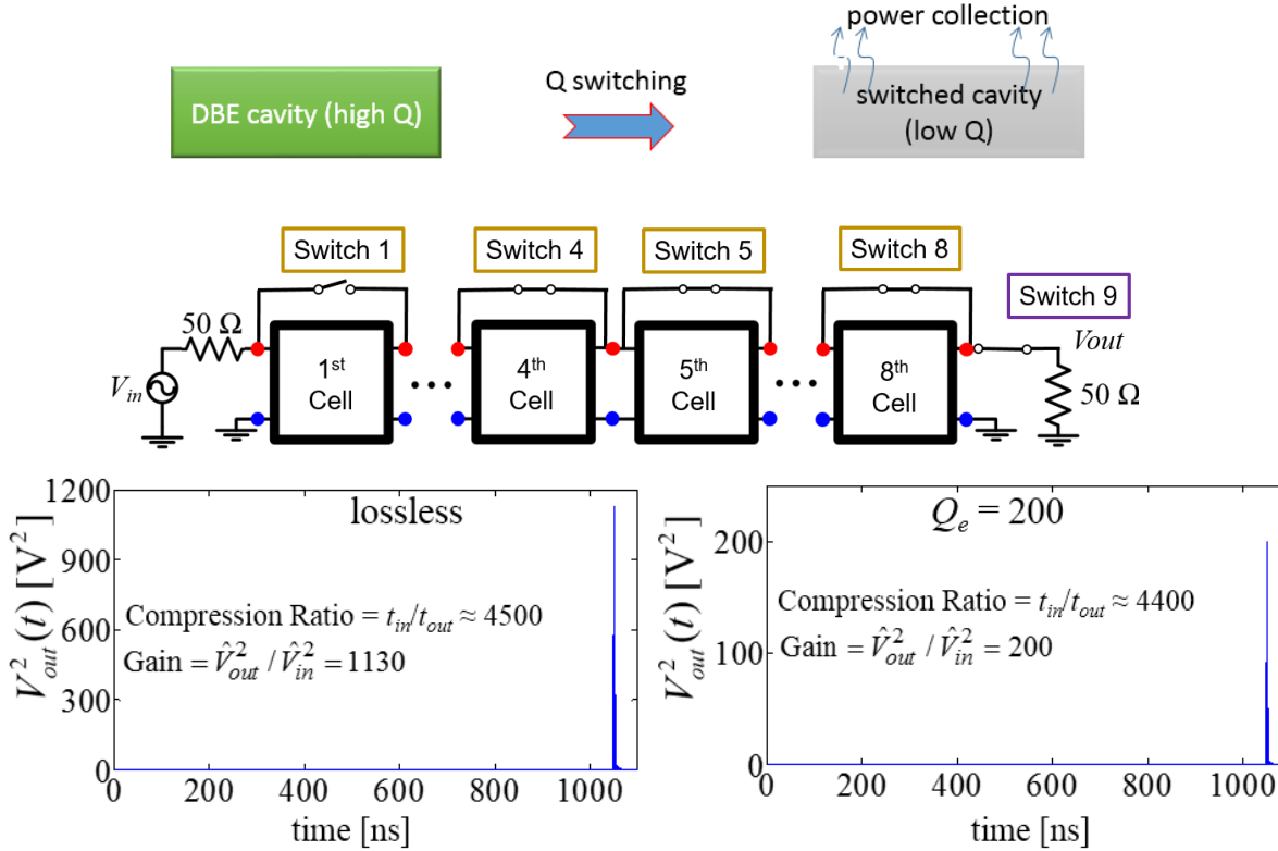
Fig. 22. (Top) Conceptual framework for a pulse compression device based on EPD and Q-switching, proposed in [C12]. (Middle) Schematic of a DBE resonator made of 8 unit cells with controlled switches that switch the high Q DBE cavity into a low-Q cavity for which energy can be extracted by shorting the switches on the upper line. (Bottom) Output load squared voltage for two cases of lossless and lossy DBE structures in which the compression ratio is \sim 4500 and a gain of at least 200 when losses are considered ( Q_e is the element Q factor equal to 200).
