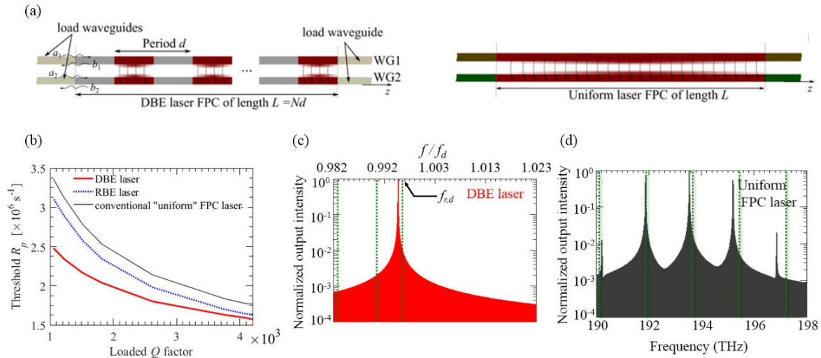
Fig. 20. (a) Schematic representation of an FPC with DBE(Left) composed of a finite number of periodic unit cells, each made of a coupled and an uncoupled section and the conventional uniform FPC(Right). (b) Comparison between the lasing threshold pumping rate of the proposed DBE laser with the conventional uniform FPC and the RBE lasers of equal length. (c) and (d) output spectrum of the DBE laser and the long uniform FPC laser at the same pumping rate, respectively.
