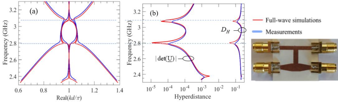
Fig. 6. (a) Dispersion relation and (b) hyperdistance measurement versus full-wave simulation of the unit cell of a periodic CTL exhibiting a 4 th EPD. The results show that the 4 th order EPD occurs at 2 different frequencies in the range shown in this plot. Full-wave simulations are performed with Keysight ADS using the method of moments (MoM).
