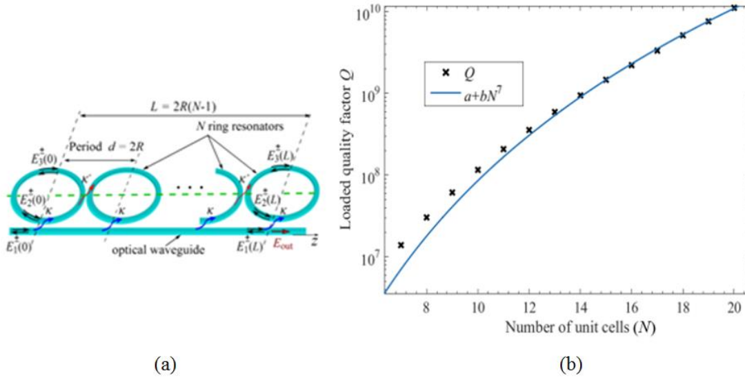
Fig. 15. (a) Loaded CROW consists of a chain of rings coupled to each other. (b) Loaded quality factor ( Q ) of the lossless EPD-CROW calculated at different number of unit cells N . The values of Q denoted by cross symbols are calculated using the group delay method while the solid line represents the fitting curve with the equation a + bN^7 .
