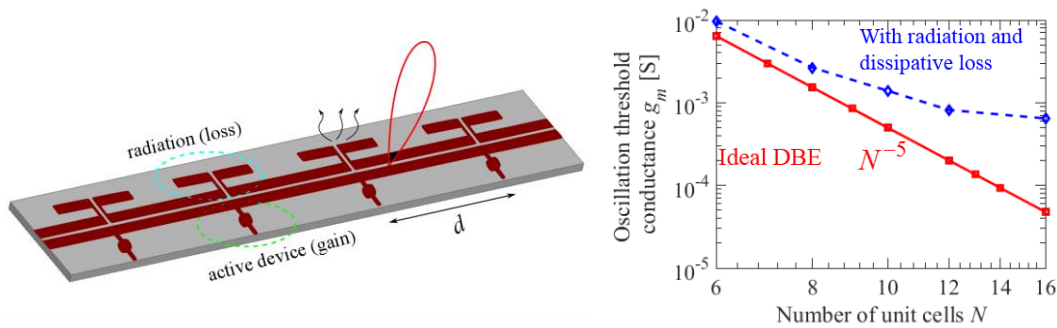
Fig. 21. (Left) Configurations of CTLs that exhibit exceptional points of degeneracy (EPD) based on coupled transmission lines (CTL) with gain and loss, [C1], [C25]. The CTL is loaded with gain and loss in the form of active devices and radiating antennas, respectively. (Right) The minimum amount of the gain conductance per unit cell required to start oscillations is shown to exhibit a unique trend typical of the DBE, by increasing the number of the unit cells.
