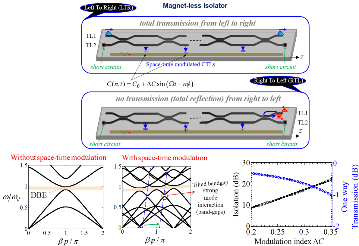
Fig. 24. (Top) Non-reciprocal coupled transmission lines (CTLs) with space-time modulations and EPDs, see [C13]. The two concepts intertwine to conceive a new class of a magnet-free isolators. (Bottom Left) Dispersion relation of periodically-coupled CTLs in the absence and presence of space-time modulations. (Bottom right) Transmission and isolation of the proposed EPD-based space-time modulated CTL showing non-reciprocity.
