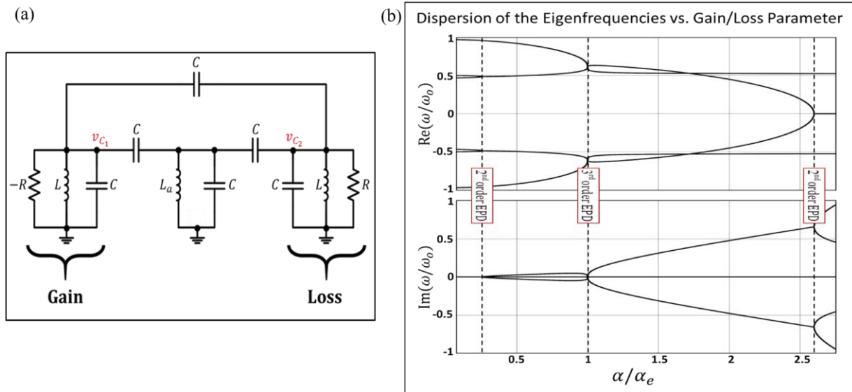
Fig. 5. (a) The proposed circuit to exhibit a third order EPD that consists of three coupled LC oscillators. (b) Dispersion diagram of the real and imaginary parts of the eigenfrequencies of the circuit (a) versus the normalized gain/loss parameter. The third order EPD is located at the point where three branches coalesce. Despite it is not shown here, the three associated eigenvectors coalesce as well.
