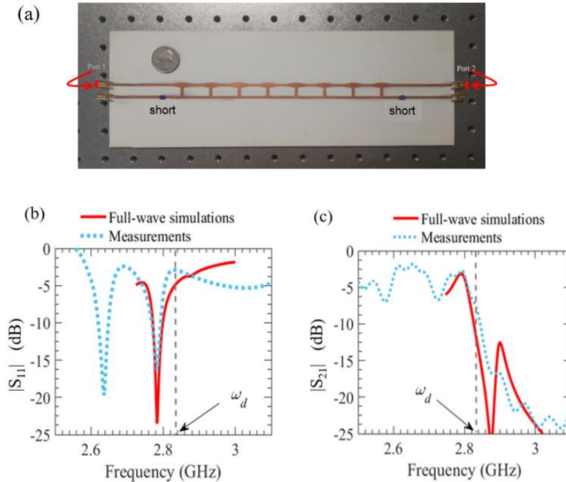
Fig. 7. (a) A fabricated microstrip 8 cell array with an EPD. The CTL is based on the unit cell shown in Fig. 6. (b-c) Simulations and measurements of the scattering parameters S_{11} (b) and S_{21} (c) for an 8-unit-cell array; where a good agreement between full-wave simulations and measurements is clear at the resonance frequency associated with the EPD.
