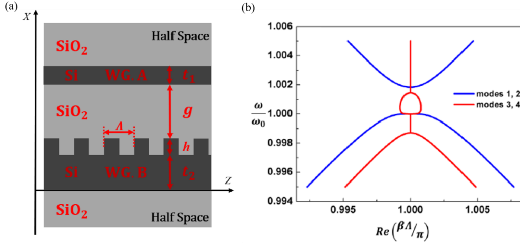
Fig. 9. (a) Proposed multi-layer waveguide structure with grating exhibiting a DBE. (b) The dispersion diagram of such structure based on coupled mode theory formulation showing a DBE, i.e., the coalescence of four eigenvalues. Though not shown here, at that frequency also the four eigenvectors (polarization states) are coalescing.
