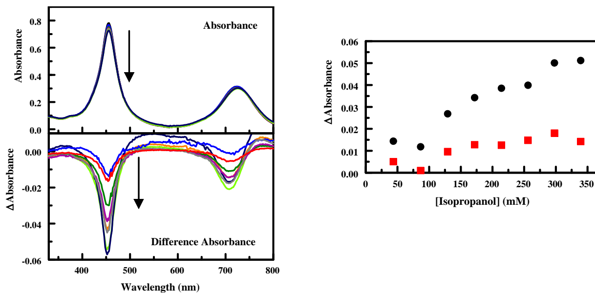
Figure A-26. Absorbance spectra (top) of \text{YN}_4\text{TPP} ( 9.86 \mu\text{M} ) in the absence and presence of increasing concentrations of isopropanol: 43, 86, 129, 171, 214, 256, 298, and 339 mM. Arrows indicate increasing target concentration. Absorbance spectra have been corrected for dilution resulting from target addition. Difference absorbance spectra (bottom) are calculated as porphyrin + target minus porphyrin. The concentration dependence of features in the absorbance spectra is also presented (right). Here, the change in absorbance at the trough positions (456 and 712 nm) is plotted against target concentration.
