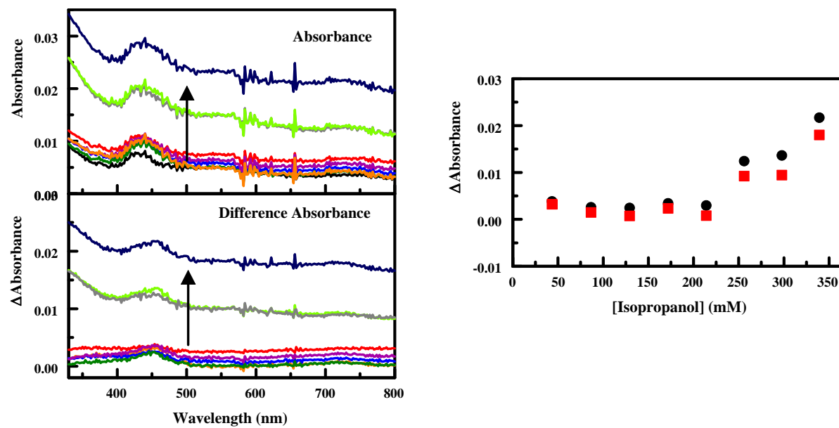
Figure A-20. Absorbance spectra (top) of FeN 4 TPP (9.86 \mu M) in the absence and presence of increasing concentrations of isopropanol: 43, 86, 129, 171, 214, 256, 298, and 339 mM. Arrows indicate increasing target concentration. Absorbance spectra have been corrected for dilution resulting from target addition. Difference absorbance spectra (bottom) are calculated as porphyrin + target minus porphyrin. The concentration dependence of features in the absorbance spectra is also presented (right). Here, the change in absorbance at the peak positions (454 and 730 nm) is plotted against target concentration.
