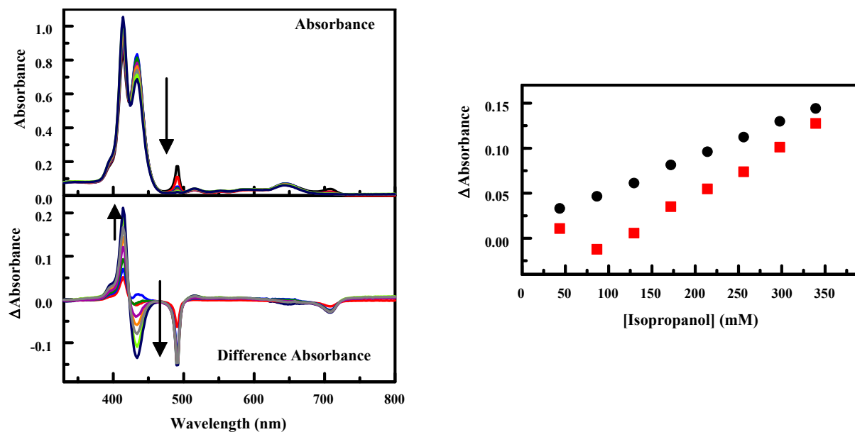
Figure A-2. Absorbance spectra (top) of S 4 TPP (9.86 \mu M) in the absence and presence of increasing concentrations of isopropanol: 43, 86, 129, 171, 214, 256, 298, and 339 mM. Arrows indicate increasing target concentration. Absorbance spectra have been corrected for dilution resulting from target addition. Difference absorbance spectra (bottom) are calculated as porphyrin + target minus porphyrin. The concentration dependence of features in the absorbance spectra is also presented (right). Here, the change in absorbance at the peak and trough positions (418 and 436 nm) is plotted against target concentration.
