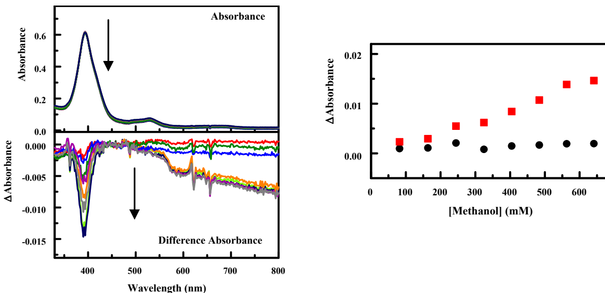
Figure A-21. Absorbance spectra (top) of FeC 4 TPP (9.86 \mu M) in the absence and presence of increasing concentrations of methanol: 82, 163, 244, 325, 404, 483, 563, and 641 mM. Arrows indicate increasing target concentration. Absorbance spectra have been corrected for dilution resulting from target addition. Difference absorbance spectra (bottom) are calculated as porphyrin + target minus porphyrin. The concentration dependence of features in the absorbance spectra is also presented (right). Here, the change in absorbance at the trough and peak positions (340 and 390 nm) is plotted against target concentration.
