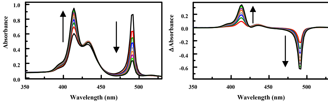
Fig. 3 — Absorbance spectra of AgS 4 TPP (9.86 μM; left) in the absence and presence of increasing concentrations of ethanol: 57, 113, 169, 225, 280, 335, 390, and 444 mM. Arrows indicate increasing target concentration. Absorbance spectra have been corrected for dilution resulting from target addition. Difference absorbance spectra (right) are calculated as porphyrin + target minus porphyrin.
