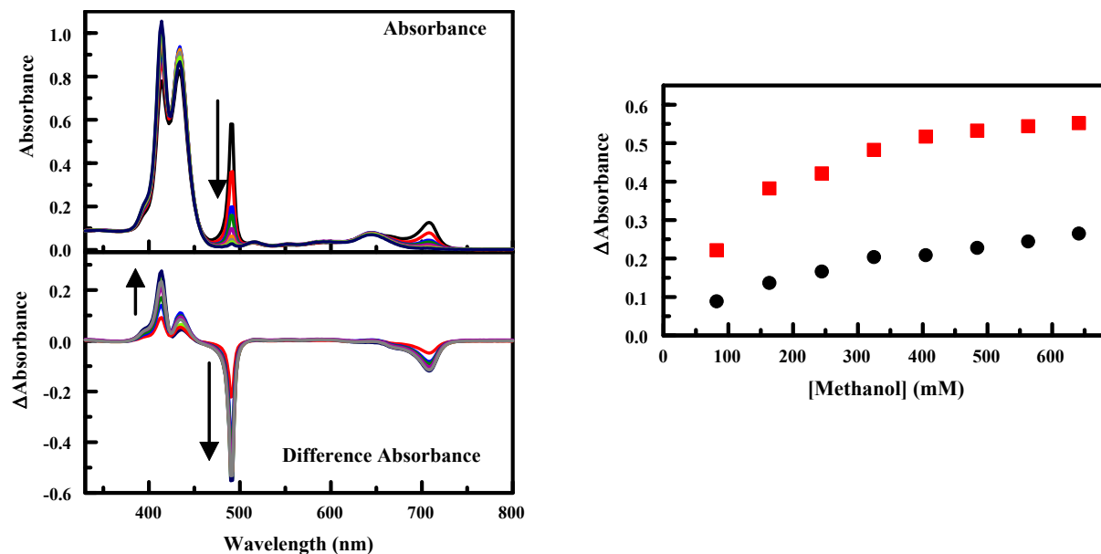
Figure A-3. Absorbance spectra (top) of S 4 TPP (9.86 \mu M) in the absence and presence of increasing concentrations of methanol: 82, 163, 244, 325, 404, 483, 563, and 641 mM. Arrows indicate increasing target concentration. Absorbance spectra have been corrected for dilution resulting from target addition. Difference absorbance spectra (bottom) are calculated as porphyrin + target minus porphyrin. The concentration dependence of features in the absorbance spectra is also presented (right). Here, the change in absorbance at the peak and trough positions (412 and 490 nm) is plotted against target concentration.
