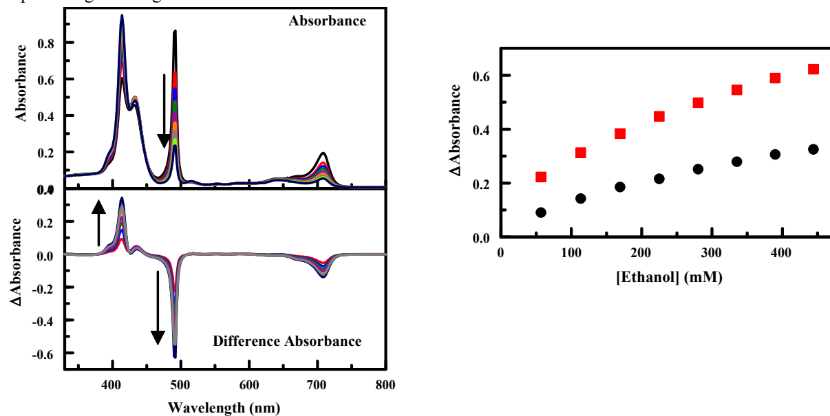
Figure A-4. Absorbance spectra (top) of AgS 4 TPP (9.86 \mu M) in the absence and presence of increasing concentrations of ethanol: 57, 113, 169, 225, 280, 335, 390, and 444 mM. Arrows indicate increasing target concentration. Absorbance spectra have been corrected for dilution resulting from target addition. Difference absorbance spectra (bottom) are calculated as porphyrin + target minus porphyrin. The concentration dependence of features in the absorbance spectra is also presented (right). Here, the change in absorbance at the trough positions (412 and 490 nm) is plotted against target concentration.
