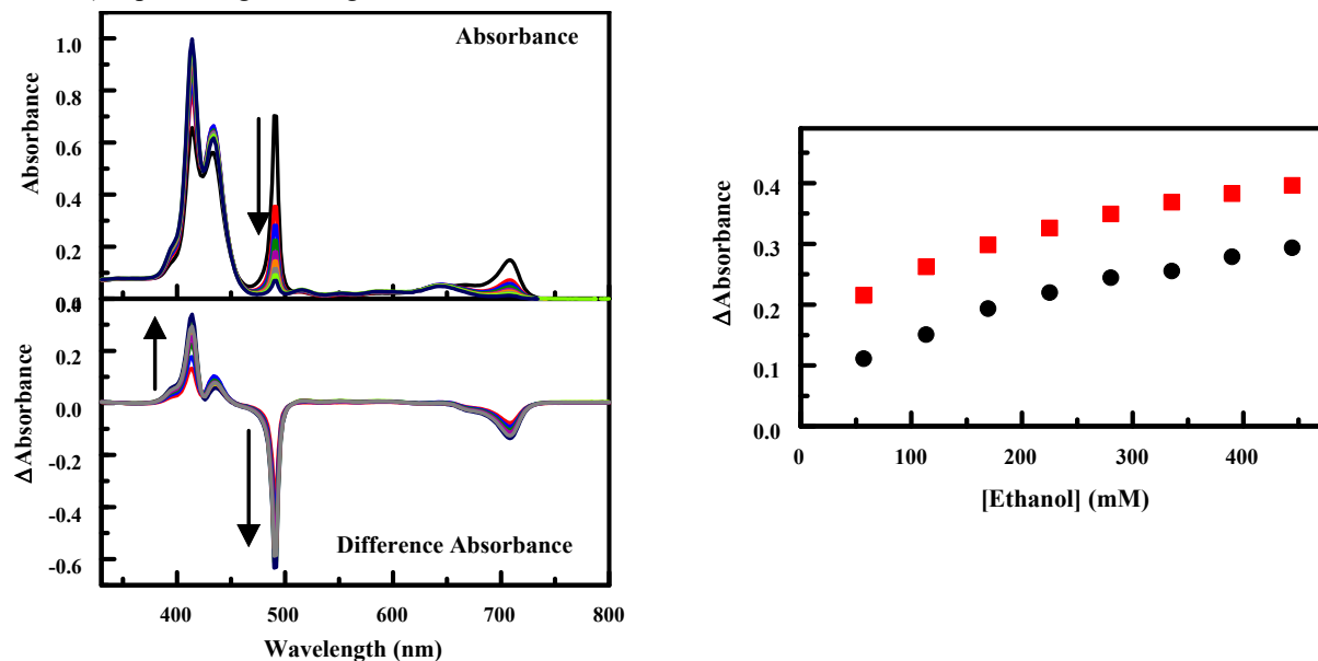
Figure A-1. Absorbance spectra (top) of S 4 TPP (9.86 \mu M) in the absence and presence of increasing concentrations of ethanol: 57, 113, 169, 225, 280, 335, 390, and 444 mM. Arrows indicate increasing target concentration. Absorbance spectra have been corrected for dilution resulting from target addition. Difference absorbance spectra (bottom) are calculated as porphyrin + target minus porphyrin. The concentration dependence of features in the absorbance spectra is also presented (right). Here, the change in absorbance at the peak and trough positions (416 and 488 nm) is plotted against target concentration.
