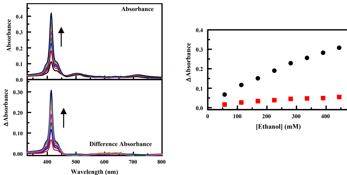
Figure A-10. Absorbance spectra (top) of CeC 4 TPP (9.86 μM) in the absence and presence of increasing concentrations of ethanol: 57, 113, 169, 225, 280, 335, 390, and 444 mM. Arrows indicate increasing target concentration. Absorbance spectra have been corrected for dilution resulting from target addition. Difference absorbance spectra (bottom) are calculated as porphyrin + target minus porphyrin. The concentration dependence of features in the absorbance spectra is also presented (right). Here, the change in absorbance at the trough and peak positions (414 and 432 nm) is plotted against target concentration.
