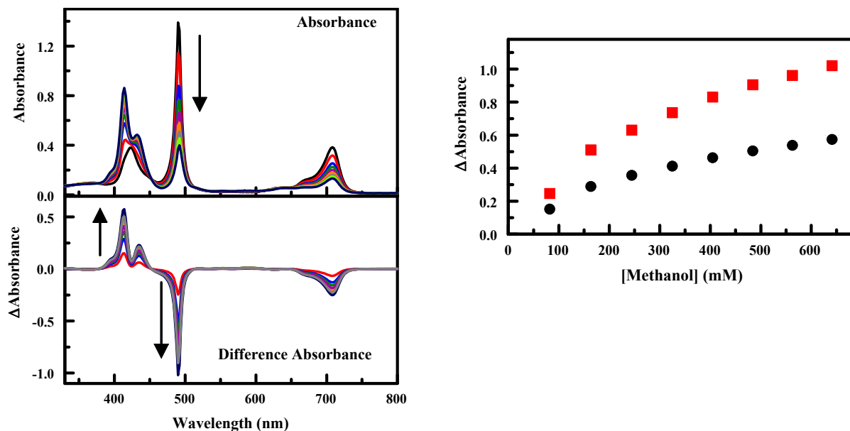
Figure A-9. Absorbance spectra (top) of CdC 4 TPP (9.86 μM) in the absence and presence of increasing concentrations of methanol: 82, 163, 244, 325, 404, 483, 563, and 641 mM. Arrows indicate increasing target concentration. Absorbance spectra have been corrected for dilution resulting from target addition. Difference absorbance spectra (bottom) are calculated as porphyrin + target minus porphyrin. The concentration dependence of features in the absorbance spectra is also presented (right). Here, the change in absorbance at the trough positions (414 and 490 nm) is plotted against target concentration.
