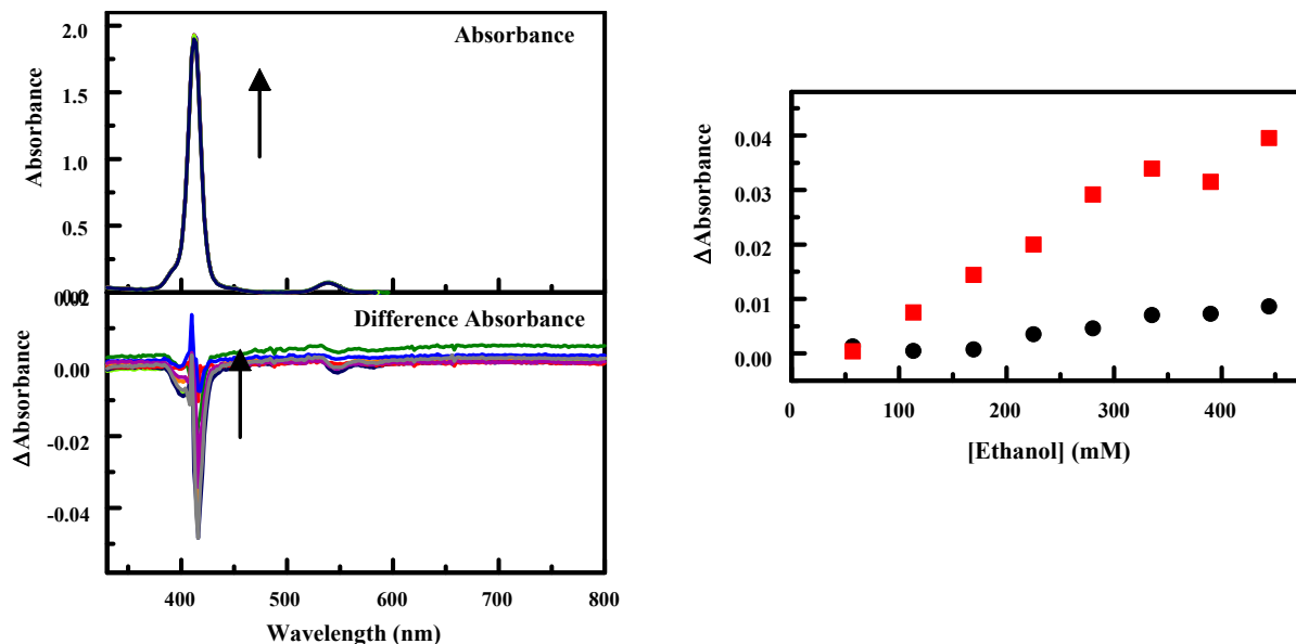
Figure A-16. Absorbance spectra (top) of \text{CuC}_4\text{TPP} ( 9.86 \mu\text{M} ) in the absence and presence of increasing concentrations of ethanol: 57, 113, 169, 225, 280, 335, 390, and 444 mM. Arrows indicate increasing target concentration. Absorbance spectra have been corrected for dilution resulting from target addition. Difference absorbance spectra (bottom) are calculated as porphyrin + target minus porphyrin. The concentration dependence of features in the absorbance spectra is also presented (right). Here, the change in absorbance at the trough positions (400 and 418 nm) is plotted against target concentration.
