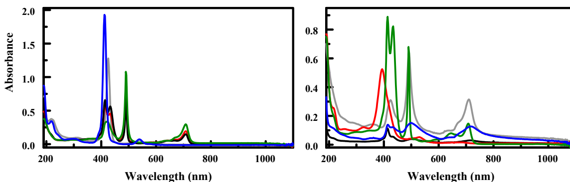
Fig. 2 — Absorbance spectra of the porphyrin and metalloporphyrin variants considered (9.86 \mu M in water): (left) S 4 TPP (black), AgS 4 TPP (red), CdS 4 TPP (green), CuS 4 TPP (blue), CoS 4 TPP (gray); (right) FeS 4 TPP (red), NiS 4 TPP (green), ZnS 4 TPP (gray), CeS 4 TPP (black), YS 4 TPP (blue).
