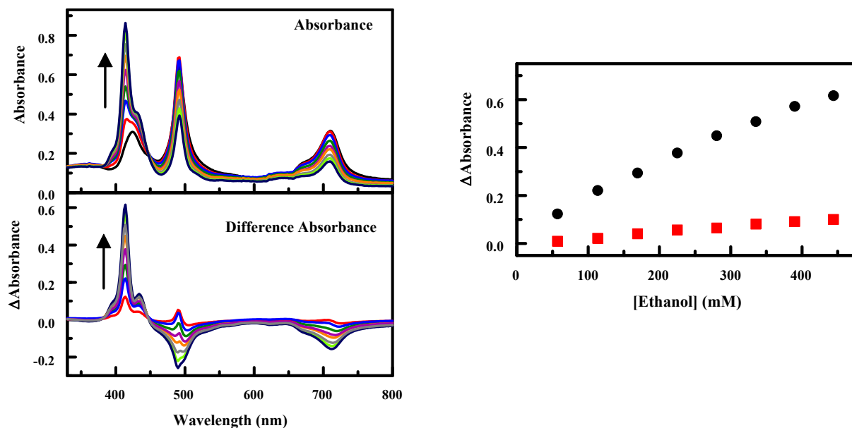
Figure A-28. Absorbance spectra (top) of Zn 4 TPP (9.86 \mu M) in the absence and presence of increasing concentrations of ethanol: 57, 113, 169, 225, 280, 335, 390, and 444 mM. Arrows indicate increasing target concentration. Absorbance spectra have been corrected for dilution resulting from target addition. Difference absorbance spectra (bottom) are calculated as porphyrin + target minus porphyrin. The concentration dependence of features in the absorbance spectra is also presented (right). Here, the change in absorbance at the trough positions (414 and 472 nm) is plotted against target concentration.
