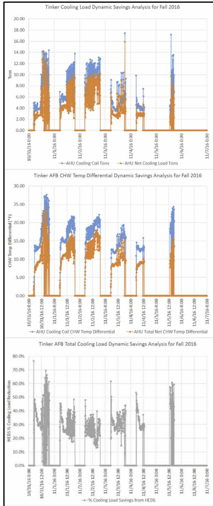
Figure 27. Tinker AFB HEDS Dynamic Savings Analysis for Part Load Days in the Fall.
