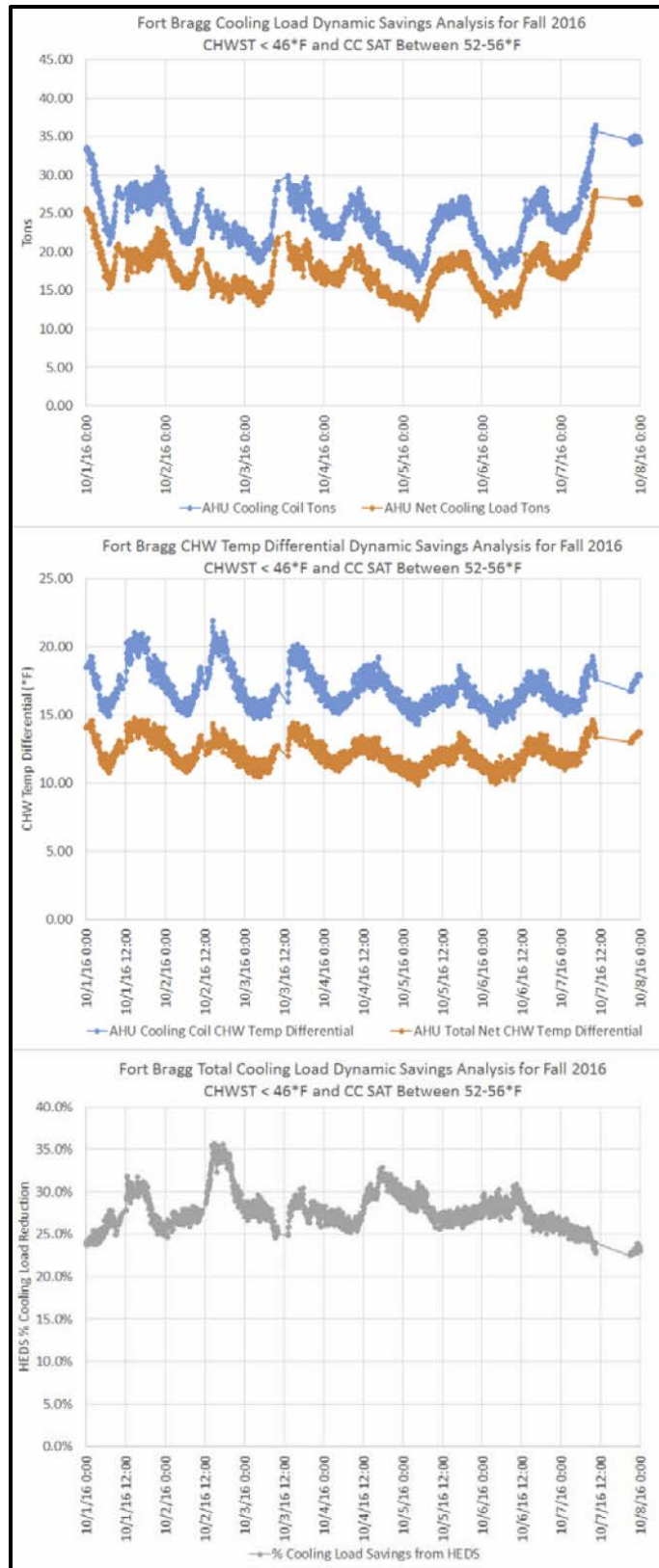
Figure 21. HEDS Savings Analysis for Fall Part Load Days Where the CHWST is less than 46 °F and the CC SAT is between 52 to 56°F.
