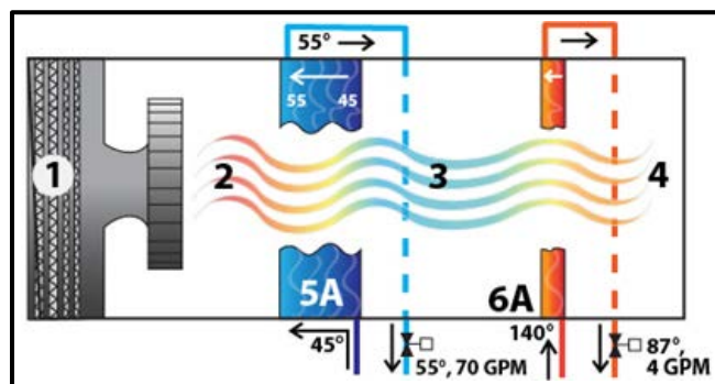
Figure 3. Typical Reheat Dehumidification Design.
