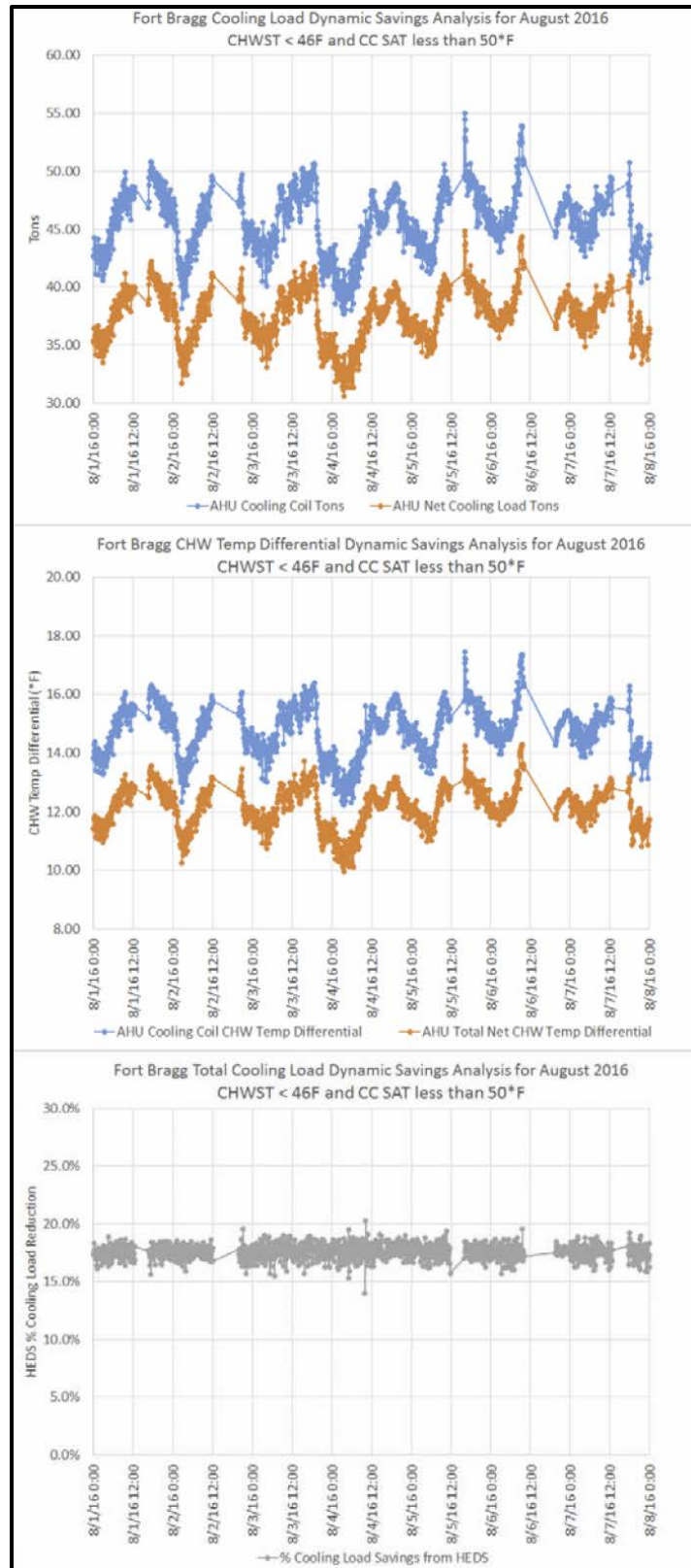
Figure 19. Dynamic HEDS Savings and Impact Analysis for the Peak Cooling Load Week of August 1, 2016.
