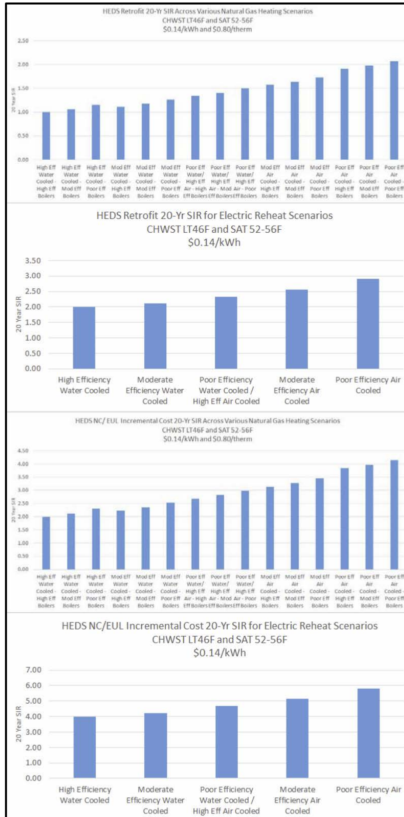
Figure 36. Lifecycle Performance across a Range of Scenarios.
