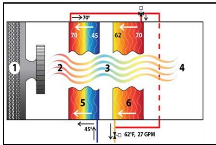
Figure 4. HEDS Unit Depiction Highlighting the Mechanism for Eliminating Reheat and Reducing Cooling Load.
