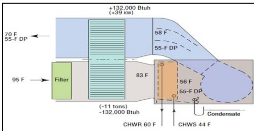
Figure 7. Rotary Heat Exchanger Design Example.
