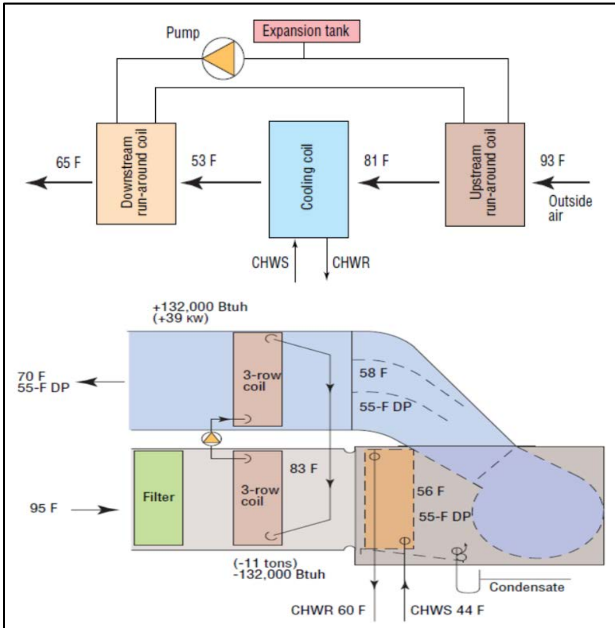
Figure 5. Run-Around Coil System Example Layouts.
