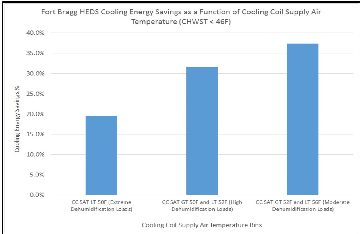
Figure 23. HEDS Cooling Load Reduction as a Function of CC Supply Air Temp (SAT) when Chilled Water Supply Temp is in control (less than 46 °F). Note that the higher SAT ranges have been removed due to the limited hours of operation within the bins.
