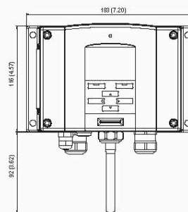
Transmitter with WLAN antenna
