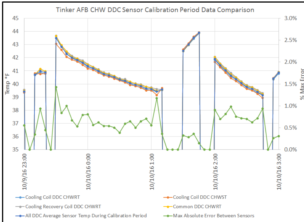
Figure 32. Calibration Period Results Highlighting the Low Error between Sensors for Tinker AFB.
