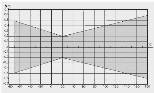
Temperature sensor Pt100 RTD Class F0.1 IEC 60751
