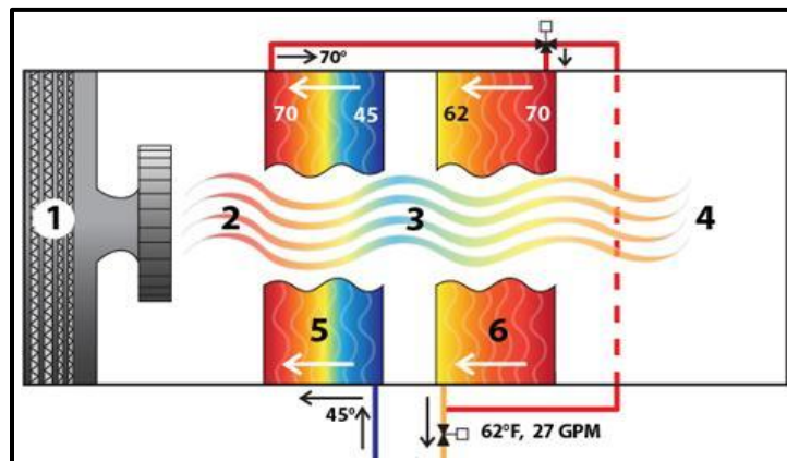
Figure 2. High Efficiency Dehumidification System.
