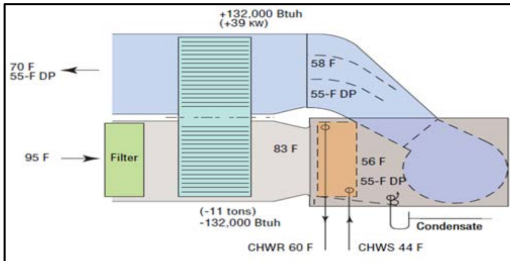
Figure 9. Desiccant Wheel System Placeholder Layout. (Ignore airside temperatures, rough physical layout only intended as a proxy for the Desiccant wheel design)
