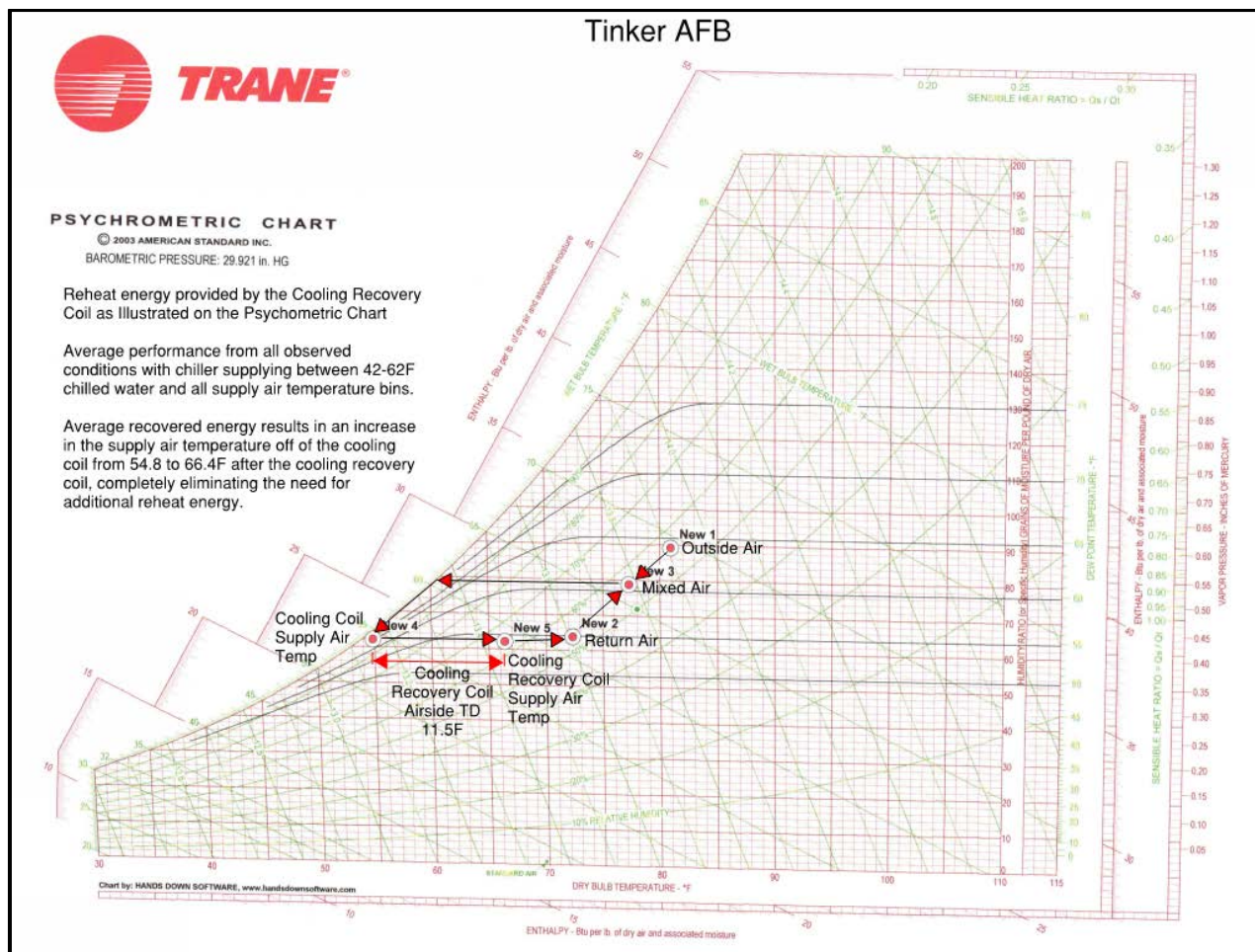
Figure 25. Psychrometric Analysis for Tinker AFB Highlighting the Impact of the Cooling Recovery Coil on HEDS Performance.
