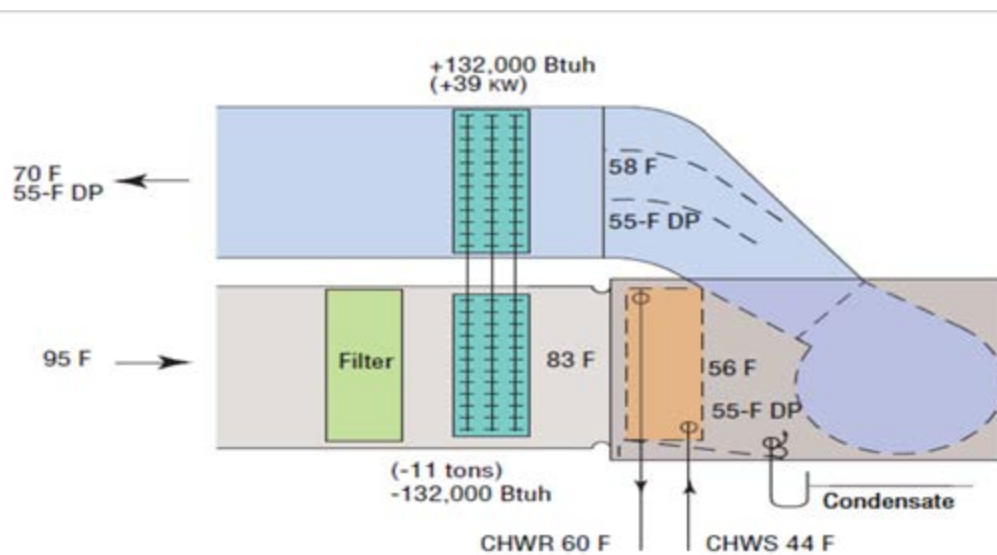
Figure 6. Heat Pipe Coil Design Example.
