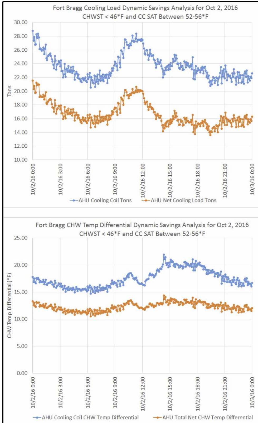
Figure 22. HEDS Savings Analysis for Fall Part Load Peak Day Oct 2, 2016 Where the CHST is less than 46 °F and the CC SAT is between 52 to 56 °F.
