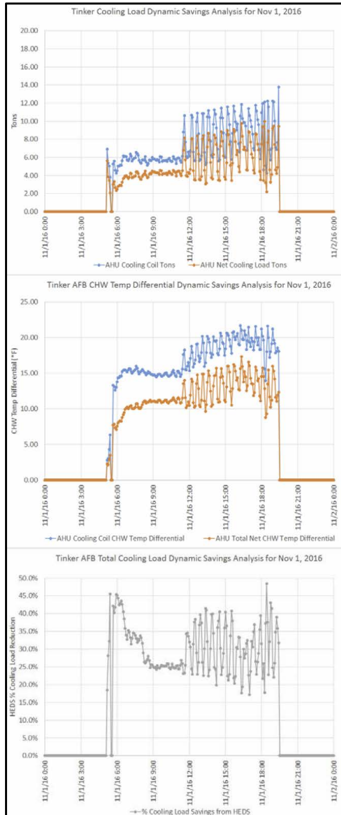
Figure 28. Tinker AFB HEDS Dynamic Savings Analysis for Part Load Day Nov 1, 2016.
