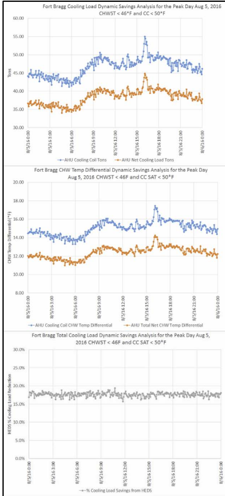
Figure 20. Dynamic HEDS Savings and Impact Analysis for the Peak Cooling Load Day of Aug 5, 2016.
