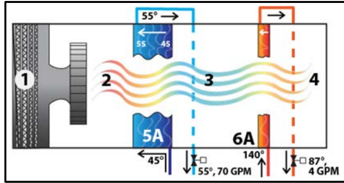
Figure 1. Typical Reheat Dehumidification Design.
