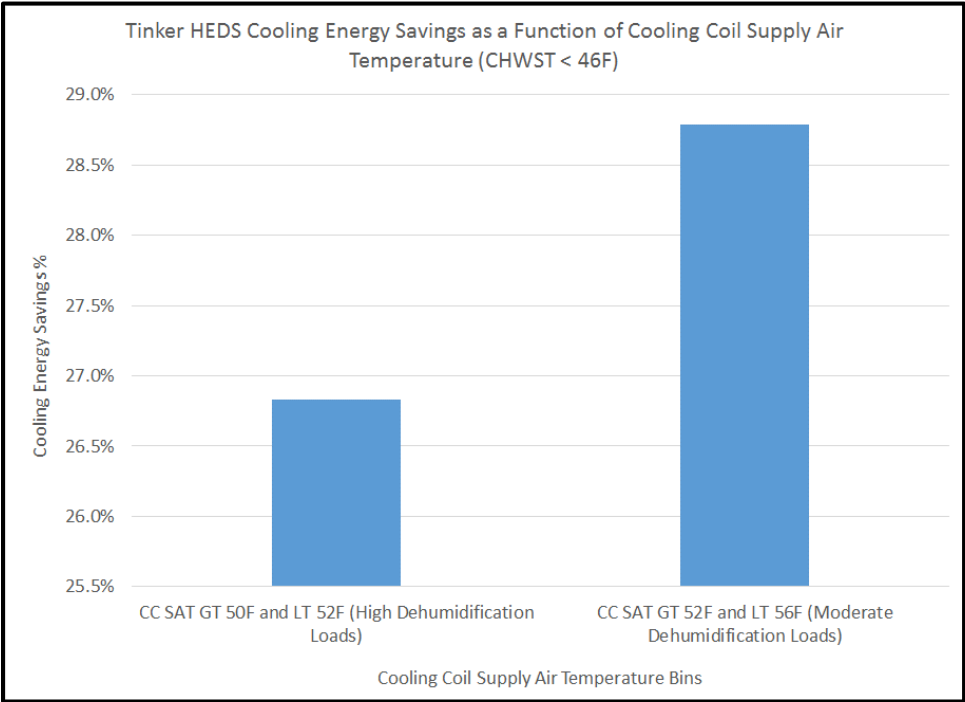
Figure 29. Tinker AFB HEDS Cooling Load Reduction as a Function of CC Supply Air Temp When the Chilled Water Temperature is in Control (less than 46 °F).
