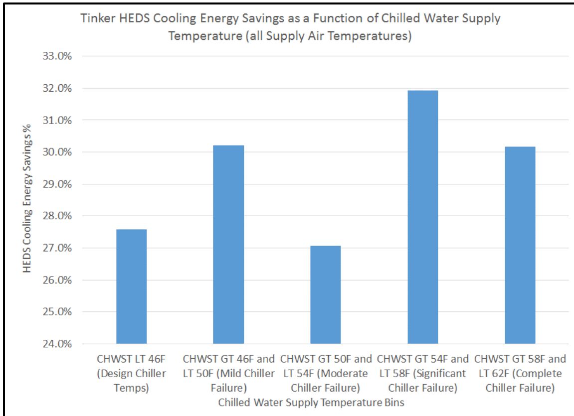
Figure 30. Tinker AFB HEDS Cooling Load Reduction as a Function of Chilled Water Supply Temperature from the Plant.
