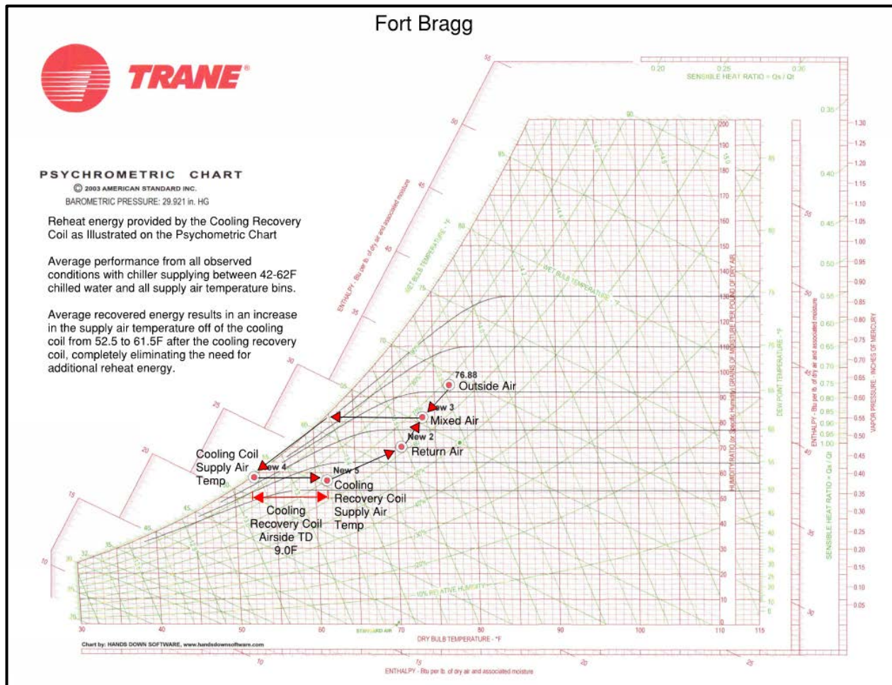
Figure 18. Psychrometric Chart Highlighting the Impact of the Cooling Recovery Coil on HEDS System Performance at Fort Bragg.
