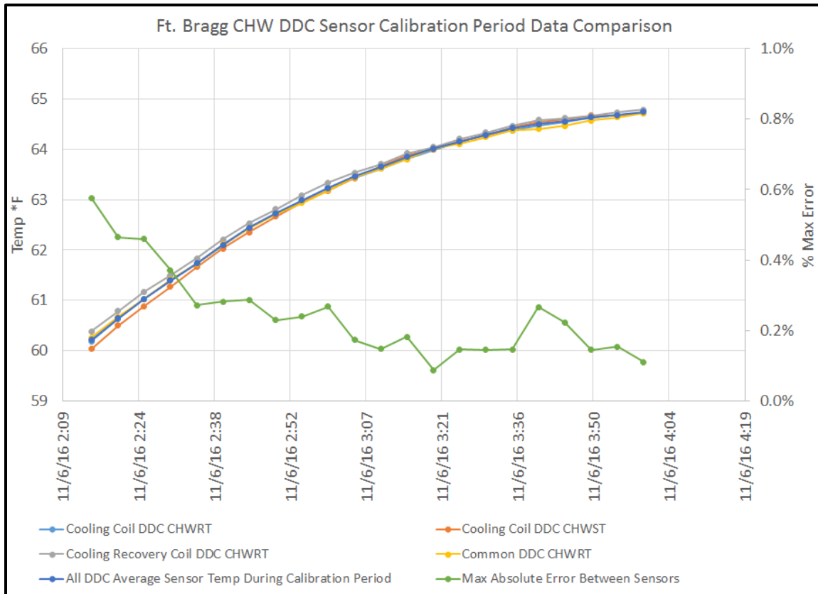
Figure 31. Calibration Period Results Highlighting the Low Error between Sensors for Fort Bragg.
