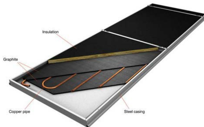
Figure 2-1. Radiant heating/cooling panel for ceiling mount application.
