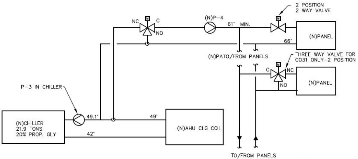
Figure 2-8. Chilled water system schematic.
