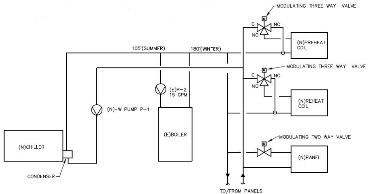
Figure 2-7. Hot water system schematic.
