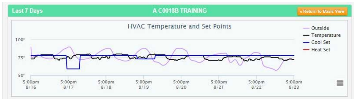
Figure 2-11. Temperature display from Energy Monitoring System for IA Training Rm C0018B for the 7-day period 16-23 Aug 2016.
