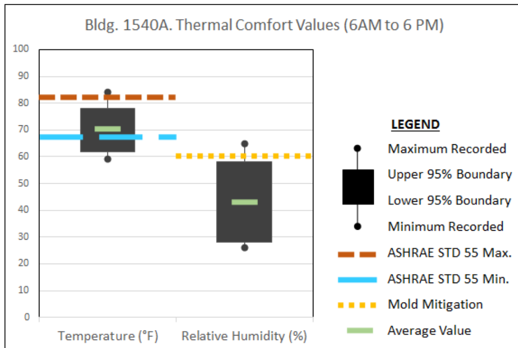
Figure 6-3. Thermal comfort values for Bldg 1540 during occupied hours (6 a.m. to 6 p.m.).
