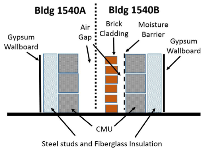
Figure 4-3. Illustration depicting assumed construction details of air gaps separating adjoining walls of Bldgs 1540A and 1540B
