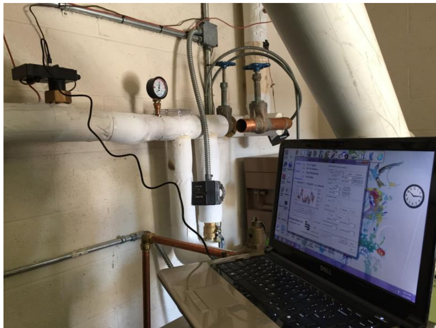
Figure 5-14. Boiler BTU Meter connected to programming software.
