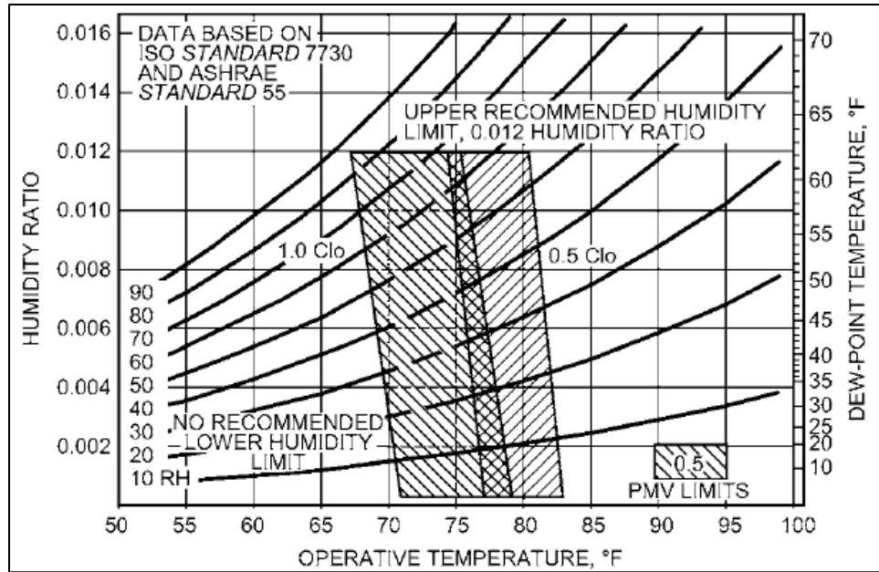
Figure 6-2. A Graphical Zone Method chart derived from ASHRAE Standard 55.
