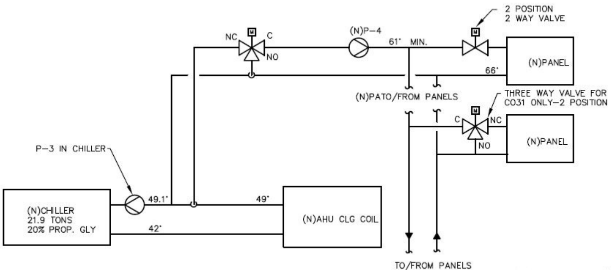
Figure 5-10. Chilled water system schematic.
