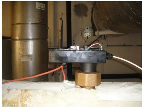
Figure 5-24. BTU Meter located on Bldg 1540B boiler.
