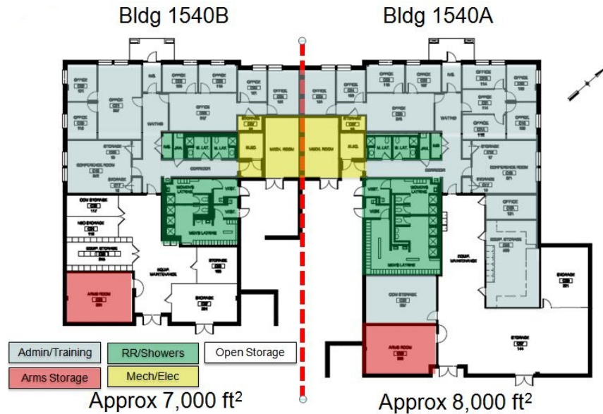
Figure 4-2. Floor plan of Bldg 1540A and Bldg 1540B.
