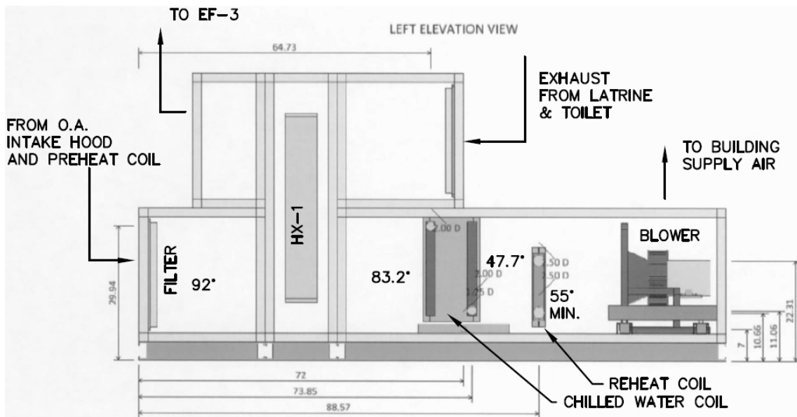
Figure 2-9. DOAS Air Handling Unit.
