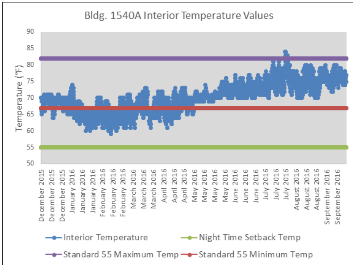
Figure 6-4. Interior temperatures recorded within Bldg 1540A.
