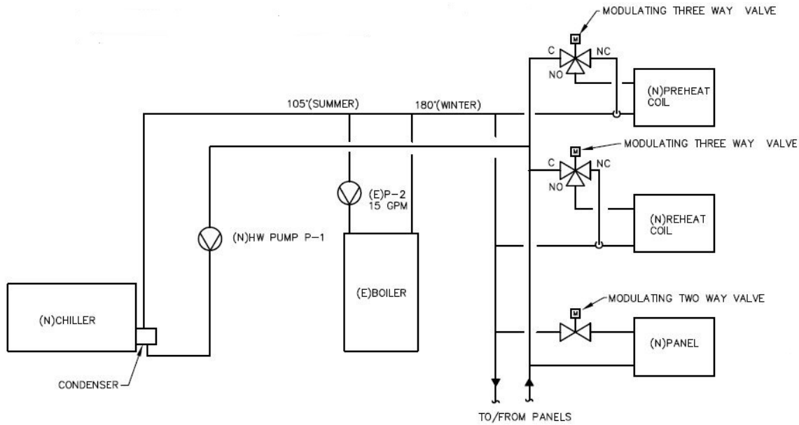
Figure 5-9. Hot water system schematic.
