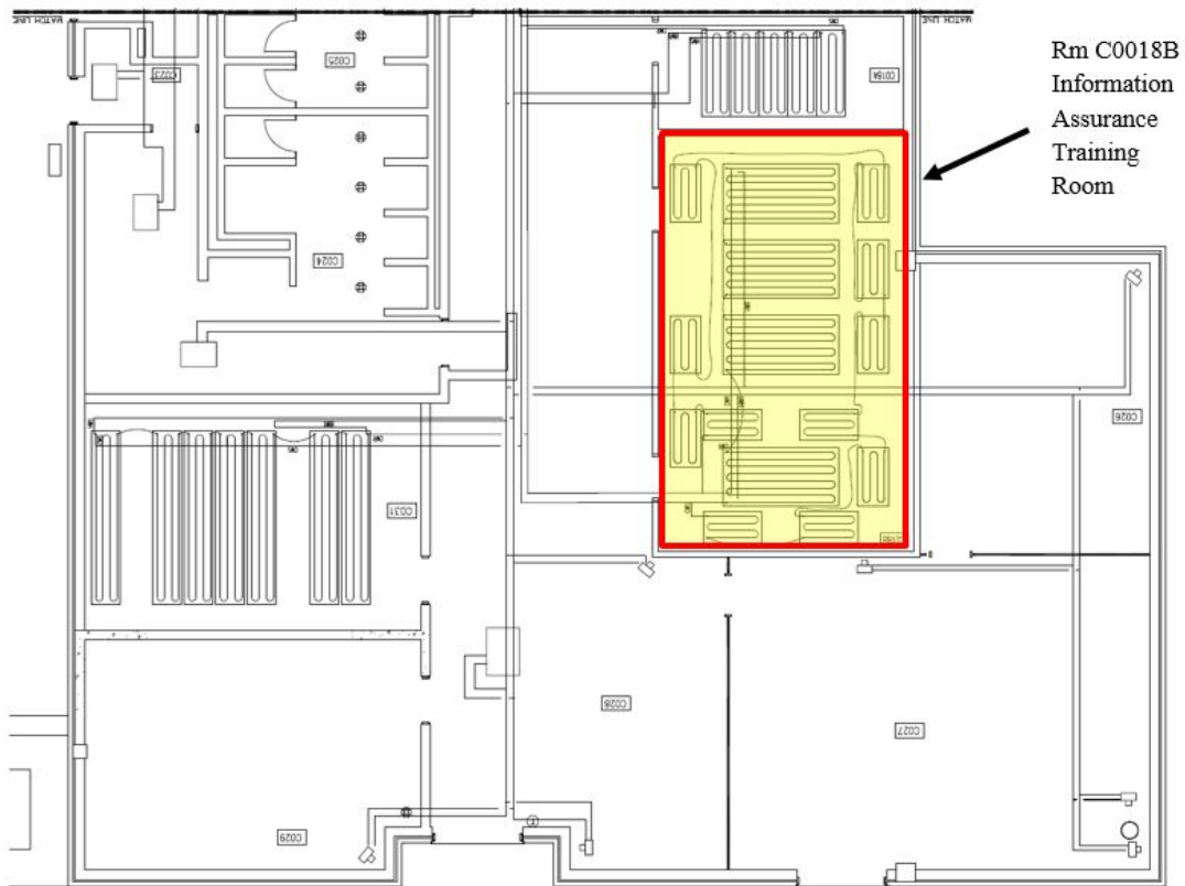
Figure 2-5. Partial plan view (southwest half) of Bldg 1540A showing radiant panels. The 11 smaller panels shown in Room C018B (highlighted) added to address a cooling capacity issue.
