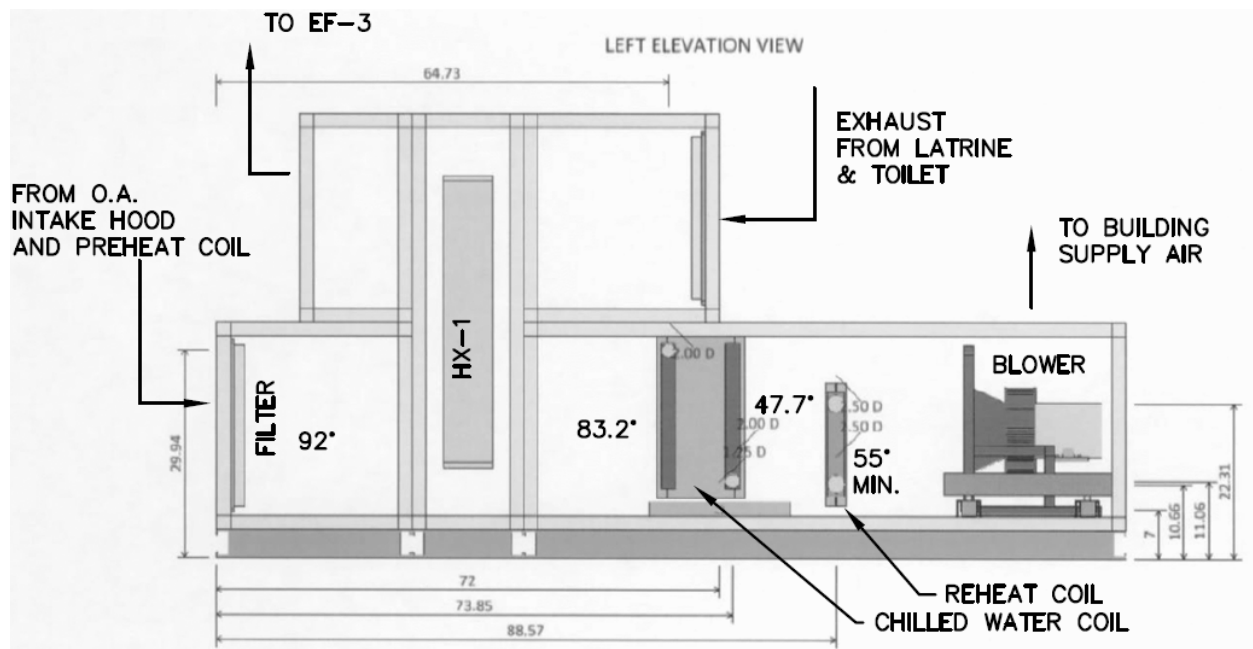
Figure 5-11. DOAS Air Handling Unit.
