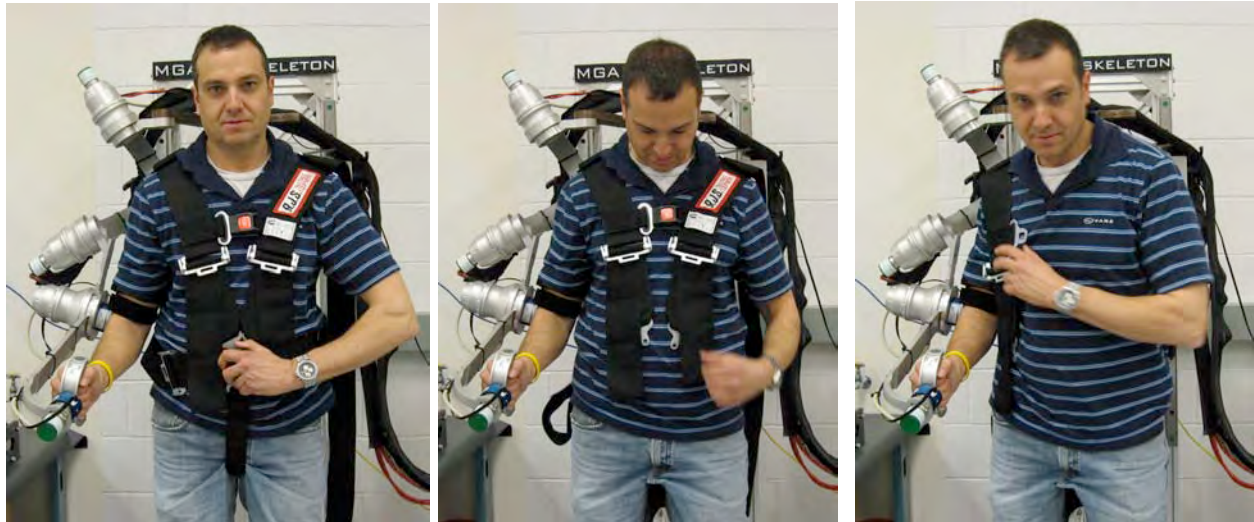
Figure 7: Time series snapshots showing quick release of subject using 5-point harness system.
