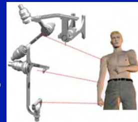
Maryland-Georgetown-Army Exoskeleton (MGAXOS)
