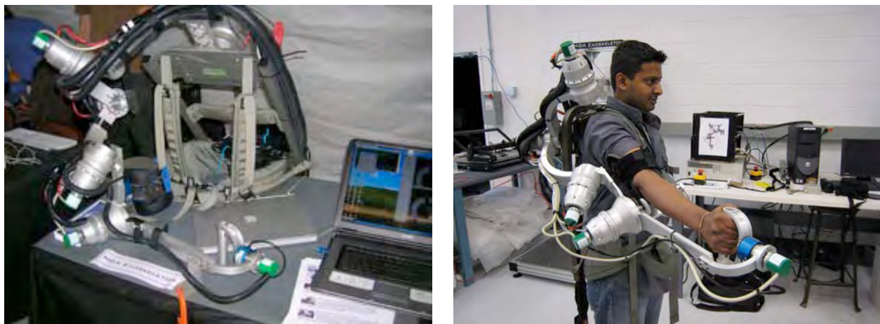
Fig. 15: The MGA Exoskeleton shown on display in the ISIS booth at OASIS Exposition (left) and deployed on subject (right).
