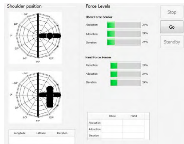
Fig. 13: Telemetry panel prototype for monitoring position and force.
