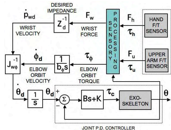
Fig. 11: Admittance (XW) and elbow orbit (EO) control modules used for wall-painting.
