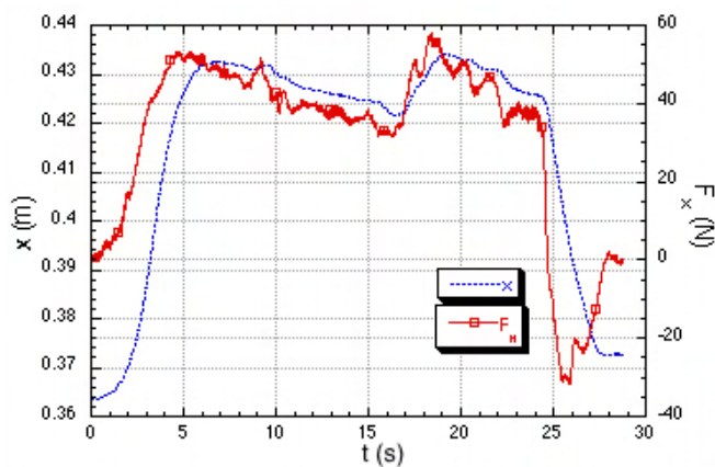
Fig. 11. Handle position and contact force normal to wall.
