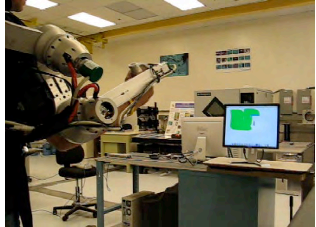
Fig. 9: Exoskeleton handle exerts forces back on subject as roller brush contacts wall.
