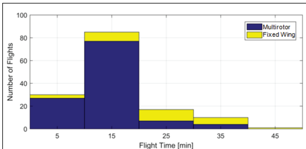
Figure 4-4. Histogram of individual flight durations. Bins are centered on tick marks and 10 min wide. Birdseye View is considered a fixed-wing platform in this analysis.
