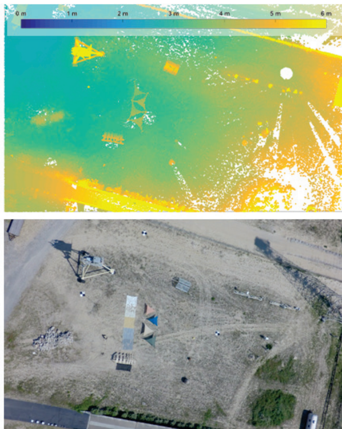
Figure 3-7. Example point cloud in plan view (top) and near nadir UAS image (bottom) of target pad area. Point cloud scans performed 26 June 2017. NAVD88 1 elevation plotted in point cloud; color is saturated with a maximum of 6 m to highlight low-elevation targets. Imagery from CHL X8+.
