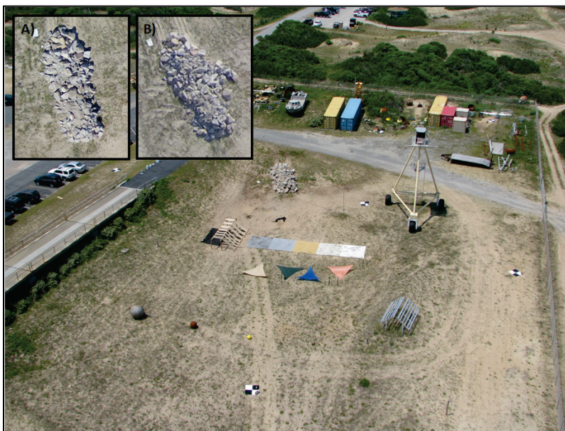
Figure 3-6. Image of target pad area and UAS evaluation targets. Camera position is east of the target pad, oriented west. Inset: Image of (A) intact and (B) destroyed mock jetty.
