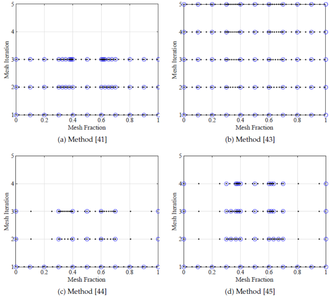
Figure 18. Mesh refinement history for each method. Note that the blue circles and black dots represent mesh points and collocation points, respectively.
