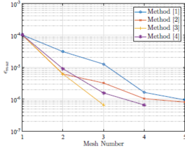
Figure 59. Mesh maximum relative error for each mesh.
