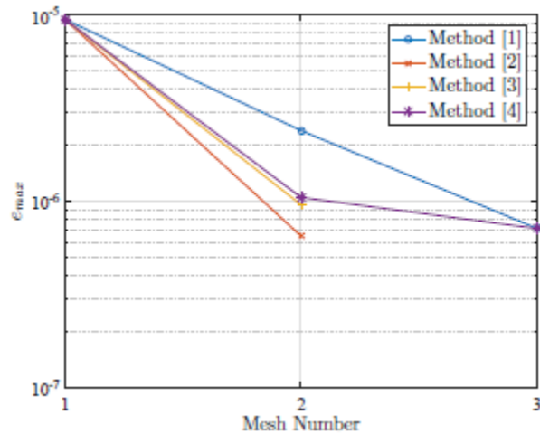
Figure 55. Mesh maximum relative error for each mesh.
