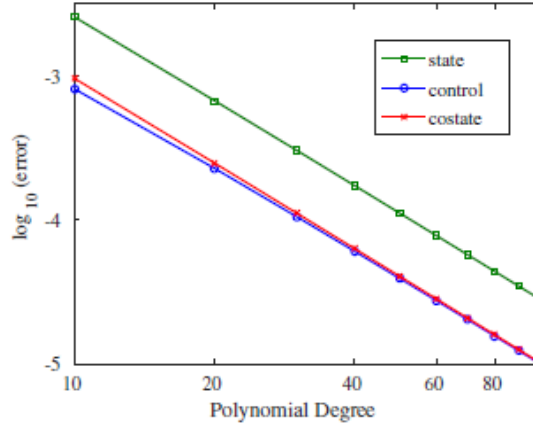
Figure 74. Logarithm of sup-norm error in state, control, and costate versus polynomial degree.
