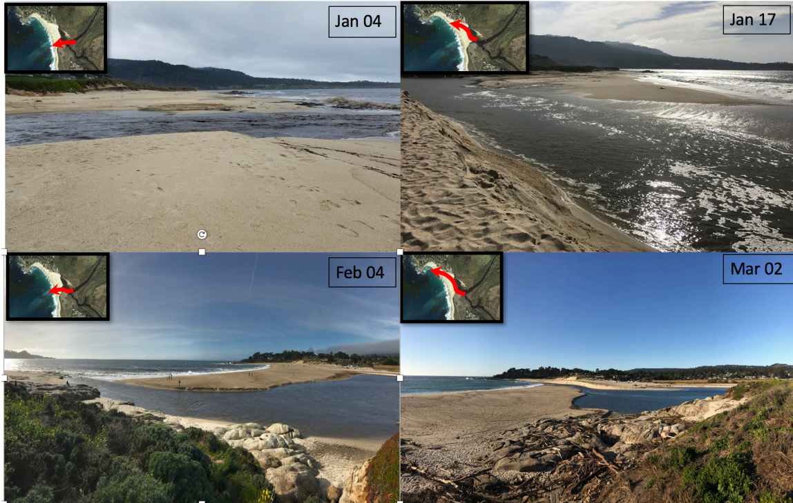
Figure 19. Photos showing the different locations of the channel after the river remained open.
