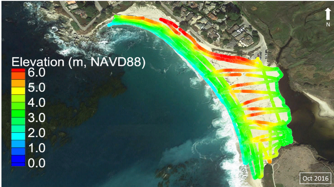
GPS survey showing berm height. Red colors running down the middle of the beach from north to south is the peak of the berm, which averaged 6 m. Near the southern end (bottom of map) there is a depression measuring 4.3 m, which is the location of the initial breach.
