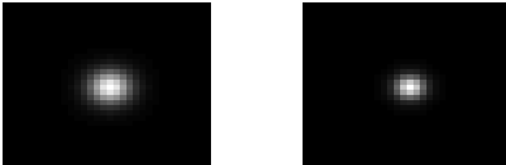
Figure 38. Point spread functions used to generate simulated data and conduct spatial correlation testing. Scenario 1: PSF with r_0 = 5 cm (left side). Scenario 2: PSF with r_0 = 8 cm (right side).
