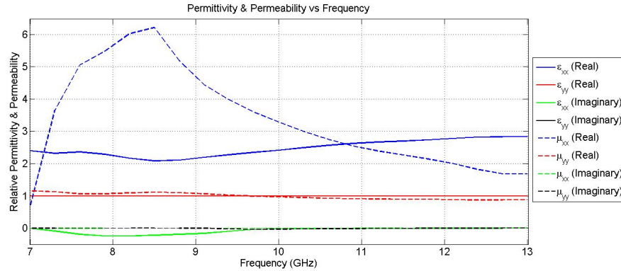
Figure 61. Permittivity and Permeability Results for the 2 by 48 wired media.
