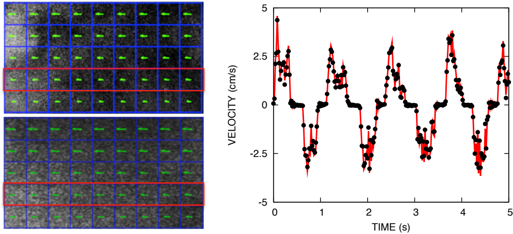
Figure 6 – Left: Part of the flow field of a sheared gelatin sample imaged by a camera (top) and the same sample imaged by the ultrasound (bottom). Right: Velocity averaged over a horizontal line (labeled with red boxes on the left) at a single vertical position as a function of time, measured by the camera (red line) and the ultrasound (black points).
