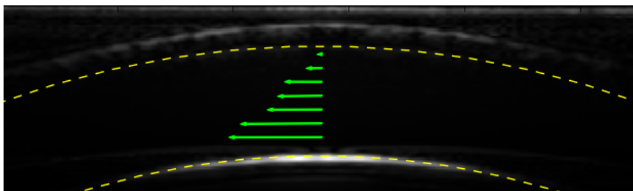
Figure 10 – Ultrasound image of the Couette-geometry, with the measured velocity profile (green arrows). The yellow dashed lines indicate the cylinder walls.
