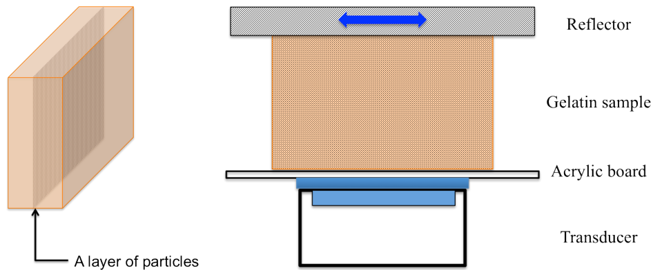
Figure 5 – Left: A schematic illustration of the gelatin sample embedded with a layer of scattering particles. Right: A schematic illustration of the experimental setup. The blue double sided arrow in the reflector means that the reflector was moved horizontally to shear the sample.
