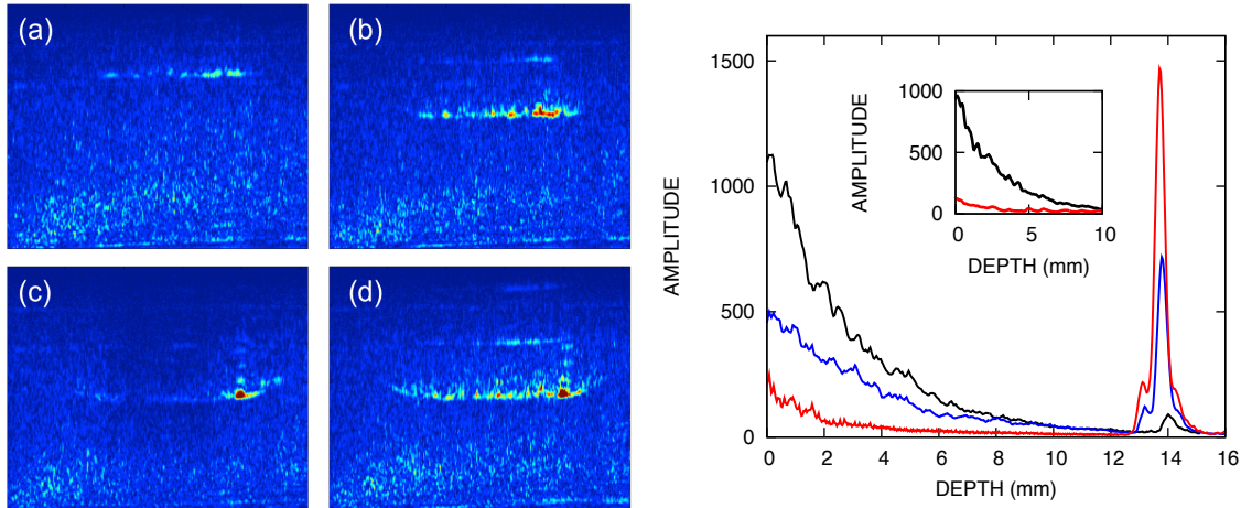
Figure 8 – Left: Change of brightness of the reflected signal in cornstarch suspension when compressed. Right: The amplitude of reflected signals in cornstarch suspension at different applied stress: black- 1P_0 , blue- 4P_0 and red- 7P_0 , where P_0 is a stress level corresponding to atmospheric pressure (1 bar). Inset: The amplitude of reflected signals in degassed (red) and non-degassed (black) cornstarch suspensions.
