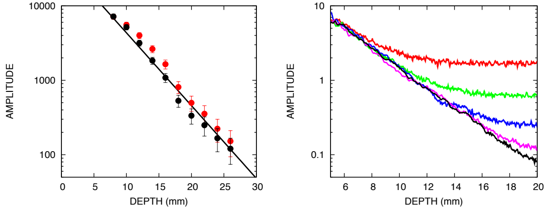
Figure 4 – Left: Attenuation of the reflected signal in 45% degassed cornstarch suspension before (red) and after (black) the amplitude correction. Right: Amplitude of signals in 40% non-degassed cornstarch suspension at different amplifications. Color indicates TGC: red-100, green-300, blue-500, pink-700 and black-900. The amplitudes were normalized by TGC = 1.
