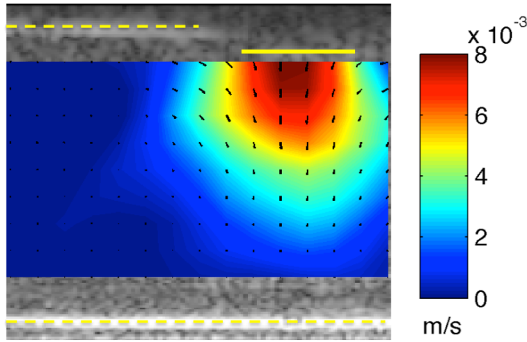
Figure 9 – Flow field in a density matched cornstarch suspension under vertical impact. The color code represents the magnitude of the vertical velocity. The two horizontal dashed yellow lines denote the fluid surface and the bottom of the container, respectively. The solid yellow bar indicates the position of the pusher (reflector).
