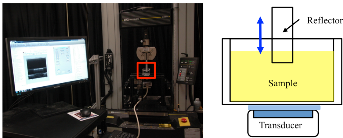
Figure 1 – Left: Photo of the setup, showing part of the ultrasound system and how it is combined with the Instron material tester. Right: Schematic view of the setup in the red box where the reflector is attached to the Instron.
