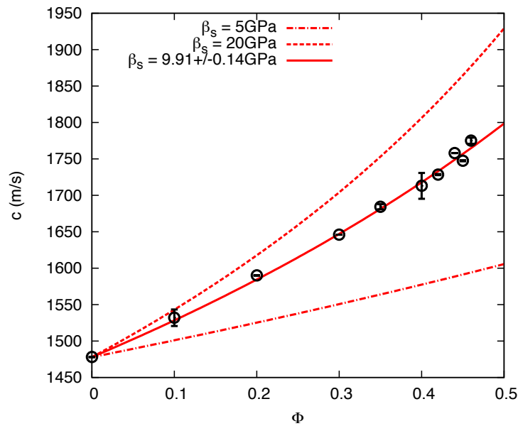
Figure 7 – Speed of sound c in density matched cornstarch suspensions at different packing fractions \Phi . The solid red line is a fitting of the data with Equation XX and the dashed red lines are predictions of the trend at two other particle moduli \beta_s .
