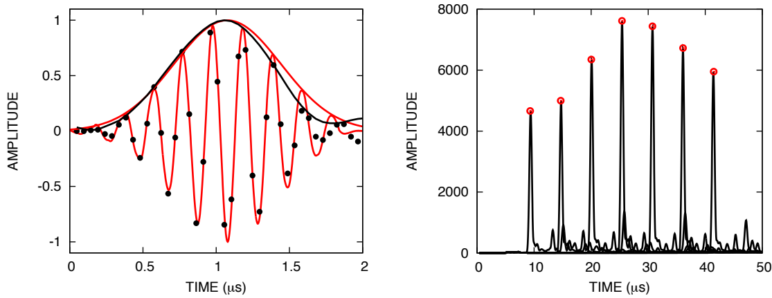
Figure 3 – Left: Comparison between the transmitted signal from the ultrasound transducer (red) and the received signal (black). Right: Envelopes of the received signals reflected from different distances (equally separated from 4mm to 28mm). The red circles label the peak of each envelope.
