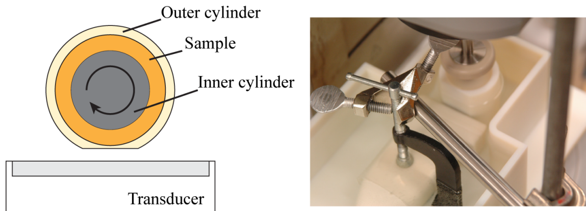
Figure 2 – Left: Schematic view of the setup where we combine ultrasound imaging with rheometry. Right: Photo of the setup, showing part of the outer container in which the transducer is submerged.
