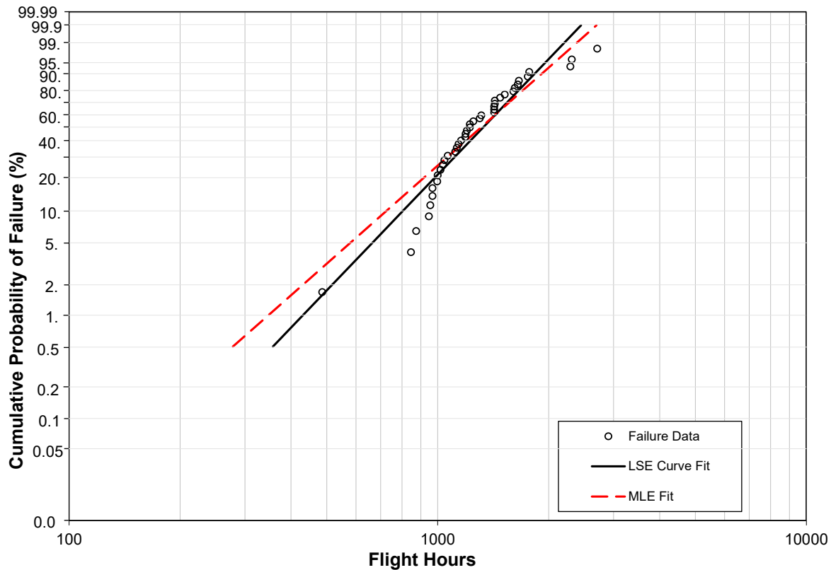
Figure 15. Updated Lifetime Distribution from Additional Cracking Data
