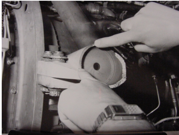
Figure 23. Failed fitting attached to the engine indicating length of fatigue crack.
