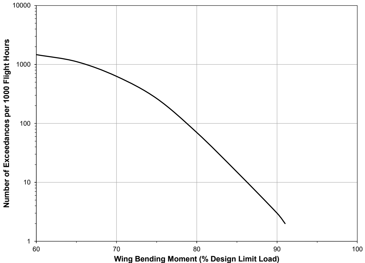
Figure 30. Wing Bending Moment Exceedances per 1000 Hours
