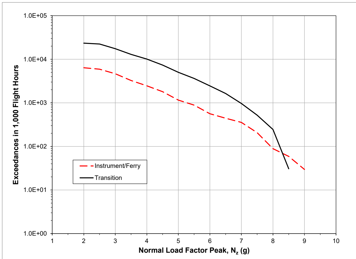
Figure 40. Peak N_z Exceedances for Transition and Instrument/Ferry Flights
