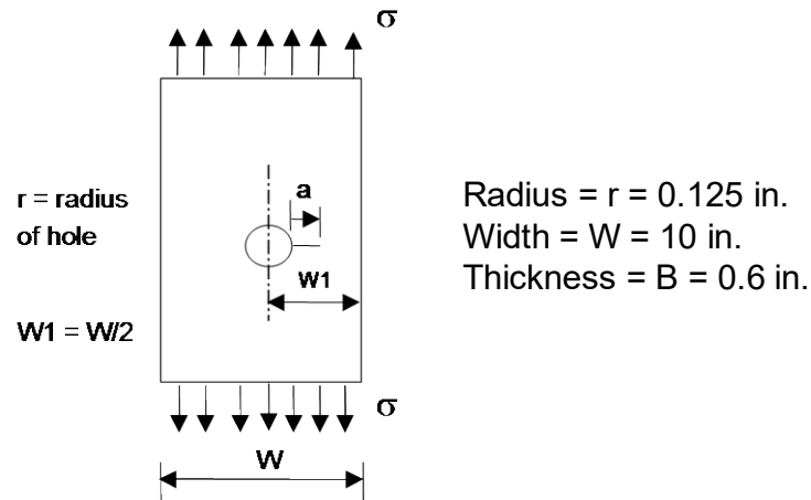
Figure 48. Geometry for Fracture Reliability Example (Repeated) Plate loaded in uniform tension with a through-thickness, radial cracked hole
