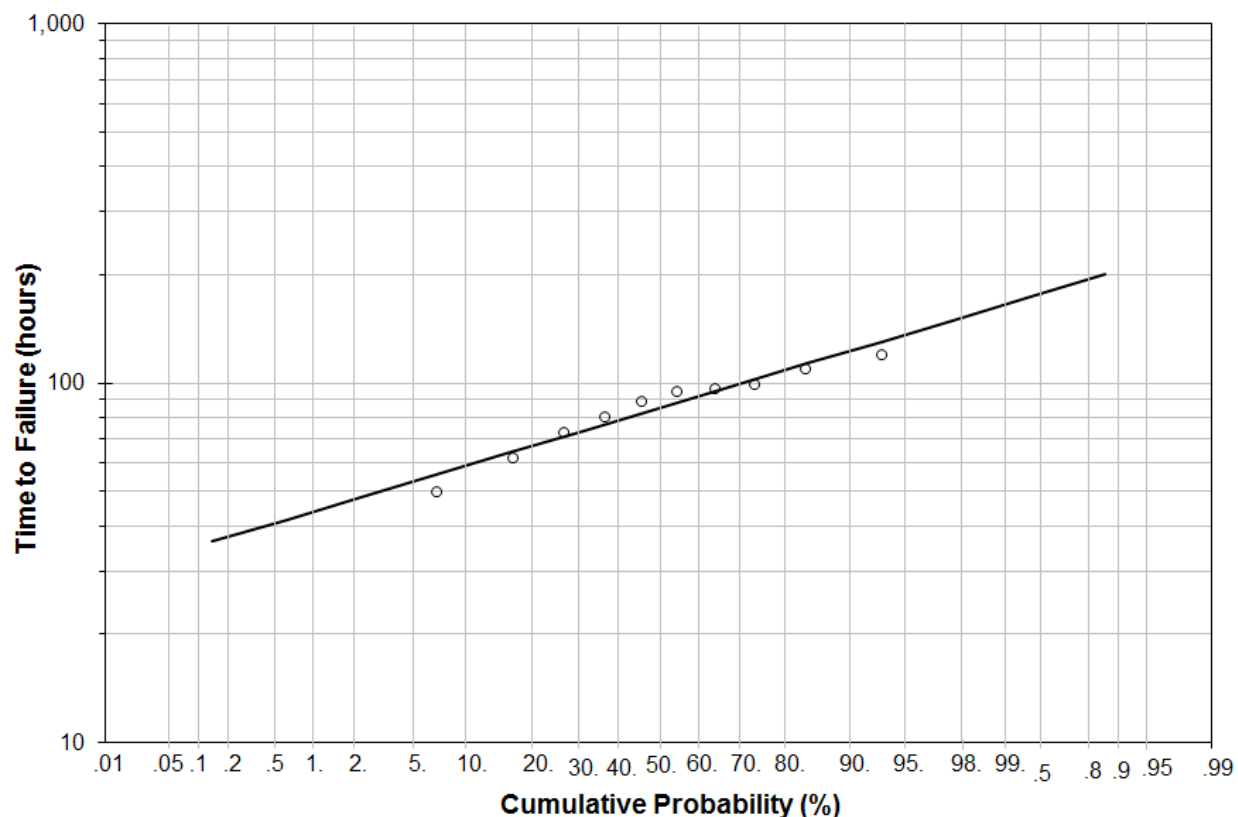
Figure 9. Lognormal Probability Plot of Failure Data
