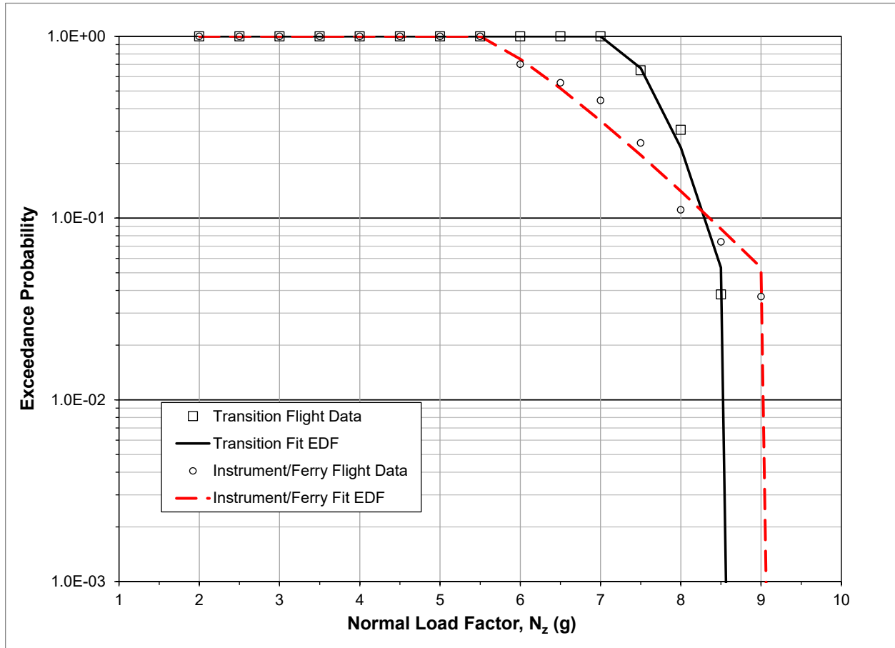
Figure 42. N_z EDFs for Transition and Instrument/Ferry Flights
