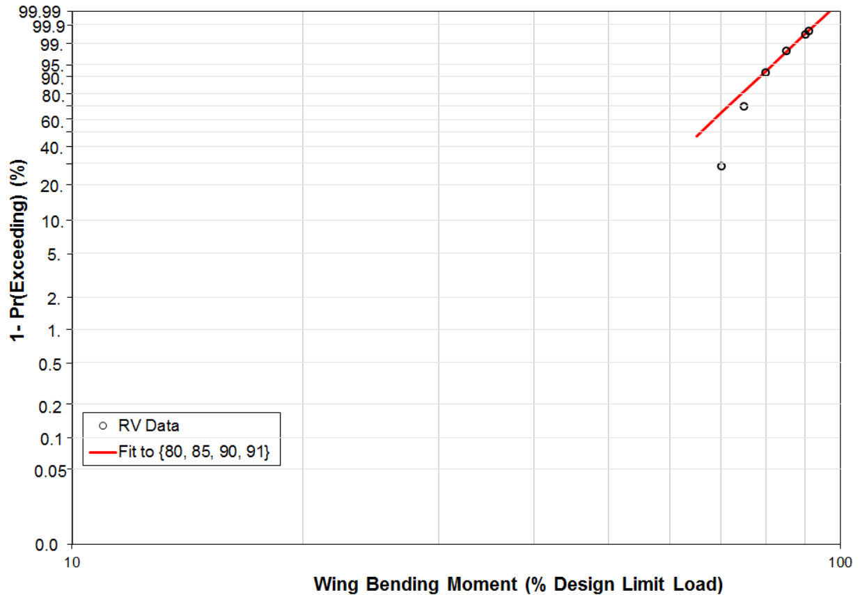
Figure 32. Weibull Extrapolation of WBM EDF
