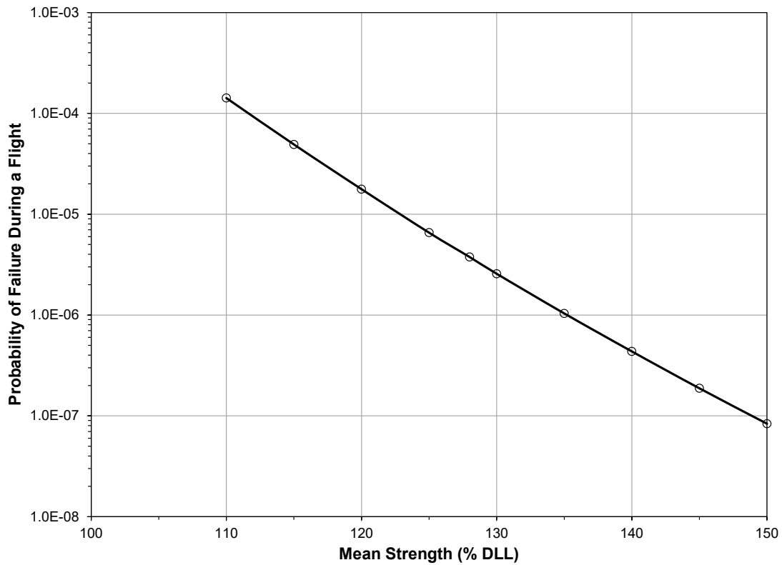
Figure 35. POF as a Function of Mean Strength with a Shape Parameter of 24
