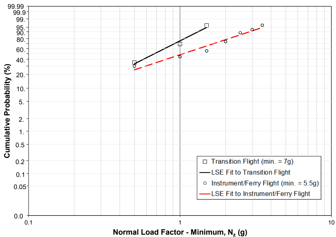
Figure 41. Weibull Extrapolation of N_z EDF for Transition and Instrument/Ferry Flights
