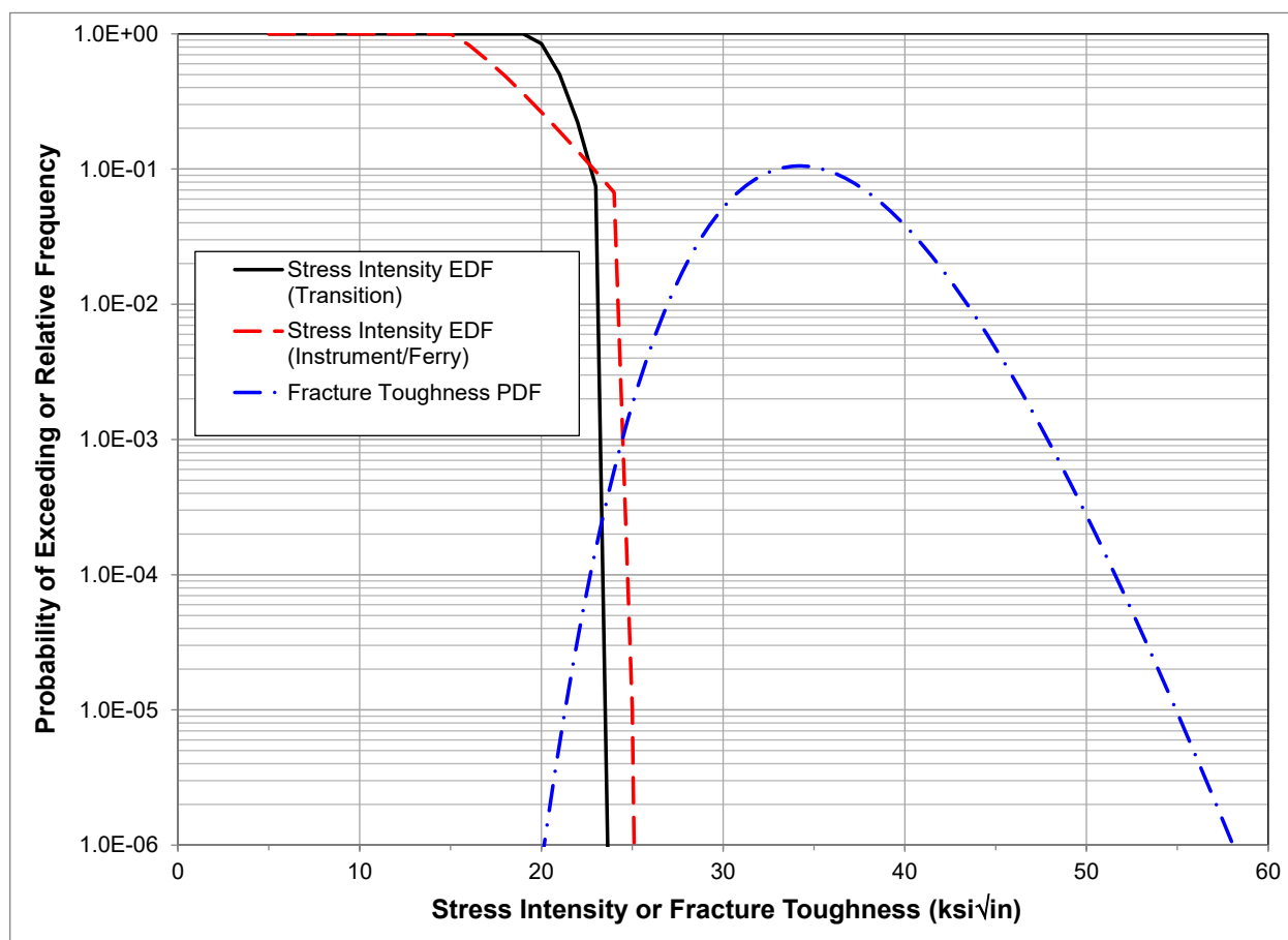
Figure 43. Plot of Applied Stress Intensity EDFs and Fracture Toughness PDF
