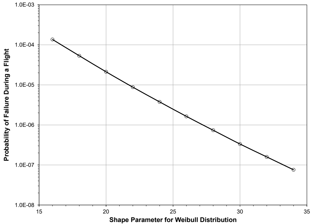
Figure 36. POF as a Function of the Shape Parameter with a Mean Strength of 128 Percent DLL
