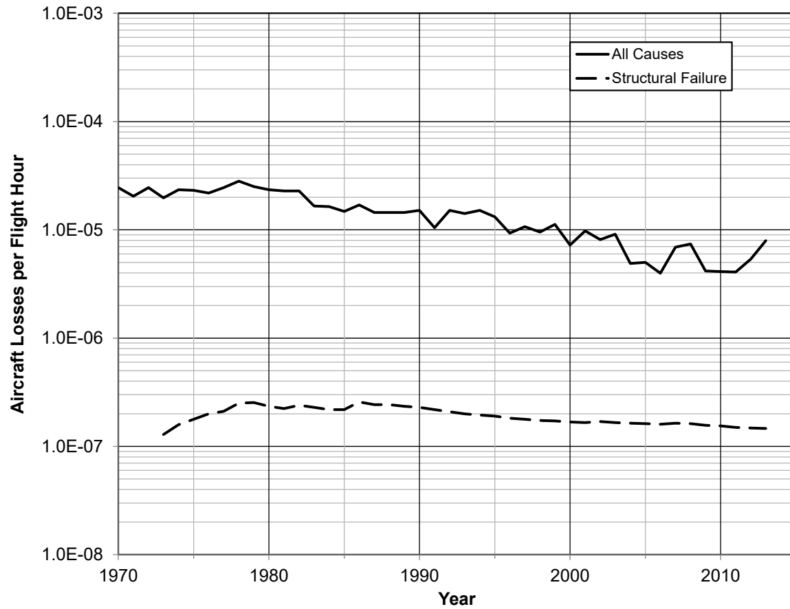
Figure 1. USAF Aircraft Loss Rate Comparing losses from all causes to those from structural failures as the primary cause [9]
