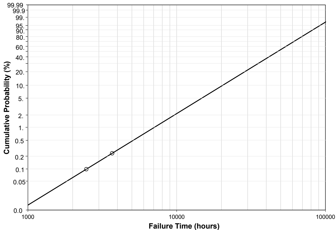
Figure 26. Weibull Probability Plot of the Two Thrust Fitting Failures.
