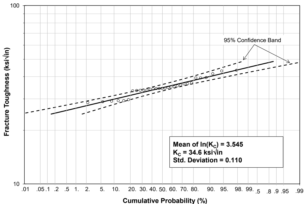
Figure 39. Lognormal Probability Plot of Fracture Toughness for Al 7050-T7351 Plate
