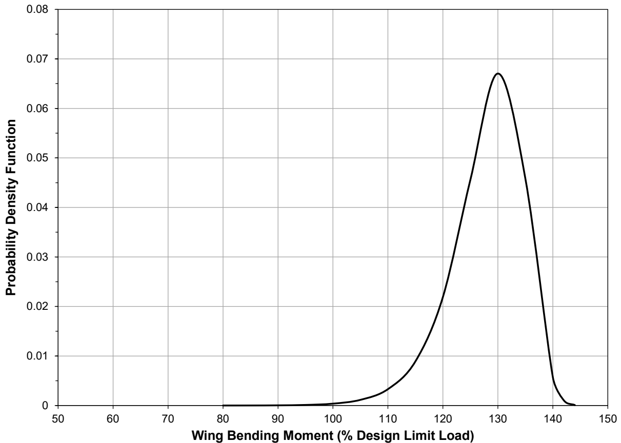
Figure 29. Weibull PDF for Wing Strength
