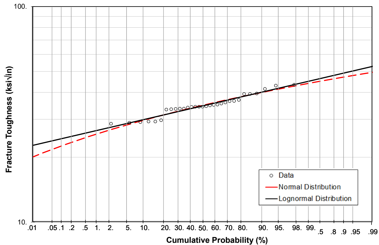
Figure 45. Normal and Lognormal Distributions for Al 7050-T7351 Plate Fracture Toughness Data
