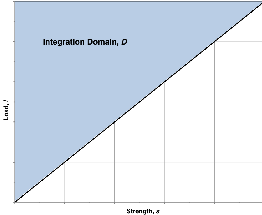
Figure 27. Integration Domain for Reliability Integral
