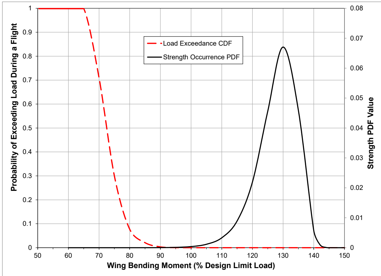
Figure 34. Plot of Load EDF and Wing Strength PDF
