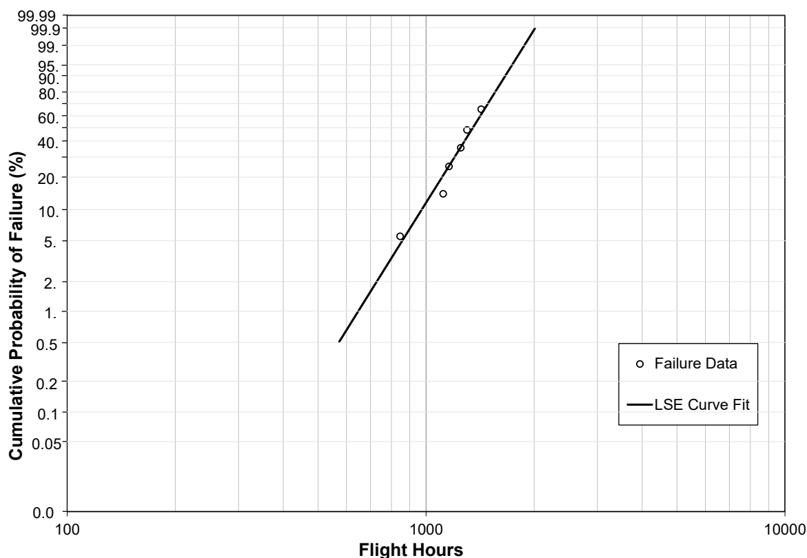
Figure 14. Weibull Probability Plot of Initial Cracking Data
