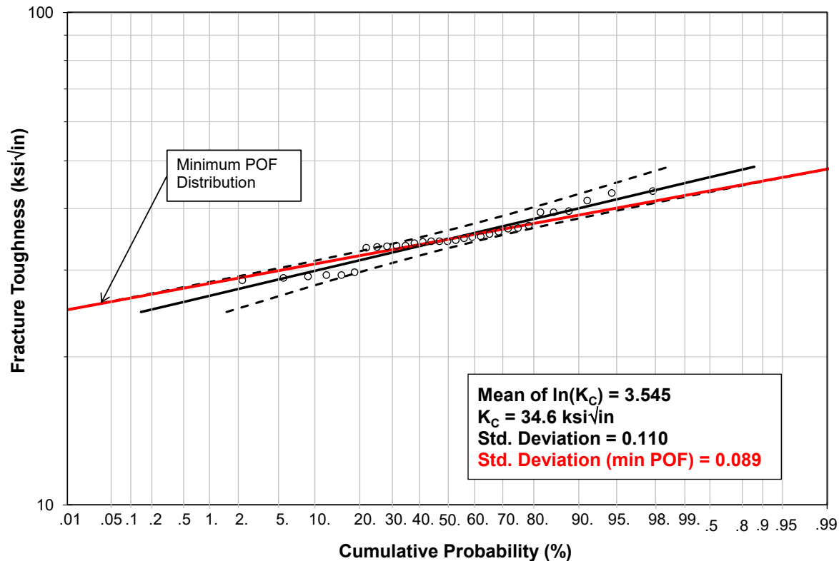
Figure 44. Minimum POF Fracture Toughness Distribution within 95 Percent Confidence Band
