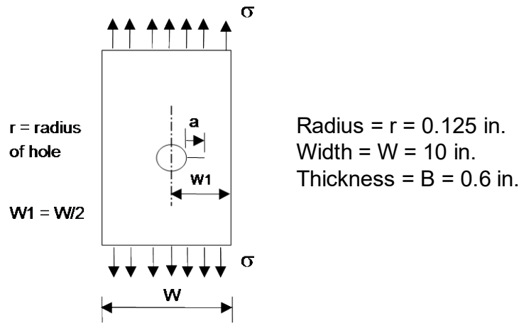
Figure 38. Geometry for Fracture Reliability Example Plate loaded in uniform tension with a through-thickness, radial cracked hole
