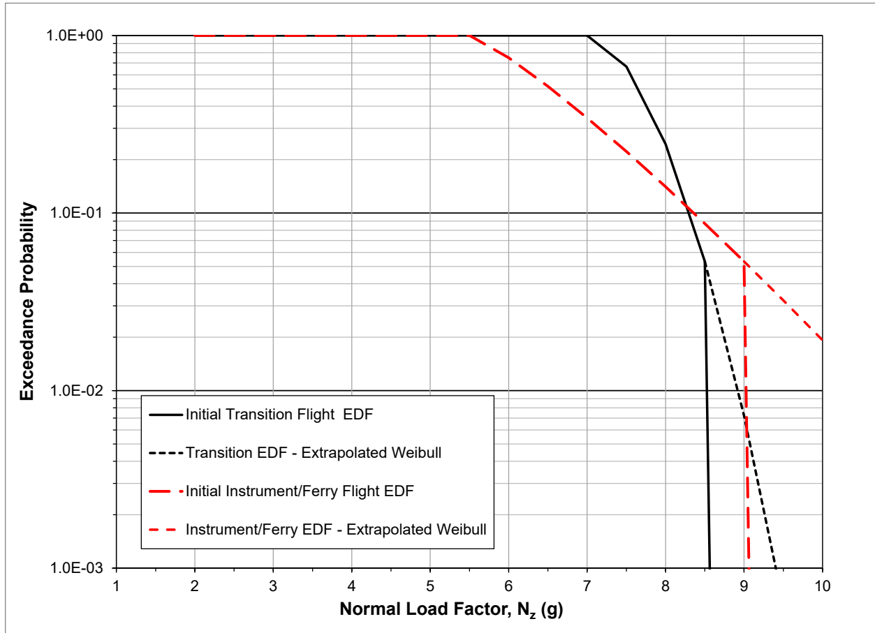
Figure 47. EDF Comparison for High N_z Tails
