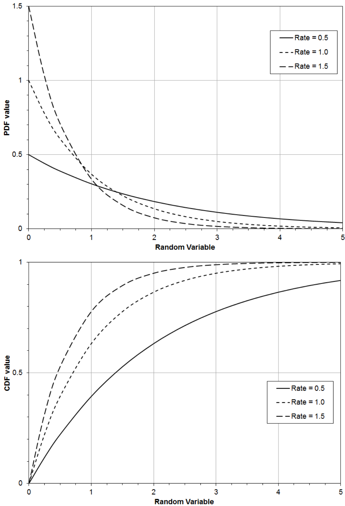
Figure 6. Exponential Probability Functions
