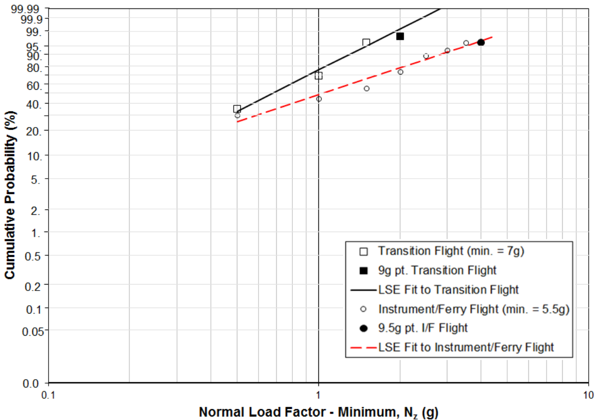
Figure 46. Weibull Plot of Extrapolation of N_z EDF to Higher N_z Values
