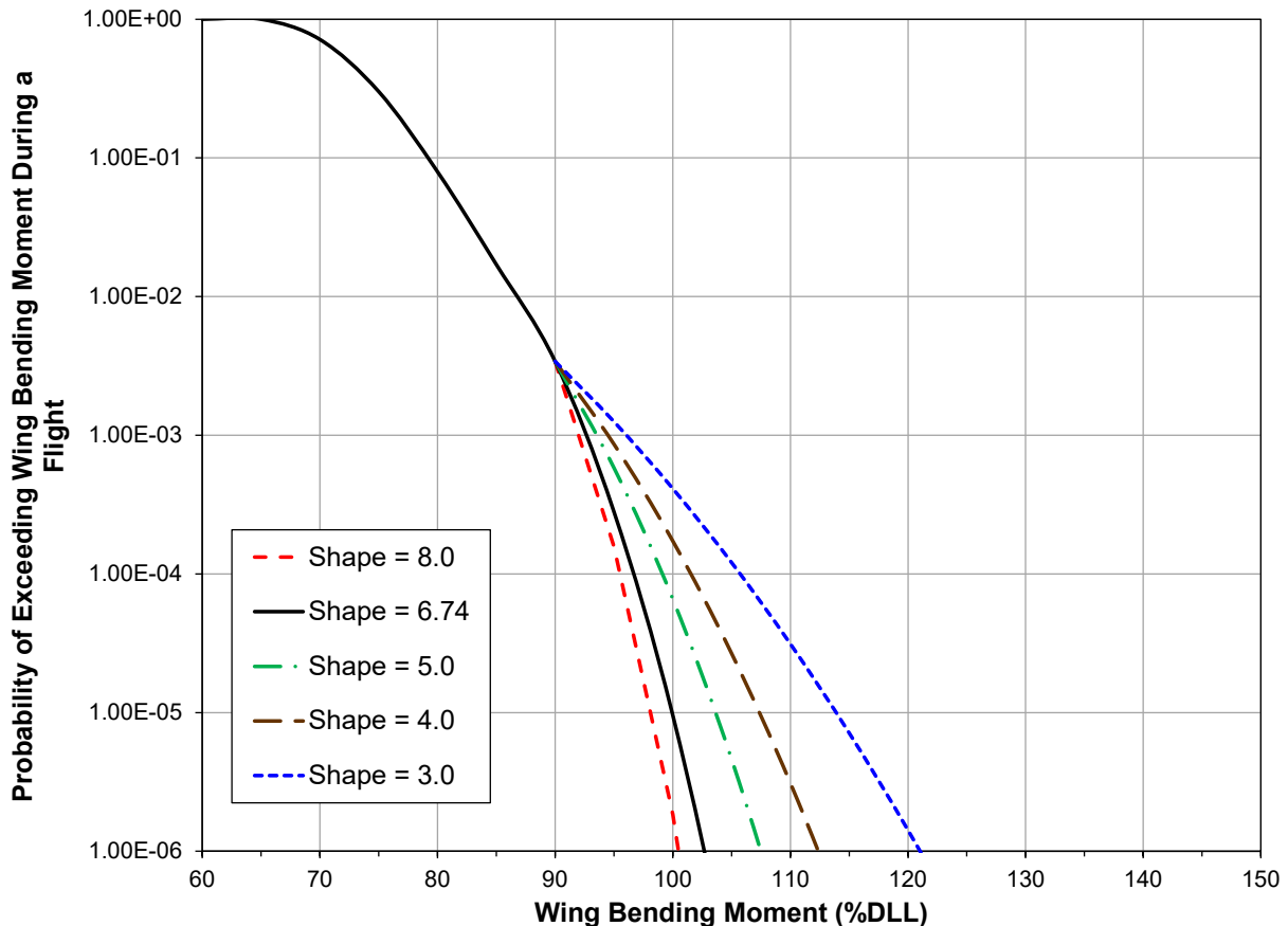
Figure 37. The Effect of Shape Parameter on Extrapolation of the EDF
