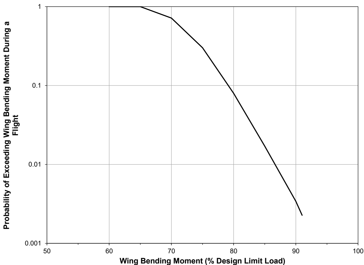
Figure 31. Probability of Exceeding WBM in a Flight
