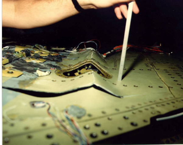
Figure 28. F-16 Block 30 Wing Failure at 128 Percent DLL
