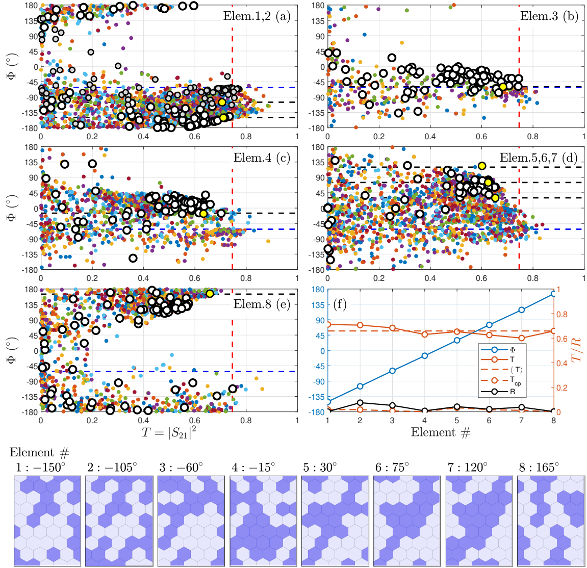
Figure 34. Repeat of Fig. 33 for the smaller-resolution 5 \times 8 hex grid, in an identical format as for the brick elements. Generally, the hex elements performed slightly better than the brick elements. The most stark difference is the reduction in reflectance, with no element generating larger than R = 0.075 , with an average of \langle R \rangle = 0.03 .
