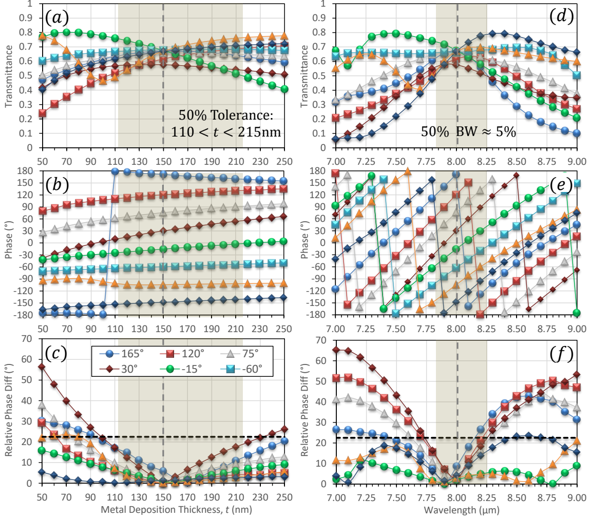
Figure 35. Variances in (a) T and (b) \Phi as a function of t for the brick designs displayed in Fig. 33, with t = 150 nm. To maintain T \geq 50\% for all \Phi_t , the metal thickness must remain between \sim 110 nm–215nm. A sufficient phase separation is maintained in this region, quantified by examining (c) the relative difference between each phase value and the reference phase for each t , as explained in the main text. (d,e,f) Spectral dispersion for these same metrics. The 3dB bandwidth is limited to just under 5%.
