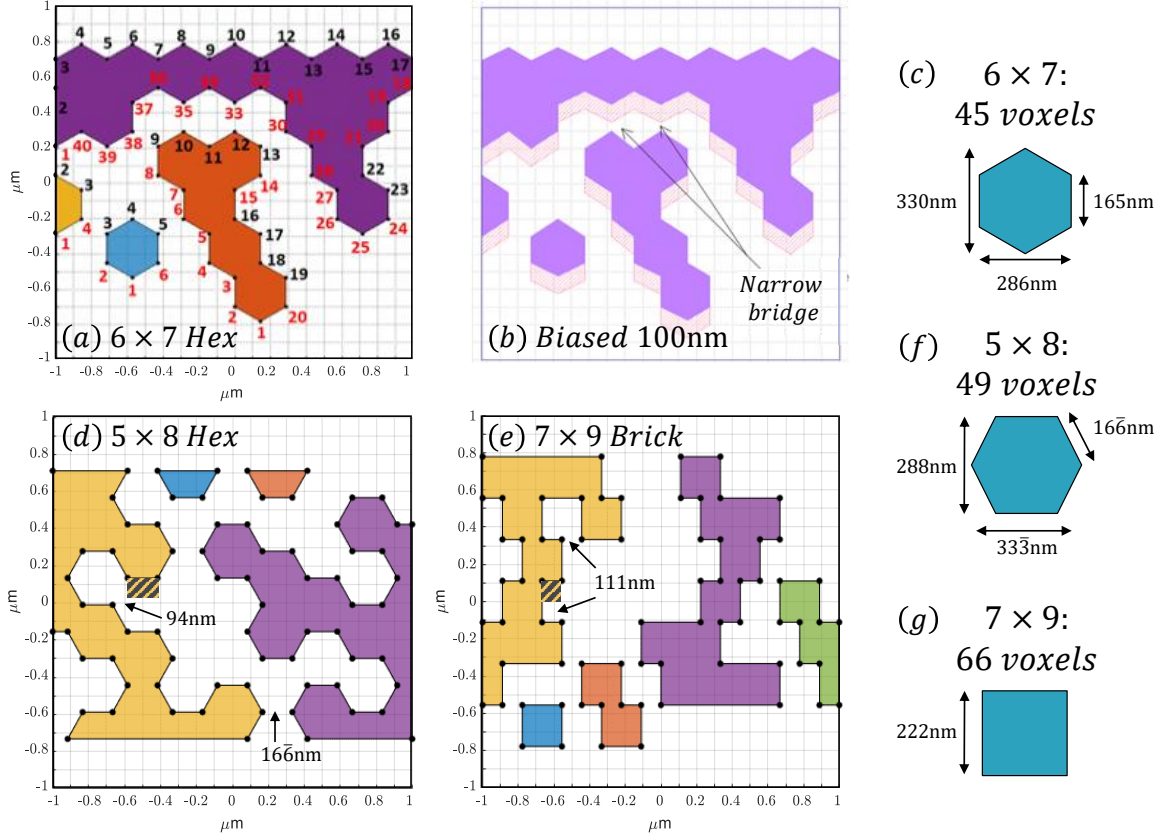
Figure 38. (a) Example 6 \times 7 hex layout showing all non-redundant exterior points, representing a coordinate pair used to draw the contours for lithographic writing of the membrane. However, the original orientations (b,c for hex example) left extremely small gaps when biased 100nm, as required. These orientations were rotated by 90^\circ (f,g) to permit more practical minimum gap widths of 94nm for hex (d) and 111nm for brick (e).
