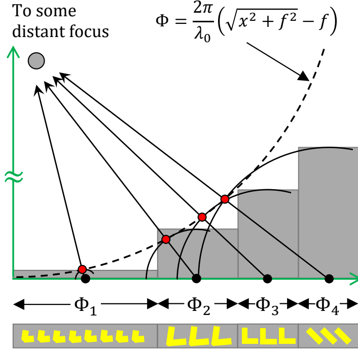
Figure 3. A parabolic phase profile (black, dashed) according to Eq. 2 can be discretized by phase zones (grey) of some determined phase \Phi_i (black dot) which are all in phase along the contour (red dot), and thus all in phase at some distant focal point (0, f) .
