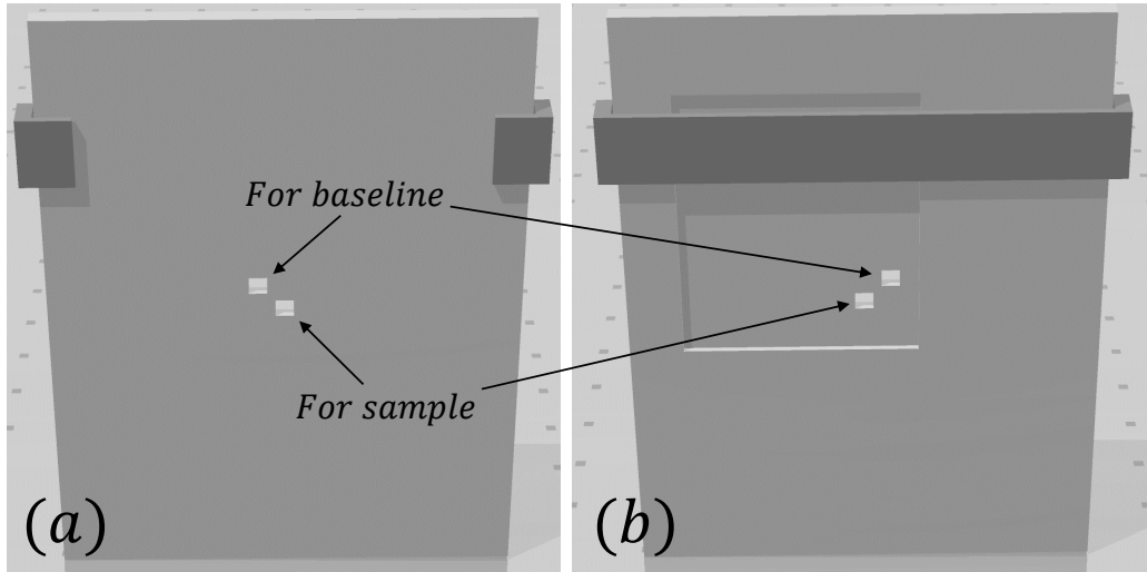
Figure 48. The (a) incidence side and (b) transmittance side of a custom sample holder designed to isolate the 2\text{mm} \times 2\text{mm} beamsteerer. It consists of a slab with two entrance apertures: one that isolates the irradiation of the sample, and one that isolates the baseline, unmetalized cavity array. A recessed region in which the sample sits is cut such that the metasurface is exactly aligned with the center aperture. A bracket was custom fit to slide over the Si wafer and brace it down, allowing unobstructed view of the entire 180^\circ observation range of \theta_t
