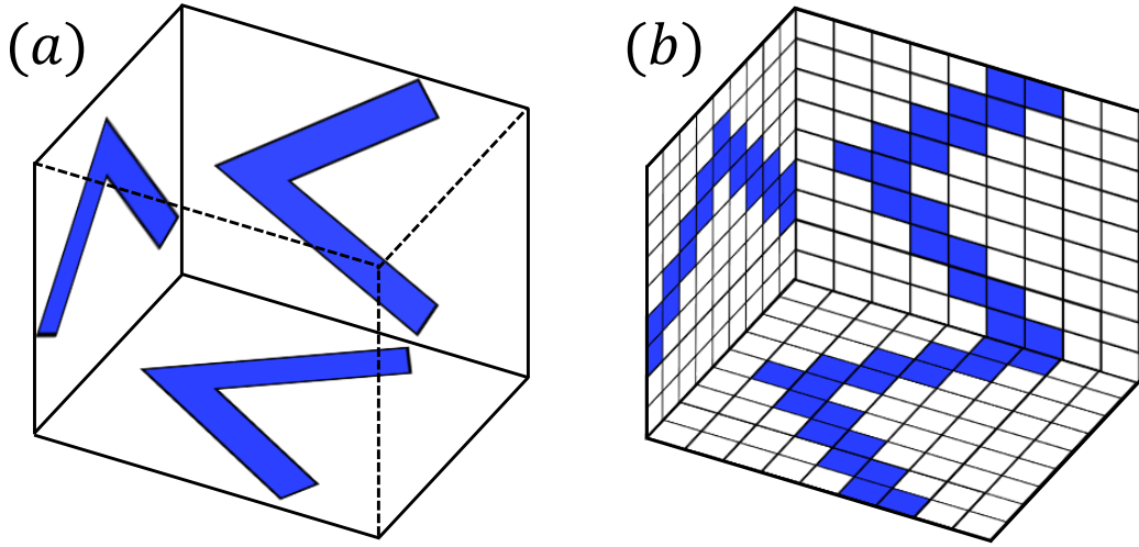
Figure 6. Concept 3D architecture for supporting out-of-plane (OOP) scatterer. (a) An analog scatterer can be supported on vertical walls and the floor of a cavity. (b) By deconstructing the walls into M \times N grids of 3D pixels—i.e. voxels—then the grids can be optimized using a genetic algorithm routine by switching the voxels in a binary operation to either a “1” for metal or a “0” for air.
