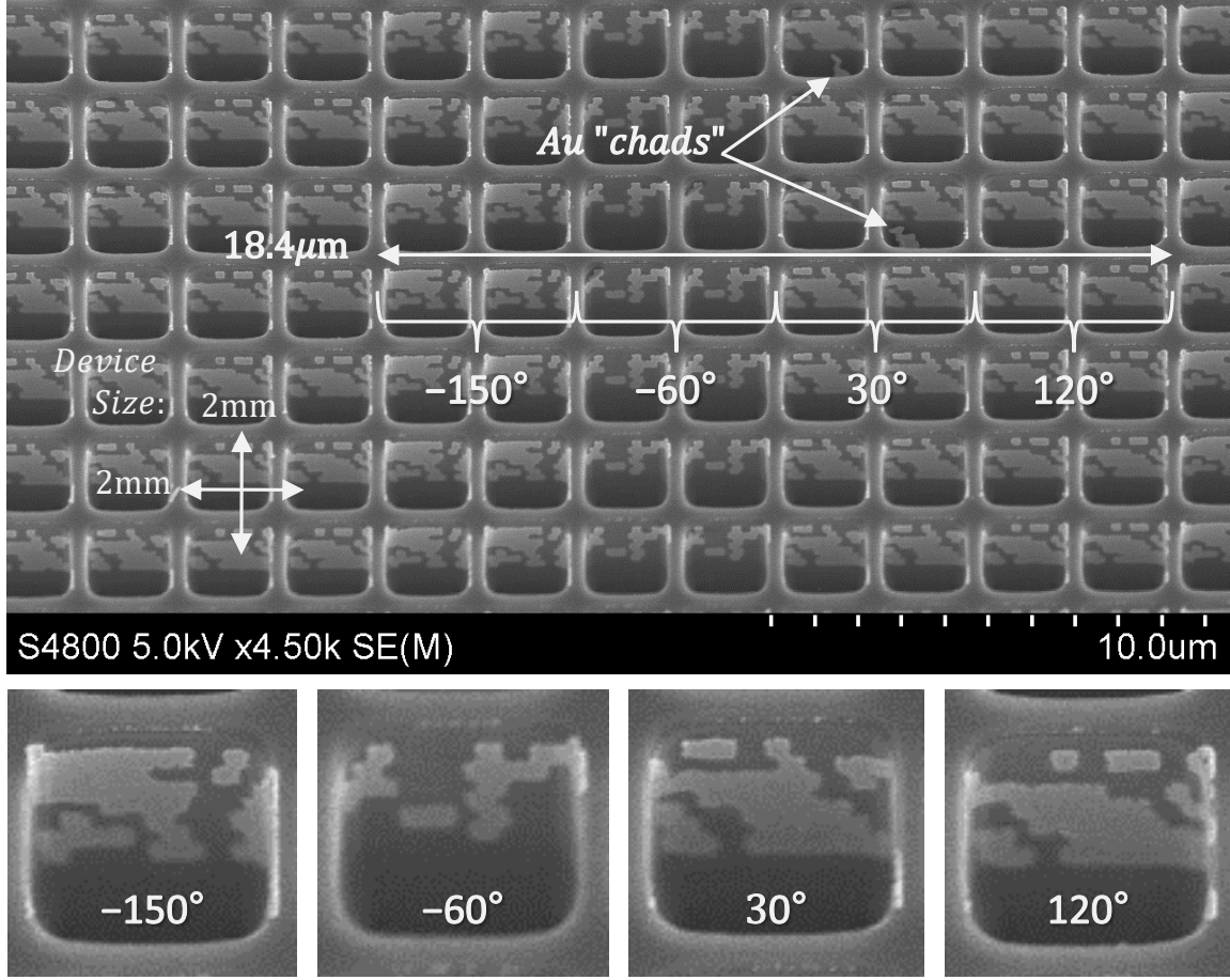
Figure 43. An SEM of the final, full-scale experimental beamsteering device, along with enlarged images of each element. Comparing to the GDS layouts in Fig. 42, the elements came out in excellent form, faithfully recreated with the least amount of clipping and improved registration over previous fab tests. The smallest features are the 111nm are clearly discernible, with good element-to-element reproducibility.
