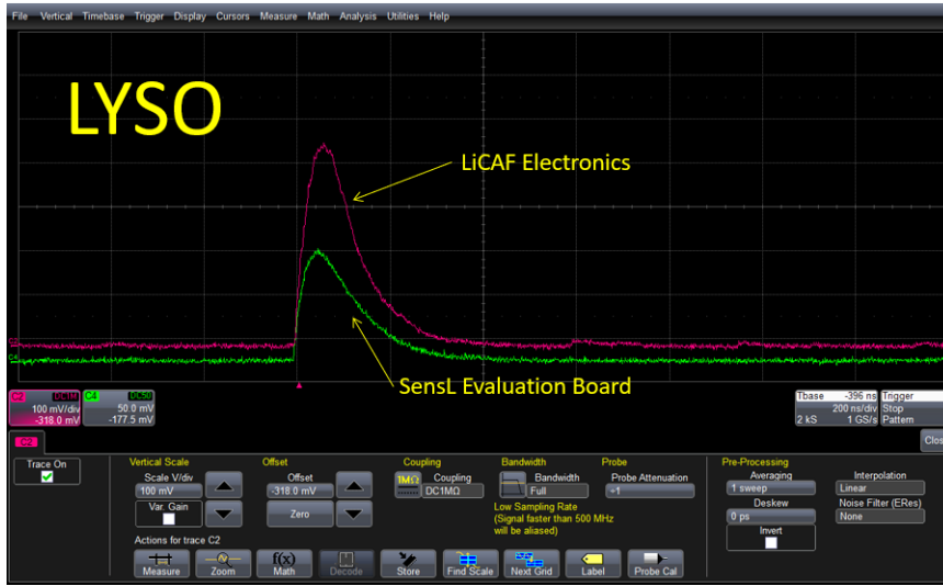
Figure 30. The analog test signal from a 4 mm \times 4 mm LYSO crystal using both the SensL evaluation board, and the custom electronics.
