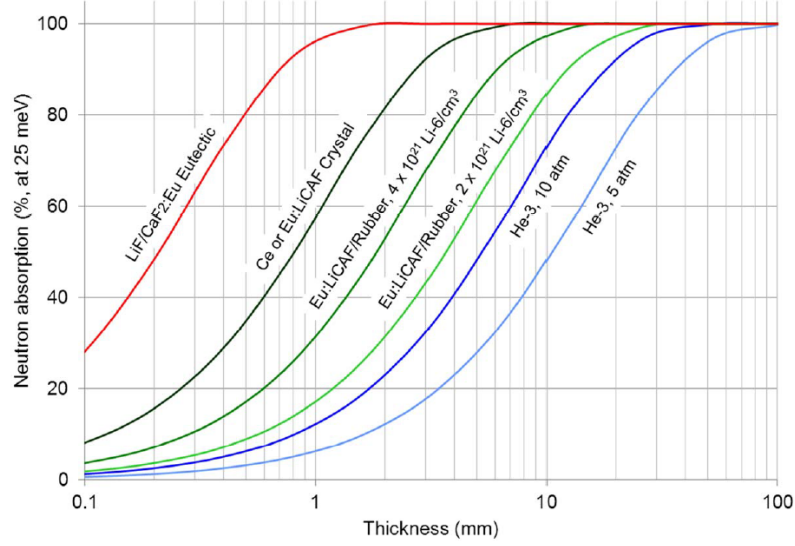
Figure 71. The detection efficiency for 25 meV neutrons for various materials [1].
