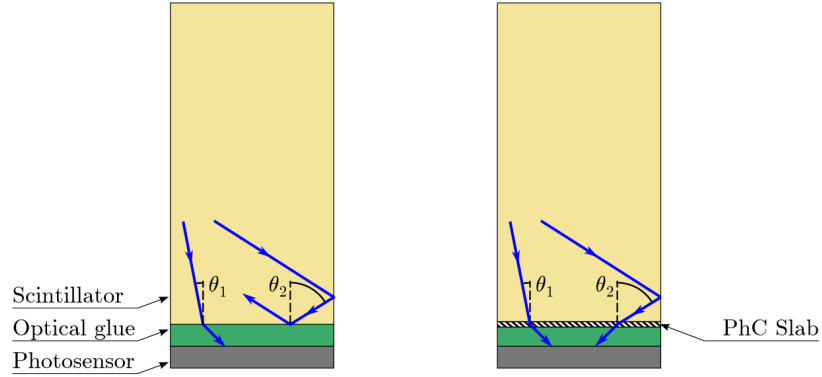
Figure 20. Proposed method to increase the light collection efficiency from the crystal to the SiPM using Photonic Crystals (PhCs) [33].
