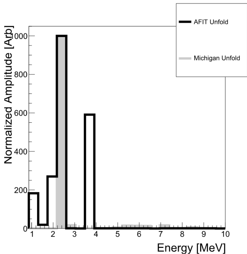
Figure 53. Results of MAXED runs at a temperature reduction factor of 0.85 for the first five layers of University of Michigan spectrometer data, versus the full 10 layer unfold of AFIT data. The incident neutron energy is deconvoluted with an a priori spectrum of monoenergetic 2.45 MeV neutrons.
