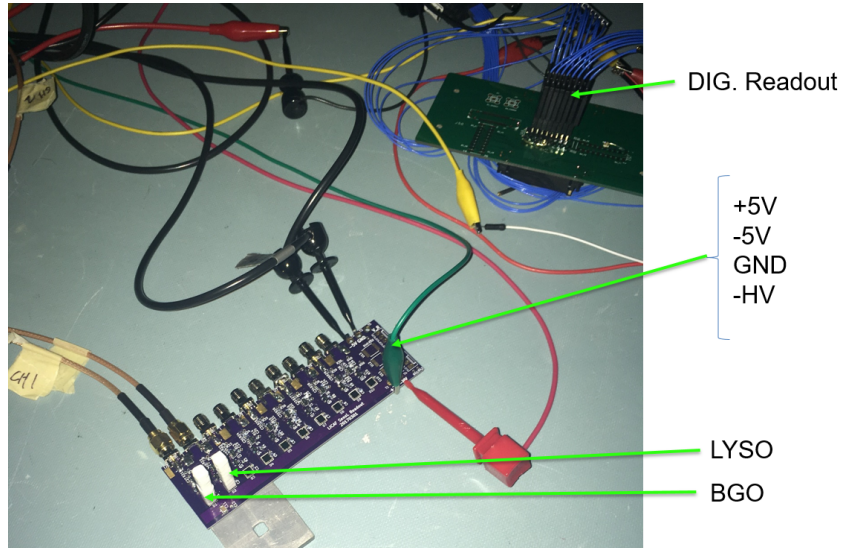
Figure 28. The fabricated circuit board being evaluated with both BGO and LYSO crystals. The BGO was used because it has a slower decay signal with high light output (similar to LiCAF) and the LYSO was used to evaluate the timing performance of the circuit since it has a very fast decay time.
