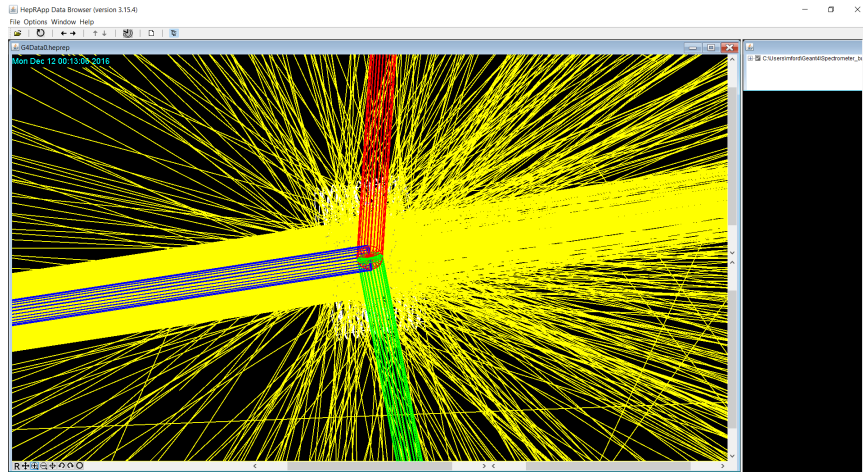
Figure 12. 1000 incident 10 MeV neutrons interacting with a 10-layer LiCAF spectrometer. It can be seen that most of the neutrons shine directly though the spectrometer.
