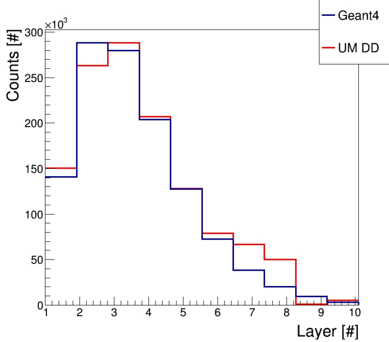
Figure 50. Comparison between Geant4 simulation and data taken after 1-hour spectrometer run at University of Michigan’s DD generator using ROOT. The experimental data matches the response function very well (within \sim 10\% ) until layers 7 and 8, where a significant increase in experimentally obtained counts is shown. The increase is likely due to backscattering of epithermal neutrons. Due to the small magnitude of the error bars, they are not represented in the plot.
