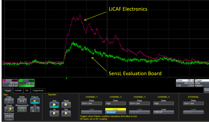
Figure 29. The analog test signal from a 4 mm \times 4 mm BGO crystal after the circuit shown in Fig 22. The BGO signal has oscillations in the falling edge, likely resulting from the relaxing time of the photocells internal to the SiPMs.
