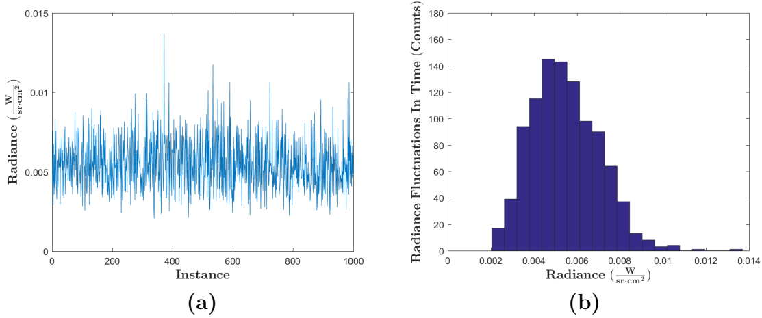
Figure 54: (a) Integrated radiance for a single projection per randomly chosen instance and (b) a histogram of these radiance fluctuations per instance.
