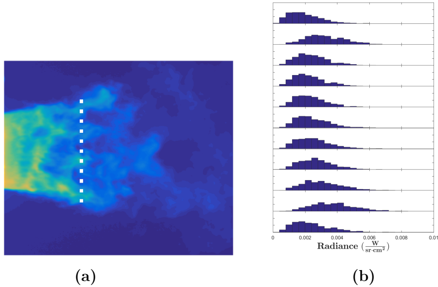
Figure 64: (a) Selected pixels in the SBFP imager and (b) the histograms of the their radiance fluctuations.
