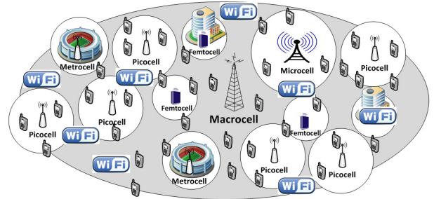
Fig. 1. An example of a large-scale, heterogeneous wireless network with various types of APs.
