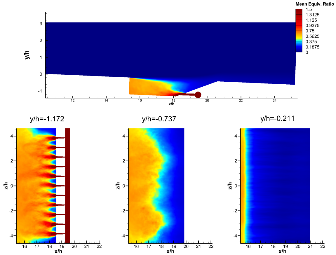
Figure 43. Time Averaged equivalence ratio with injection at 70 SLPM at the midplane (top) and three Y-planes (bottom) in the cavity, increasing in height from left to right. The far left image is on the injector plane, and the far right is in the shear layer.
