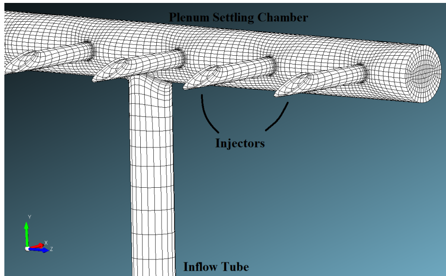
Figure 17. Isometric image from the upstream side of the plenum.
