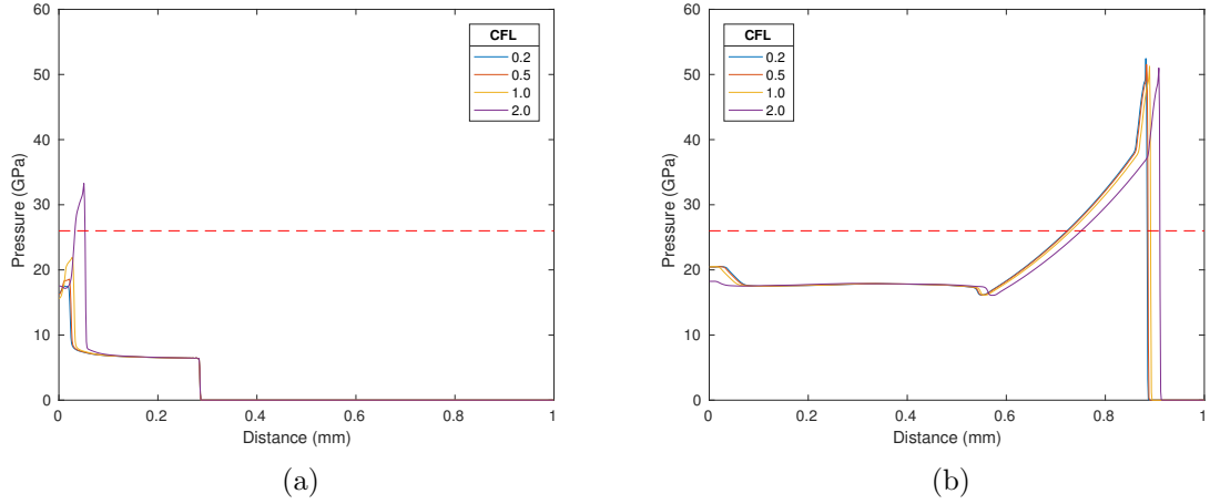
Figure 14. Temporal Refinement of MPEXS with ARCIIST: Mixture pressure ( \bar{P} ) profiles at (a) 0.1\mu s and (b) 0.2\mu s . The dashed red line (---) represents RDX CJ pressure. Piston speed of 1 km/s used in all cases.
