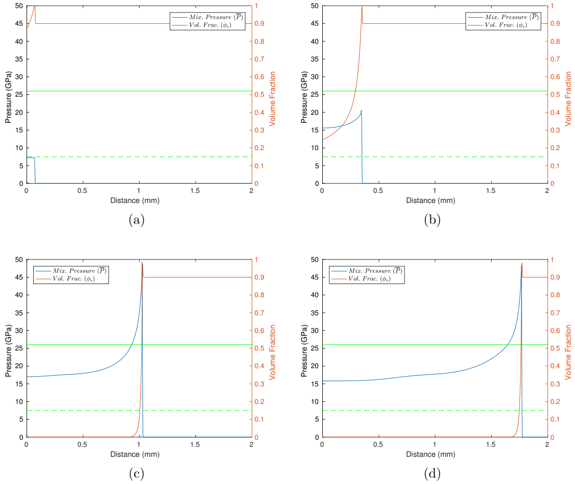
Figure 45. RDX mixture pressure ( \bar{P} ) and condensed phase volume fraction ( \phi_s ) profiles using the SIG burn model and 1 km/s piston at (a) 0.025, (b) 0.1, (c) 0.2, and (d) 0.3 \mu s . The dashed green line (---) represents expected response from the non-reacting RDX Hugoniot and the solid green line (—) represents RDX CJ pressure.
