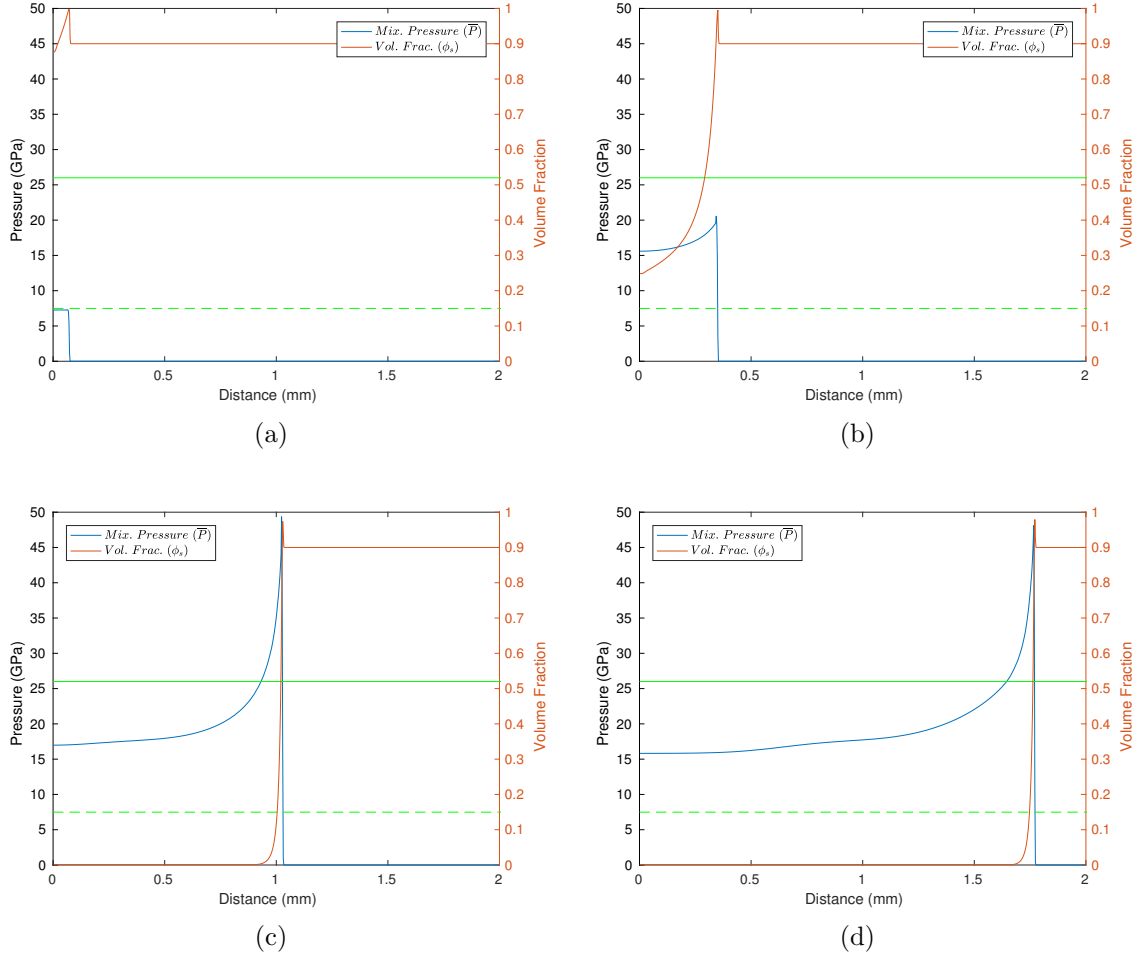
Figure 11. RDX mixture pressure ( \bar{P} ) and condensed phase volume fraction ( \phi_s ) profiles using the SIG burn model and 1 km/s piston at (a) 0.025, (b) 0.1, (c) 0.2, and (d) 0.3 \mu s. The dashed green line (---) represents expected response from the non-reacting RDX Hugoniot and the solid green line (—) represents RDX CJ pressure.
