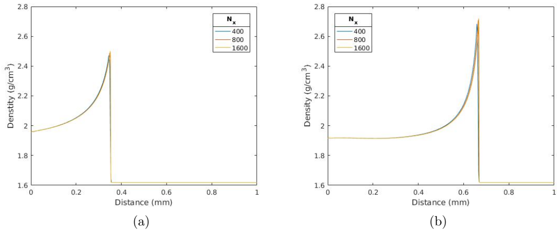
Figure 53. Spatial Refinement of MPEXS with SIG: Mixture density ( \bar{\rho} ) profiles at (a) 0.1\mu s and (b) 0.15\mu s . Piston speed of 1 km/s used in all cases.
