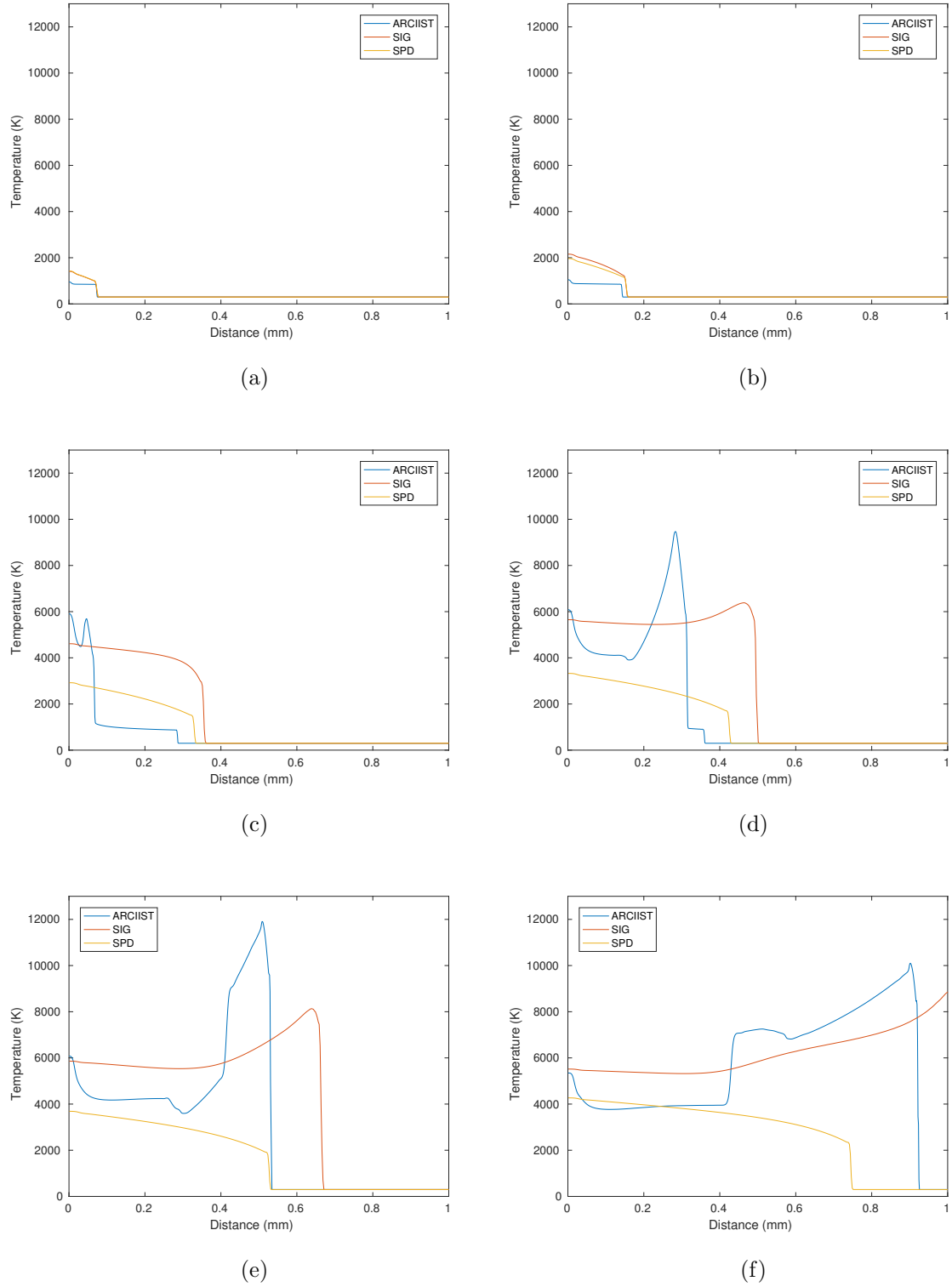
Figure 31. Comparison of RDX mixture temperature ( \bar{T} ) profiles using SPD, SIG, and ARCIIST with a 1.0 km/s piston at (a) 0.025, (b) 0.05, (c) 0.1, (d) 0.125, (e) 0.15, and (f) 0.2 \mu s .
