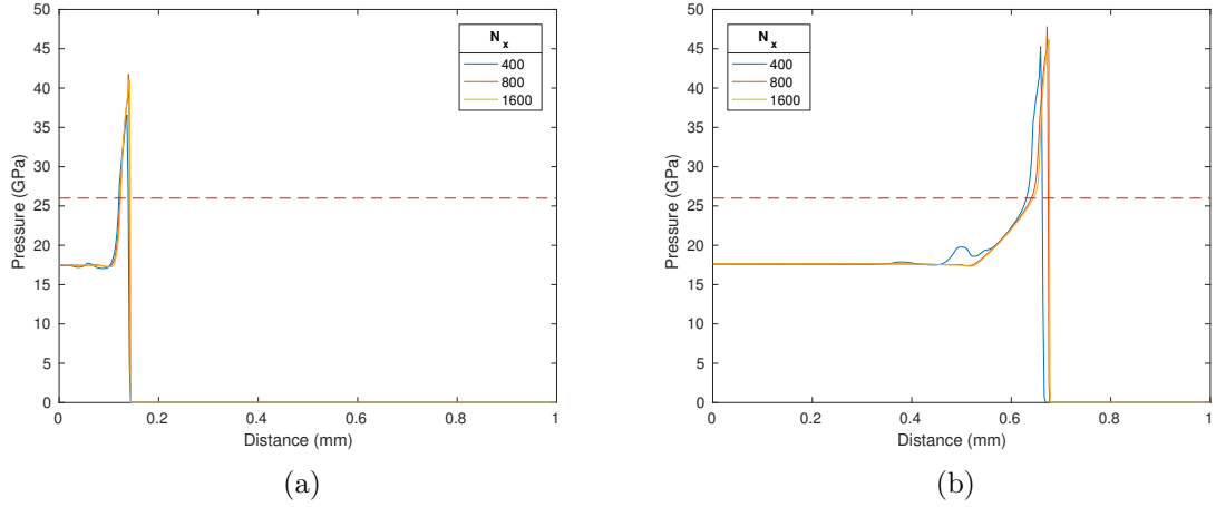
Figure 18. Spatial Refinement of MPEXS with ARCIIST: Mixture pressure ( \bar{P} ) profiles at (a) 0.025\mu s and (b) 0.1\mu s . The dashed red line ( - - ) represents RDX CJ pressure. Piston speed of 1.2 km/s used in all cases.
