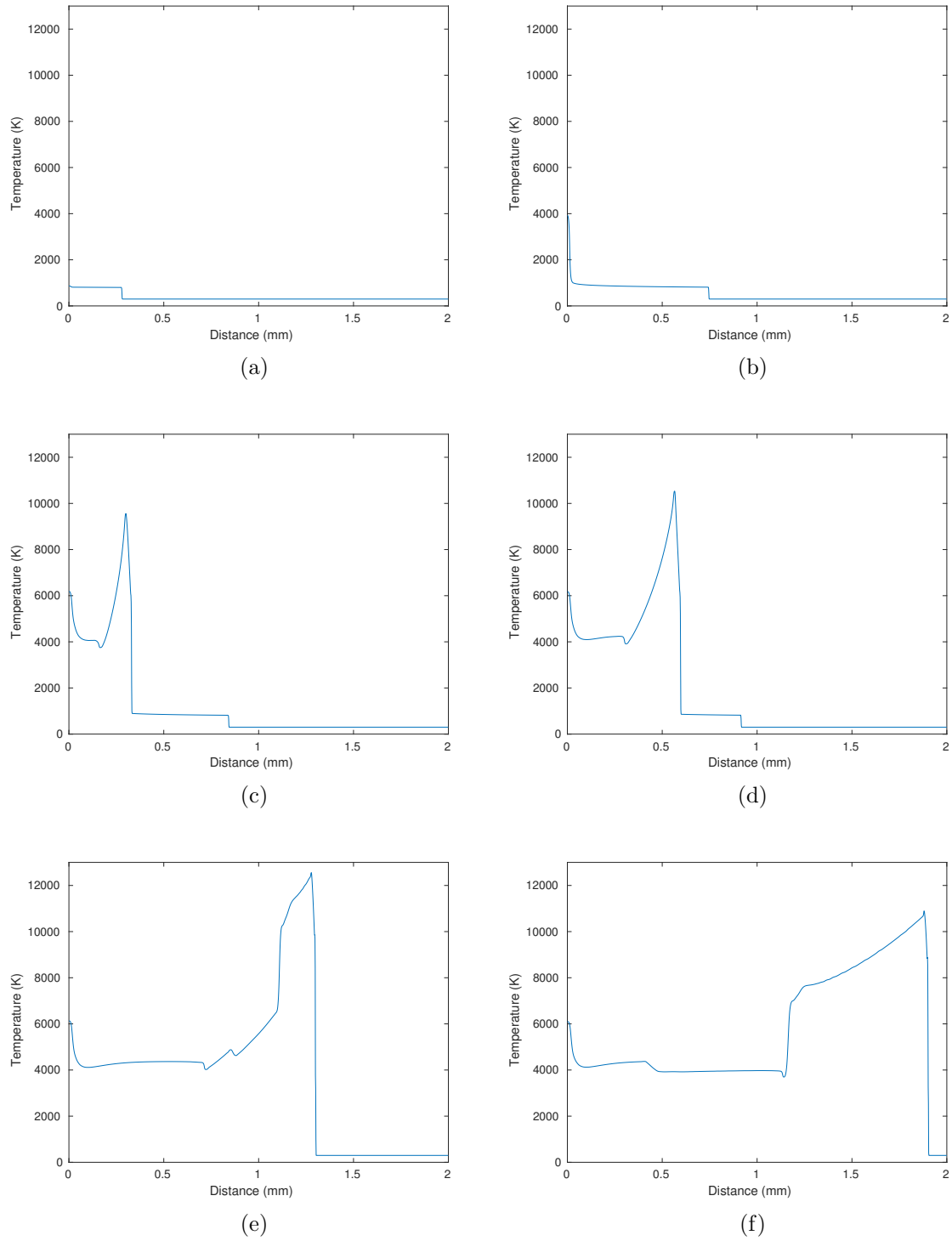
Figure 56. RDX mixture temperature ( \bar{T} ) profiles using ARCIIST with a 0.96 km/s piston at (a) 0.1, (b) 0.265, (c) 0.3, (d) 0.325, (e) 0.4, and (f) 0.475 \mu\text{s} .
