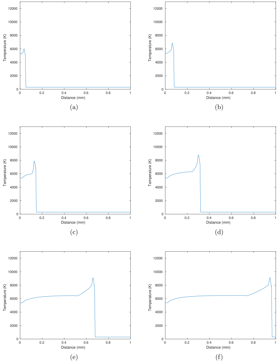
Figure 61. RDX mixture temperature ( \bar{T} ) profiles using ARCIIST with a 1.2 km/s piston at (a) 0.01, (b) 0.015, (c) 0.025, (d) 0.05, (e) 0.1, and (f) 0.14 \mu\text{s} .
