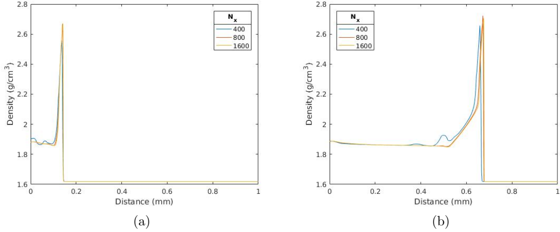
Figure 20. Spatial Refinement of MPEXS with ARCIIST: Mixture density ( \bar{\rho} ) profiles at (a) 0.025\mu s and (b) 0.1\mu s . Piston speed of 1.2\text{ km/s} used in all cases.
