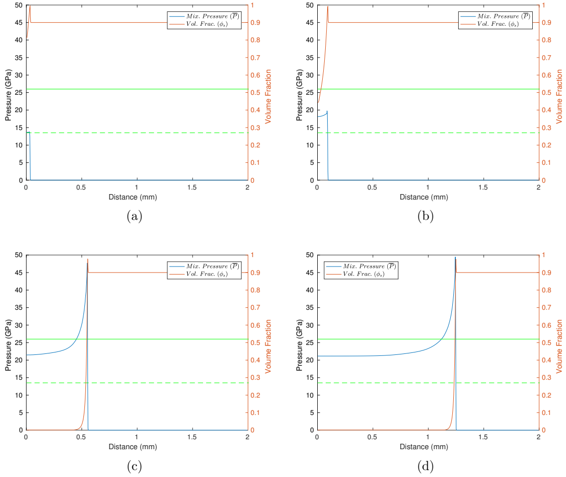
Figure 46. RDX mixture pressure ( \bar{P} ) and condensed phase volume fraction ( \phi_s ) profiles using the SIG burn model and 1.5 km/s piston at (a) 0.01, (b) 0.025, (c) 0.1, and (d) 0.2 \mu s . The dashed green line (---) represents expected response from the non-reacting RDX Hugoniot and the solid green line (—) represents RDX CJ pressure.
