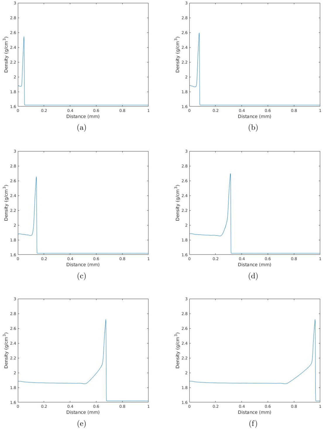
Figure 62. RDX mixture density ( \bar{\rho} ) profiles using ARCIIST with a 1.2 km/s piston at (a) 0.01, (b) 0.015, (c) 0.025, (d) 0.05, (e) 0.1, and (f) 0.14 \mu s .
