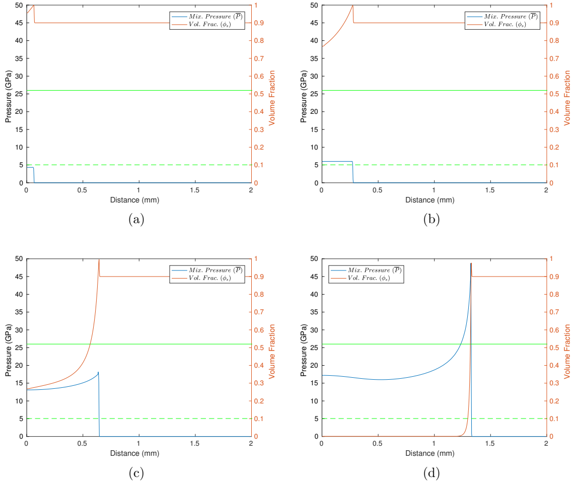
Figure 44. RDX mixture pressure ( \bar{P} ) and condensed phase volume fraction ( \phi_s ) profiles using the SIG burn model and 0.75 km/s piston at (a) 0.025, (b) 0.1, (c) 0.2, and (d) 0.3 \mu\text{s} . The dashed green line (---) represents expected response from the non-reacting RDX Hugoniot and the solid green line (—) represents RDX CJ pressure.
