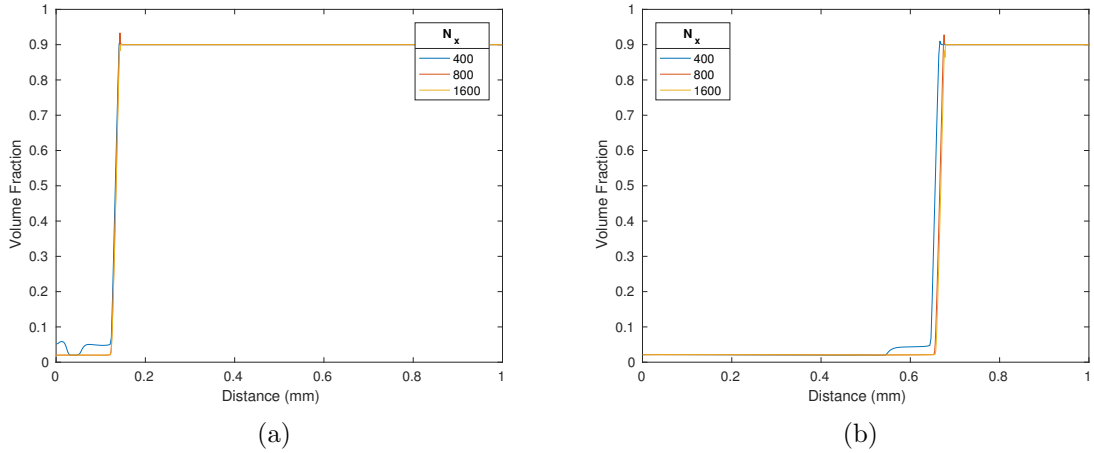
Figure 21. Spatial Refinement of MPEXS with ARCIIST: Condensed phase volume fraction ( \phi_s ) profiles at (a) 0.025\mu s and (b) 0.1\mu s . Piston speed of 1.2\text{ km/s} used in all cases.
