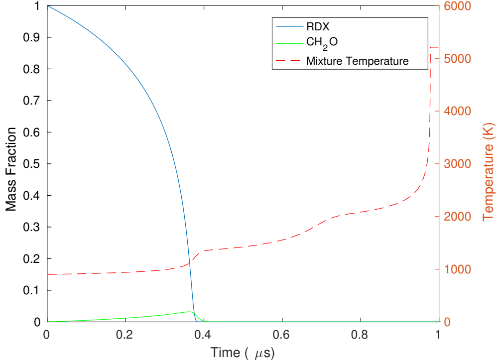
Figure 5. 0D CVTEX simulation of RDX with initial conditions \bar{T}_o = 900\text{ K} and \bar{\rho}_o = 1.8\text{ g/cm}^3 : mass fraction evolution of RDX and condensed phase intermediate species CH 2 O (left axis); mixture temperature profile (right axis).
