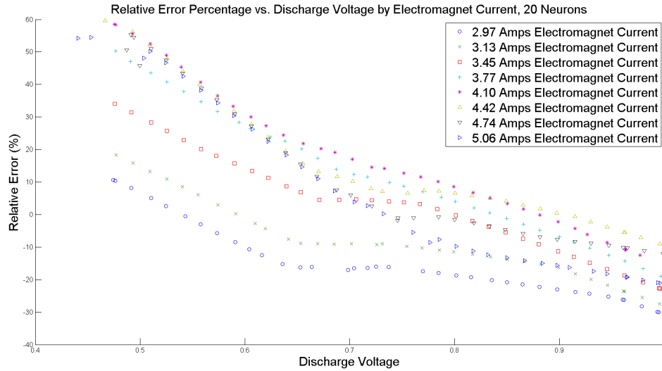
Figure 13. 20 Neuron Error % vs. Normalized Discharge Voltage and Electromagnet Current
