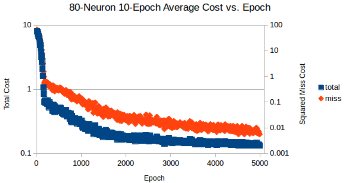
Figure 8. 80-Neuron Results
