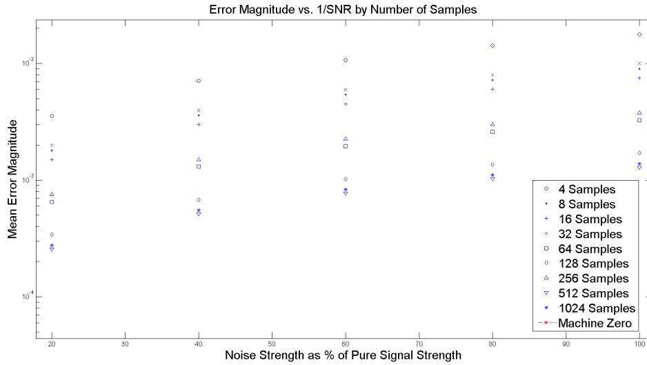
Figure 5. Close-up of the noisy data errors. Note that the error level increases approximately linearly with the noise
