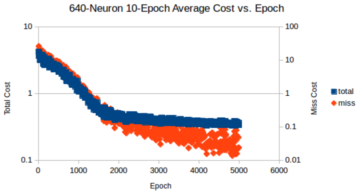
Figure 11. 640-Neuron Results
