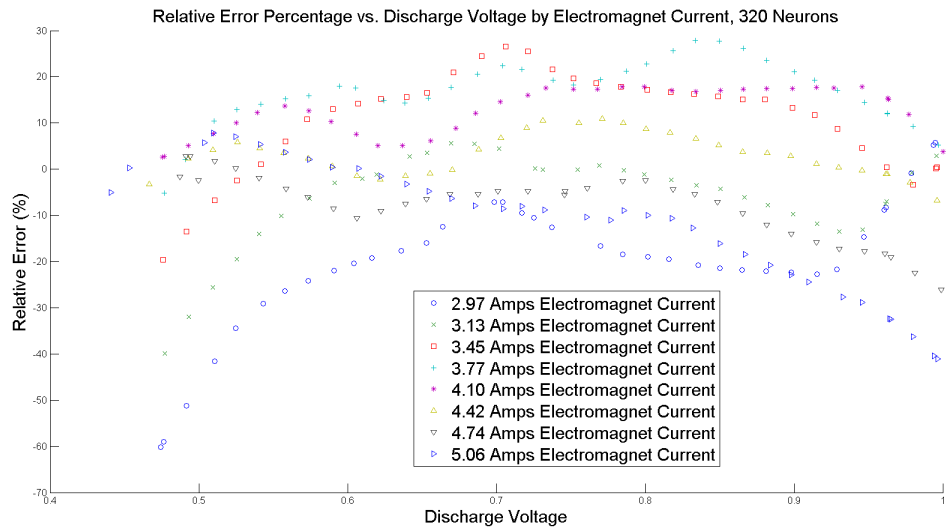
Figure 17. 320 Neuron Error % vs. Normalized Discharge Voltage and Electromagnet Current
