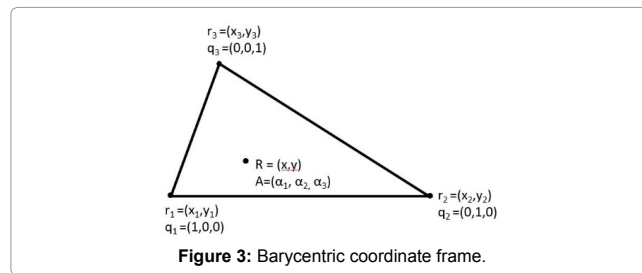
Figure 3: Barycentric coordinate frame.
