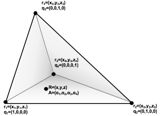
Fig. 3. Barycentric Coordinate Frame for a Tetrahedron
