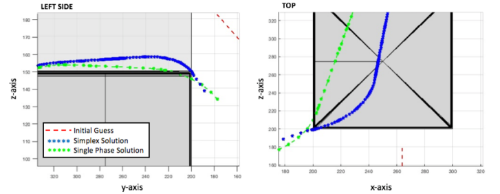
Fig. 10. Three-Dimensional Path and Constraint Comparison
