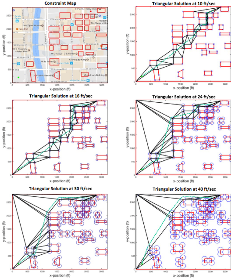
Figure 55. Triplanner Multiple Path Solutions. [Map Data @2017 Google]
