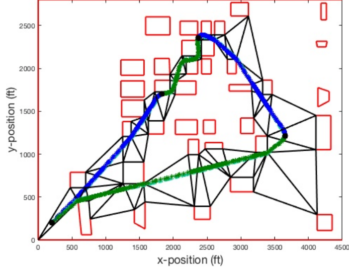
Figure 41. Multiple Waypoint Hybrid Solution
