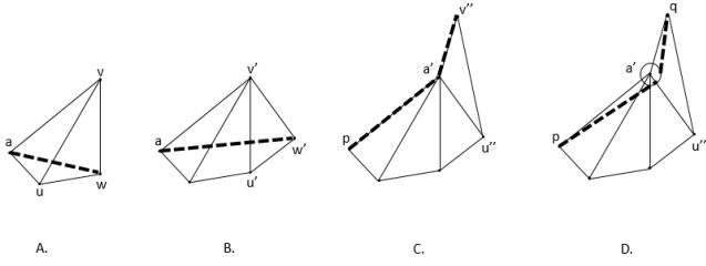
FIGURE 2. Implementation of the Funnel Algorithm on a Simplex Corridor
