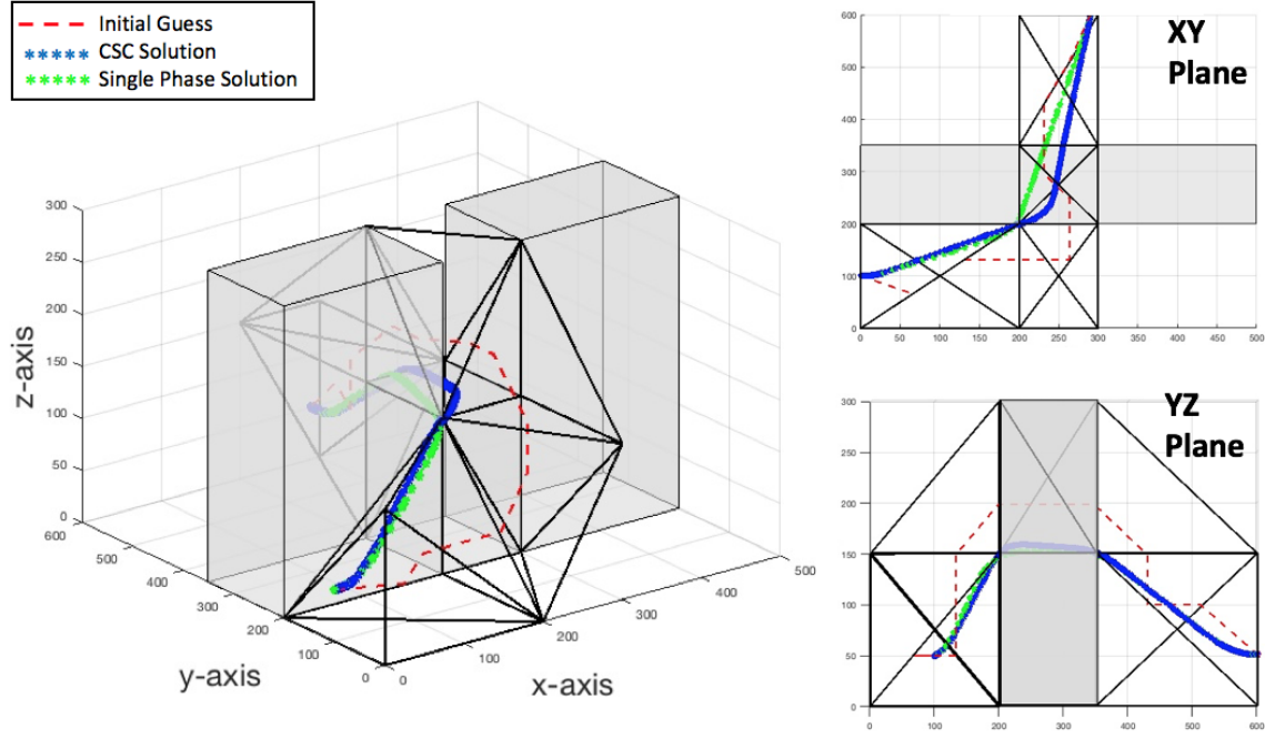
Figure 35. Three-Dimensional Optimal Path Solution Comparison
