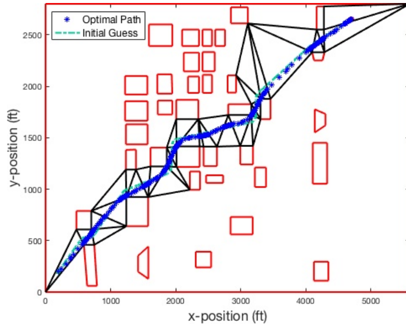
Figure 30. Two-Dimensional Hybrid Path Solution
