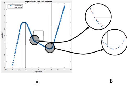
FIGURE 5. Superquadric constraint functions, illustrating converged solution for small semi-major axis with poor initial guess
