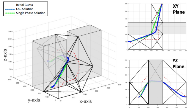
Fig. 8. Three-Dimensional Optimal Control Path Solution
