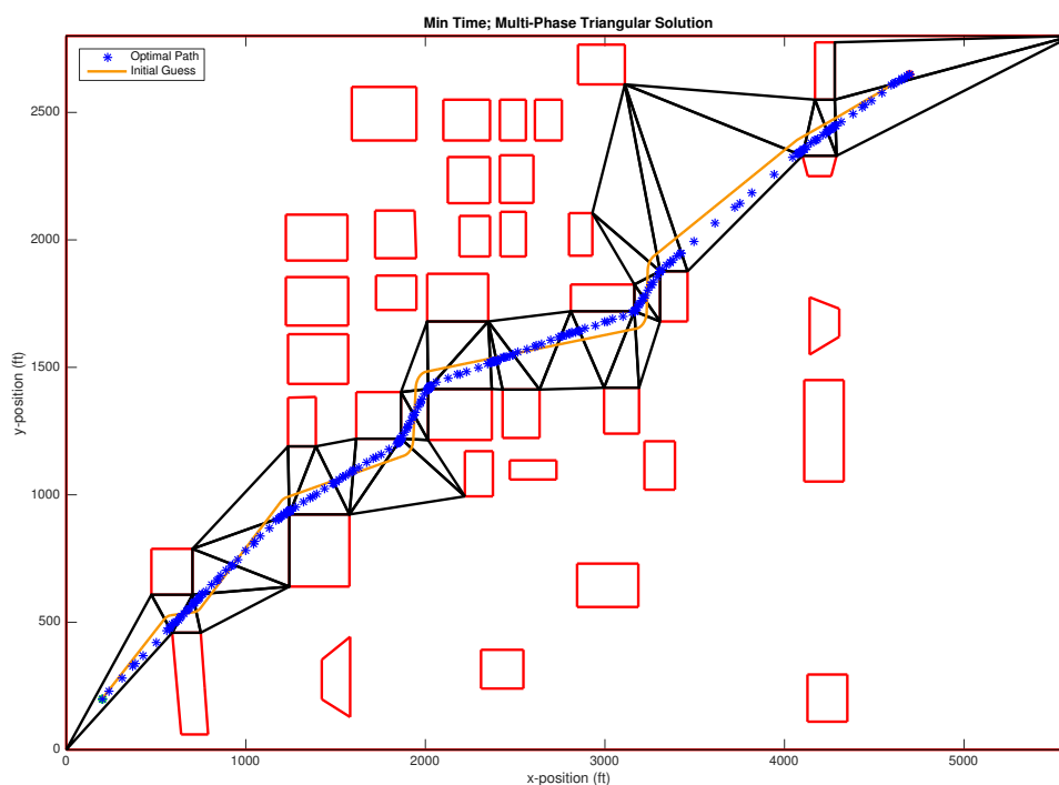
Figure 9. Hybrid Solution. Map data ©2017 Google
