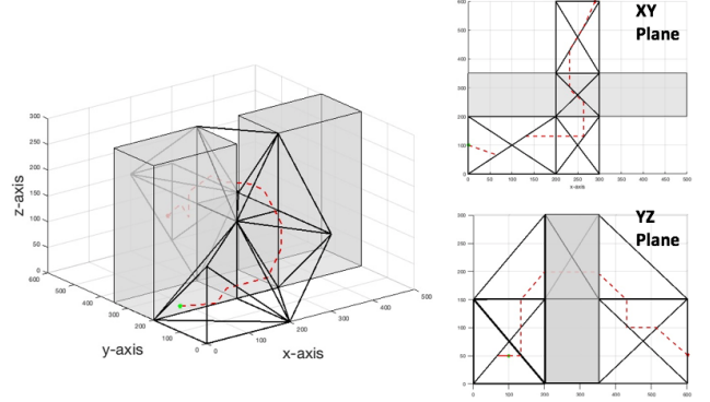
Fig. 7. Three-Dimensional Simplex Search Corridor
