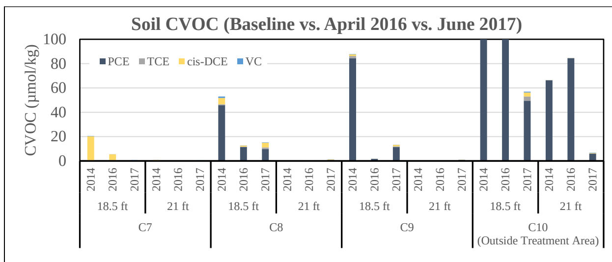
Figure 6-2. Soil CVOC Data – Comparisons Between Events
