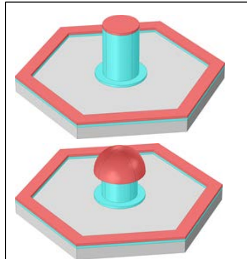
Figure 7. Pillar electrodes with flat top and with a hemispherical dome (bottom). Electrodes are coated with SIROF (red).
