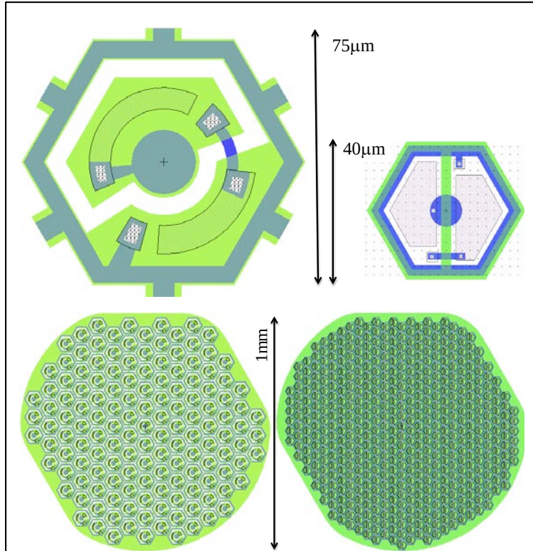
Figure 5. By eliminating the open trenches surrounding the pixels, reducing the width of the isolating trenches from 5 to 1 \mu\text{m} , and decreasing the size of the diodes, we will reduce pixel pitch from 75 to 40 \mu\text{m} . This should enable placement of more than 10,000 pixels within 20^\circ of the visual field.
