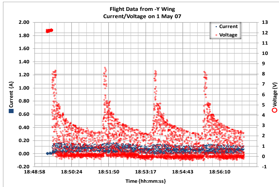
Figure A-9. Flight Data from -Y Wing on 1 May 07 (Current/Voltage)
