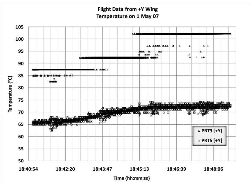
Figure 13. Flight Data from +Y Wing on 1 May 07 (Temperature)
