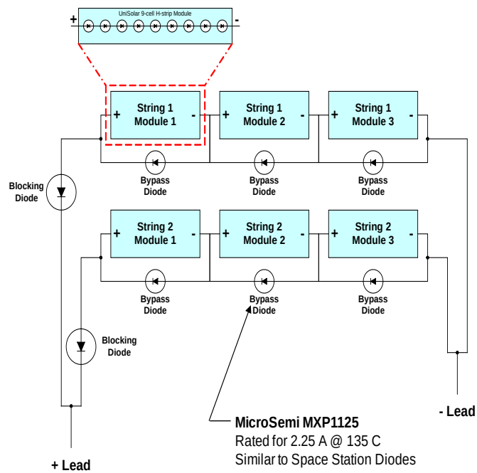
Figure 6. ExpSA Electrical Circuit Layout for One Wing
