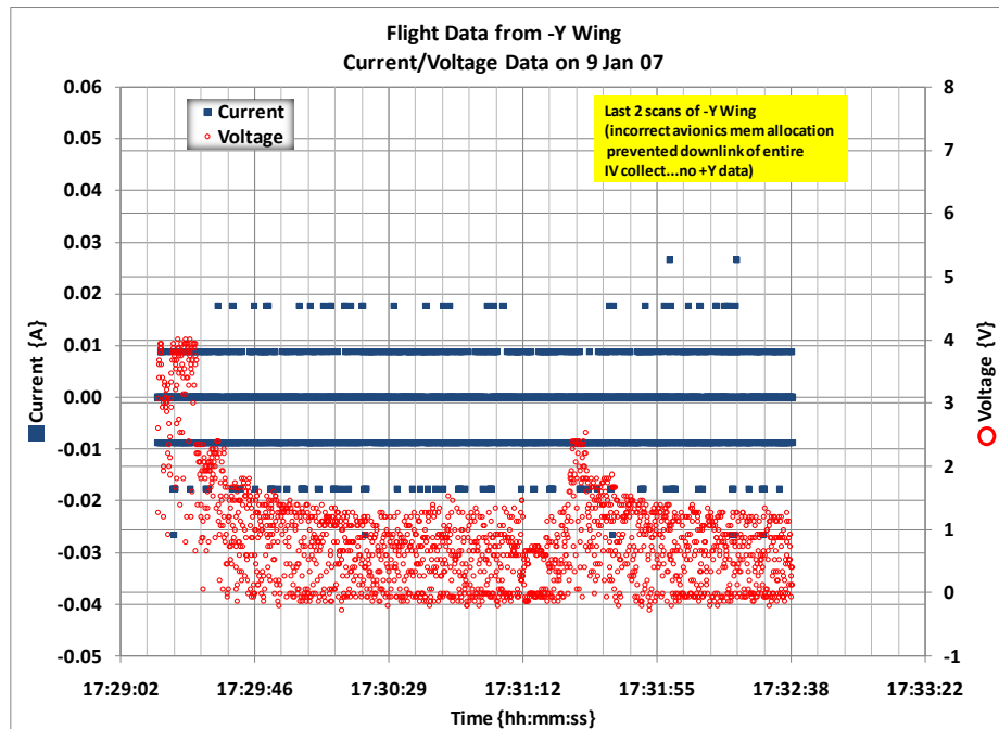
Figure A-3. Flight Data from -Y Wing on 9 Jan 07 (Current/Voltage)
