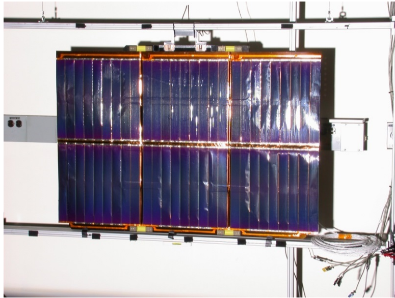
Figure 5. a-Si flight Wing Undergoing Pre-flight Electrical Performance Testing
