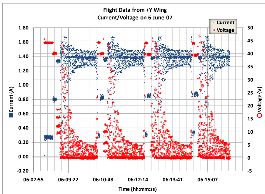
Figure 14. Flight Data from +Y Wing on 6 Jun 07 (Current/Voltage)
