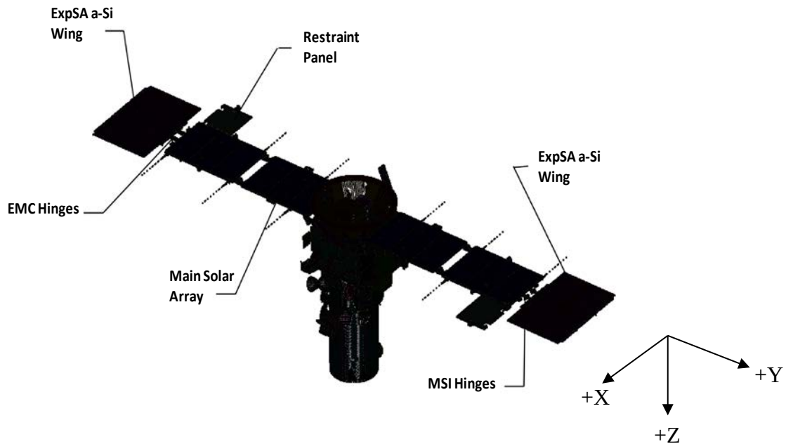
Figure 3. ExpSA Deployed on TacSat 2
