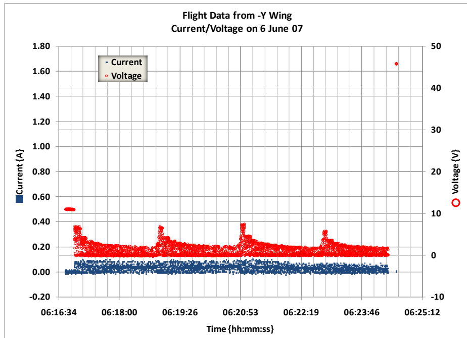
Figure A-11. Flight Data from -Y Wing on 6 Jun 07 (Current/Voltage)
