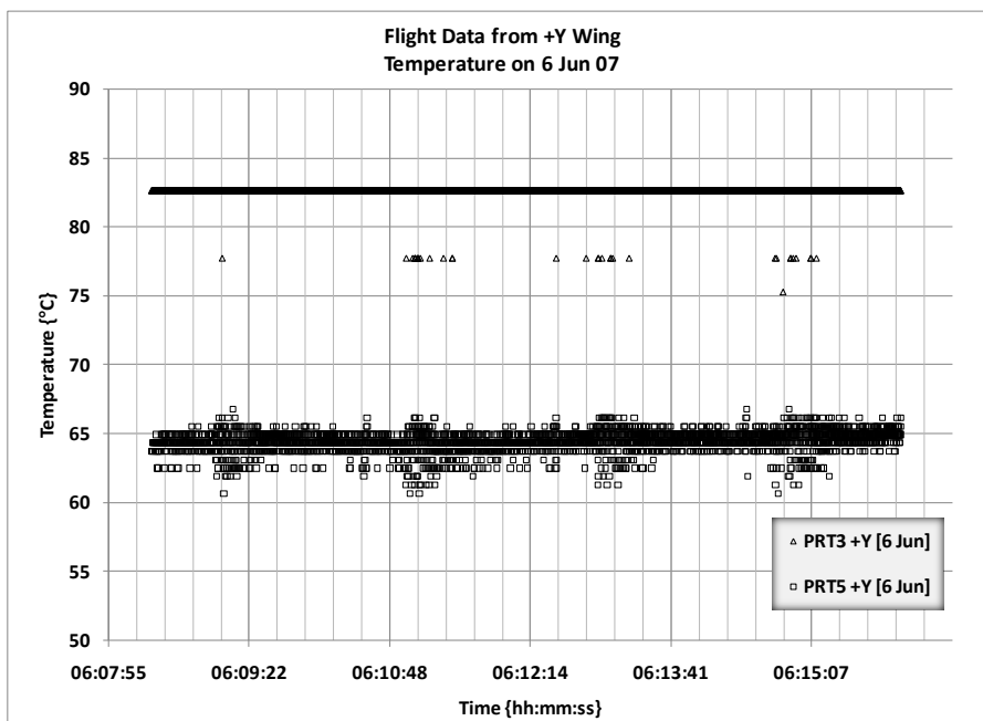
Figure 15. Flight Data from +Y Wing on 6 Jun 07 (Temperature)
