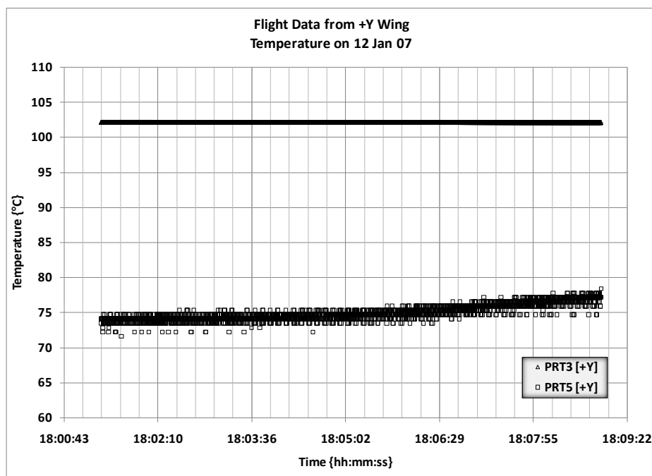
Figure A-8. Flight Data from +Y Wing on 12 Jan 07 (Temperature)
