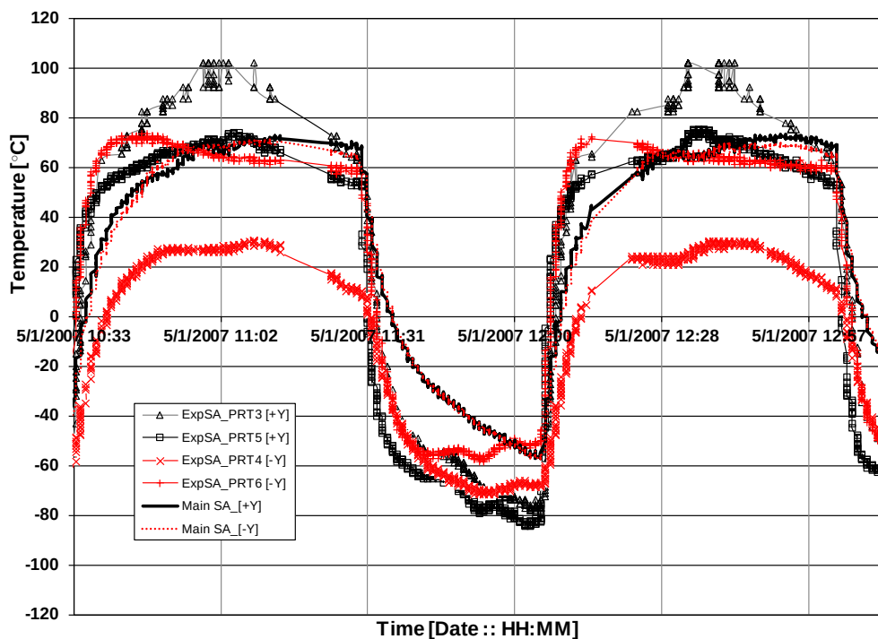
Figure 21. Example Orbital Temperature Profile (1 May 2007, ExpSA & Main Solar Arrays)
