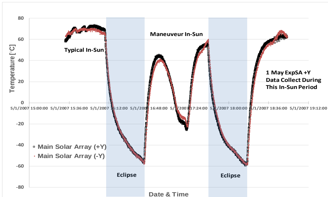
Figure 20. Main Solar Array Temperatures on 1 May 2007 (+Y and -Y)
