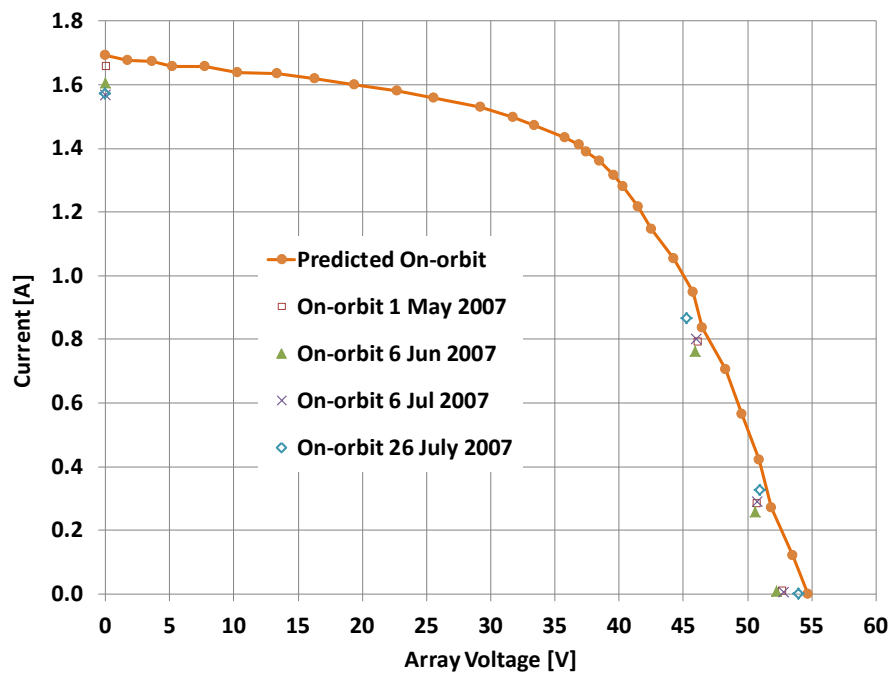
Figure 22. Comparison of On-orbit Data with Predicted Stable Current/Voltage Curve
