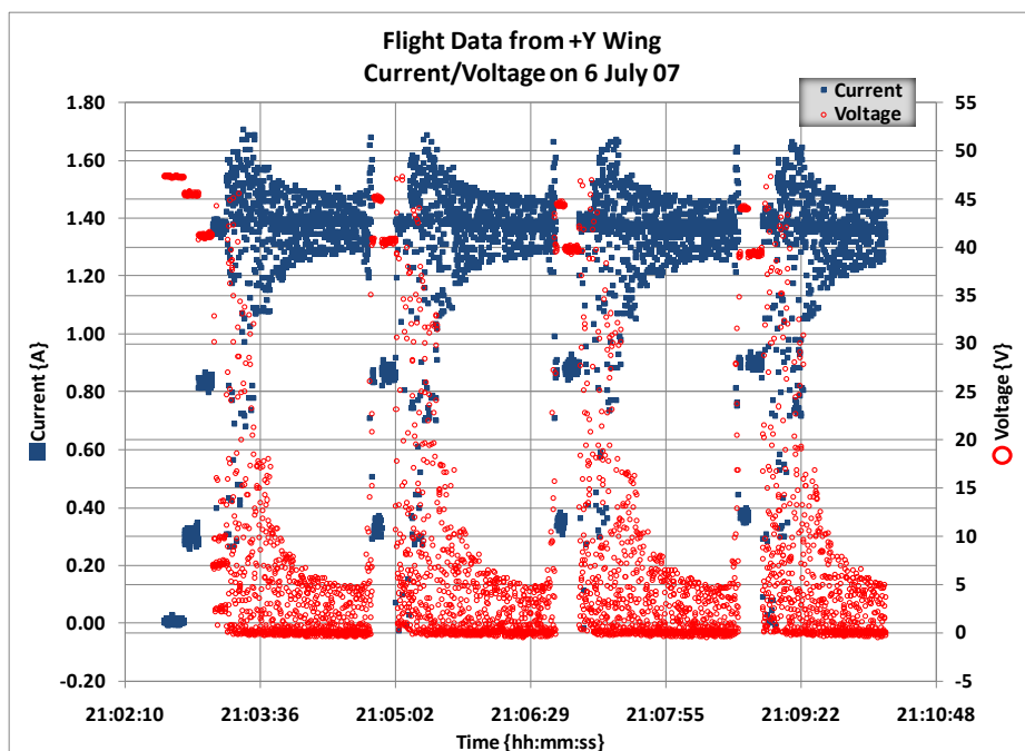
Figure 16. Flight Data from +Y Wing on 6 July 07 (Current/Voltage)
