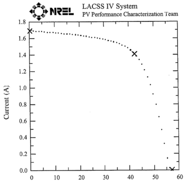
Figure 9. AM1.5 Pre-flight Electrical Performance of +Y wing (25°C)
