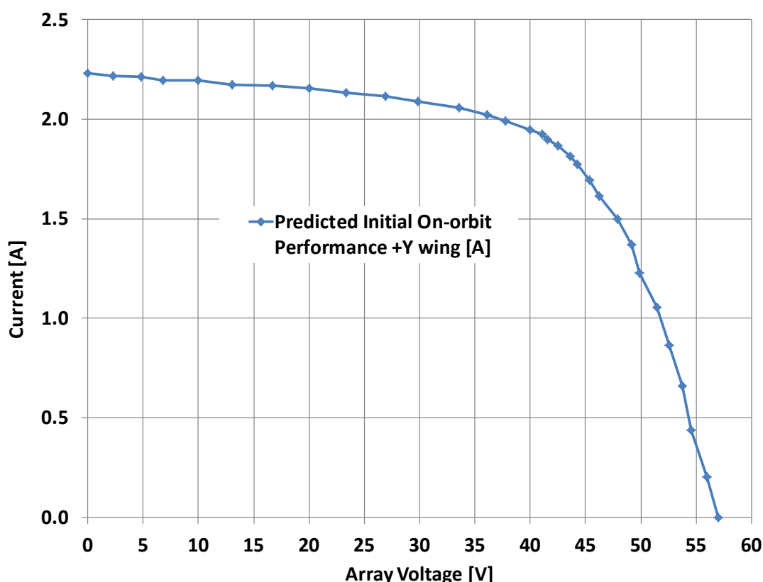
Figure 10. Predicted Initial AM0 Performance of +Y Wing (at 25°C)
