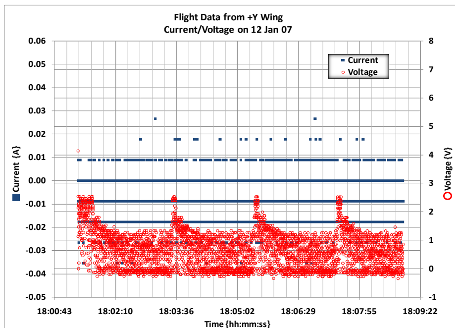
Figure A-7. Flight Data from +Y Wing on 12 Jan 07 (Current/Voltage)
