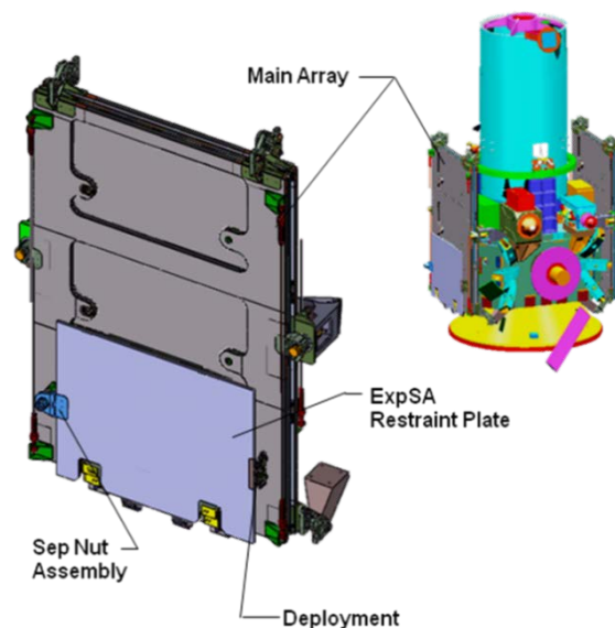
Figure 1. ExpSA Stowed (Removed from TacSat-2 and Mounted on TacSat-2)
