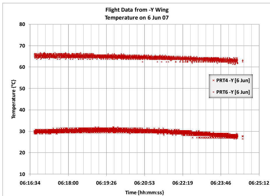
Figure A-12. Flight Data from -Y Wing on 6 Jun 07 (Temperature)
