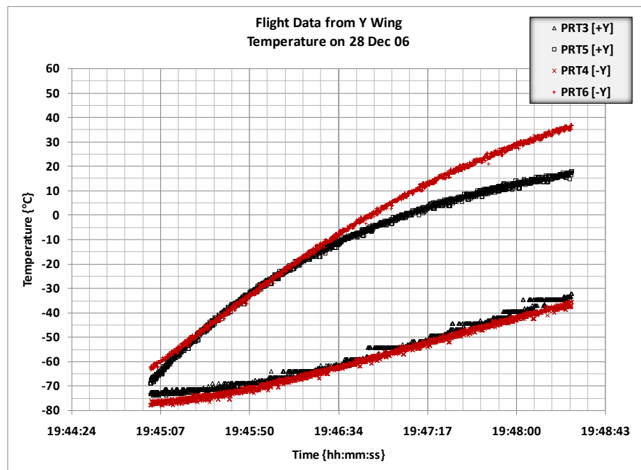
Figure A-2. Flight Data from -Y Wing on 28 Dec 06 (Temperature)
