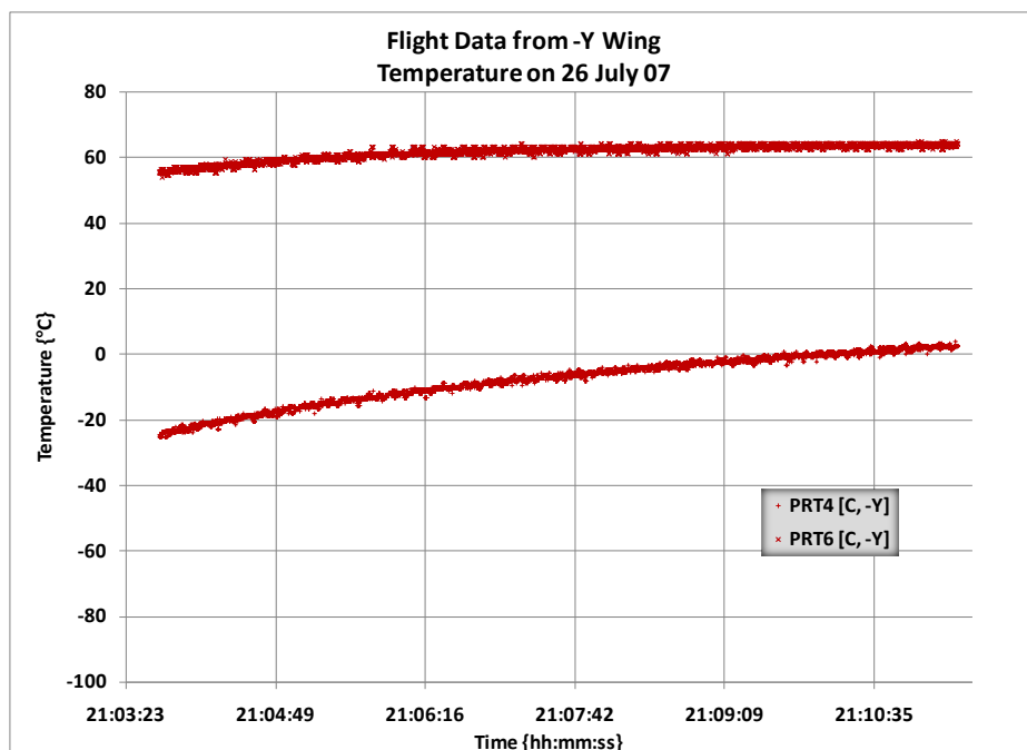
Figure A-16. Flight Data from -Y Wing on 26 July 07 (Temperature)
