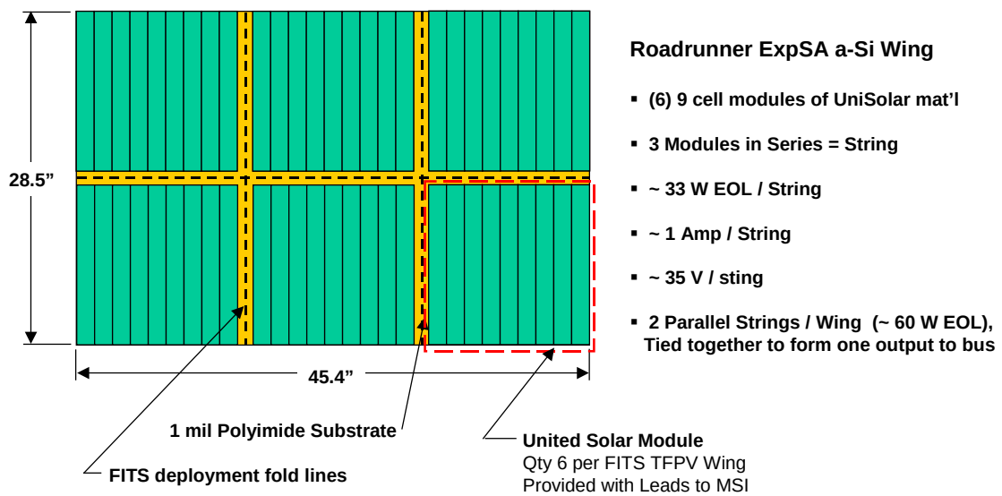
Figure 4. ExpSA a-Si TFPV Blanket Layout (EOL is End of Life)
