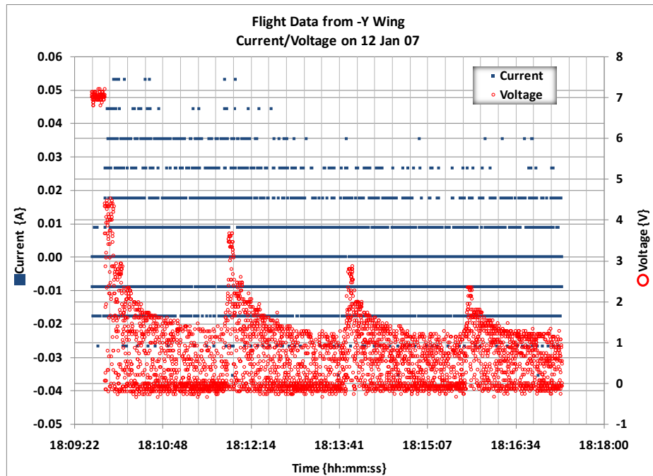
Figure A-5. Flight Data from -Y Wing on 12 Jan 07 (Current/Voltage)
