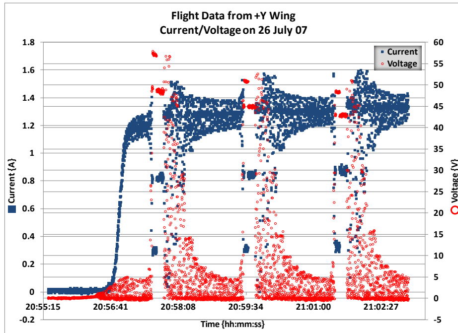
Figure 18. Flight Data from +Y Wing on 26 July 07 (Current/Voltage)
