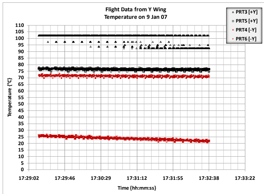
Figure A-4. Flight Data from +/-Y Wing on 9 Jan 07 (Temperature)
