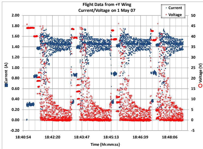
Figure 12. Flight Data from +Y Wing on 1 May 07 (Current/Voltage)
