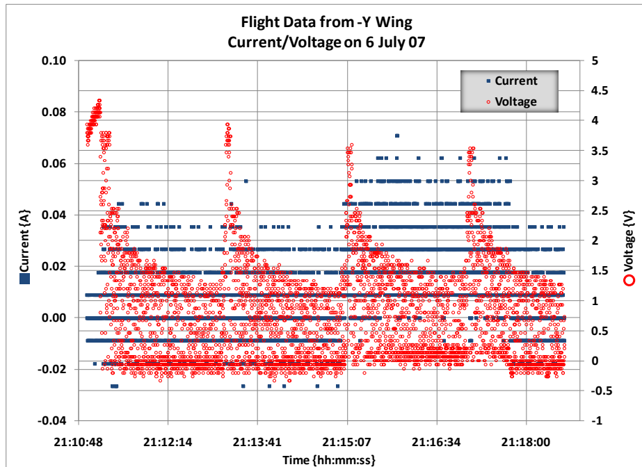
Figure A-13. Flight Data from -Y Wing on 6 July 07 (Current/Voltage)
