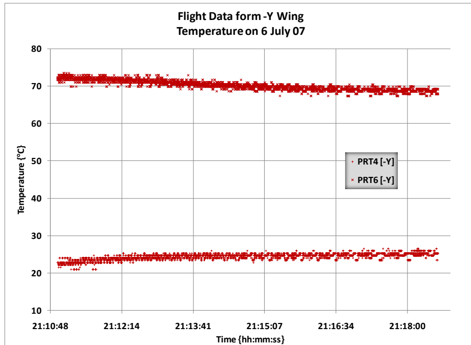
Figure A-14. Flight Data from -Y Wing on 6 July 07 (Temperature)
