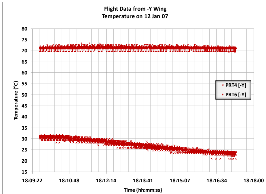
Figure A-6. Flight Data from -Y Wing on 12 Jan 07 (Temperature)
