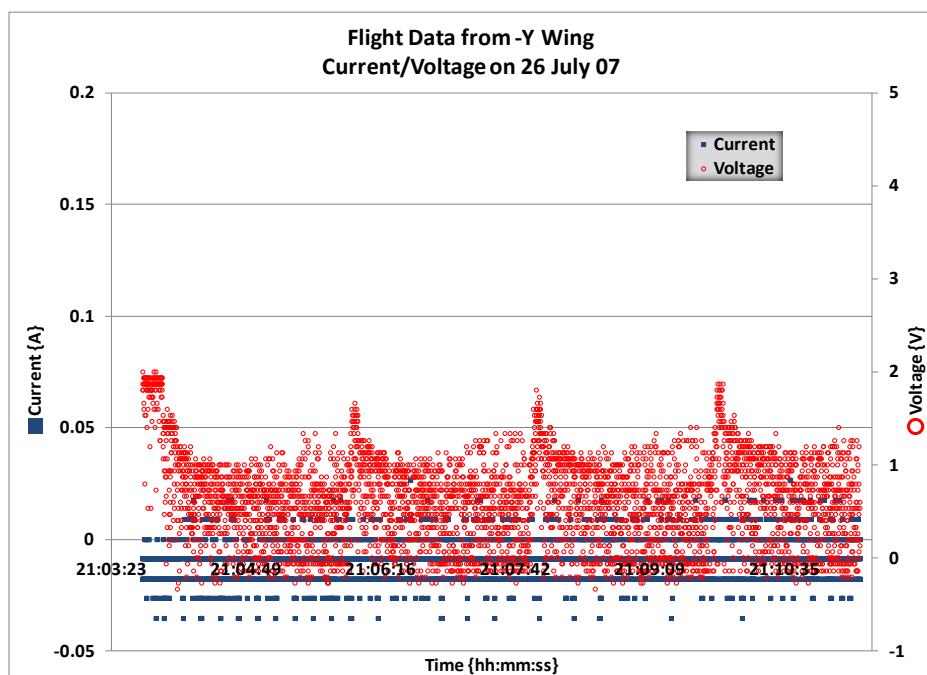
Figure A-15. Flight Data from -Y Wing on 26 July 07 (Current/Voltage)
