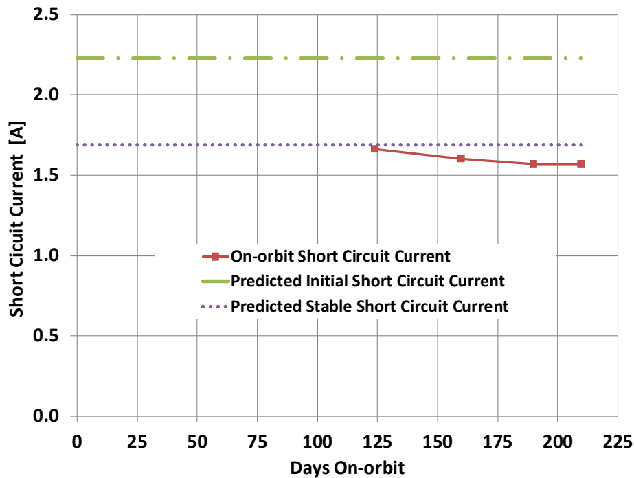
Figure 23. Short Circuit Current as a Function of Days on Orbit (All Corrected to 25 °C)
