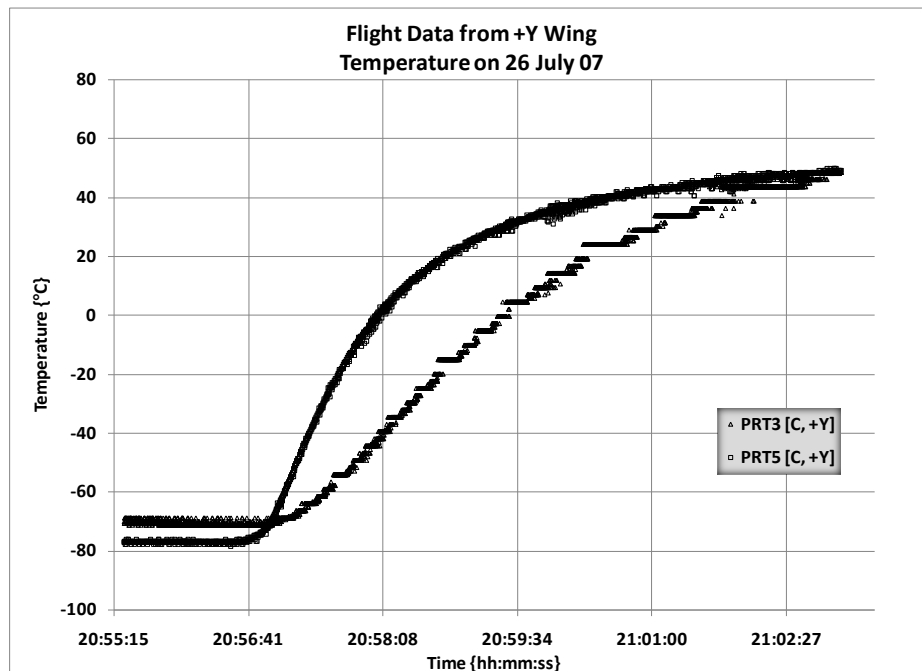
Figure 19. Flight Data from +Y Wing on 26 July 07 (Temperature)
