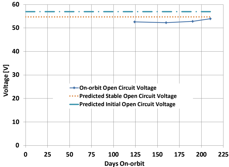
Figure 24. Open Circuit Voltage as a Function of Days on Orbit (All Corrected to 25 °C)
