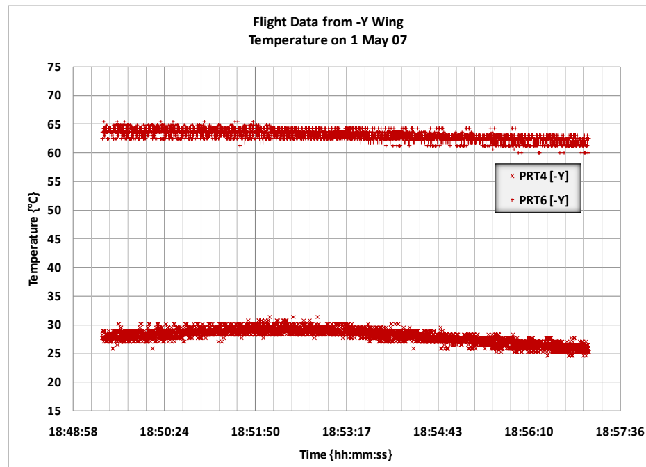
Figure A-10. Flight Data from -Y Wing on 1 May 07 (Temperature)
