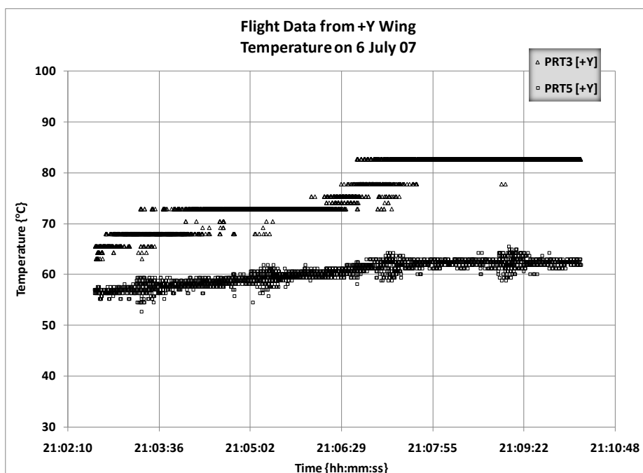
Figure 17. Flight Data from +Y Wing on 6 July 07 (Temperature)
