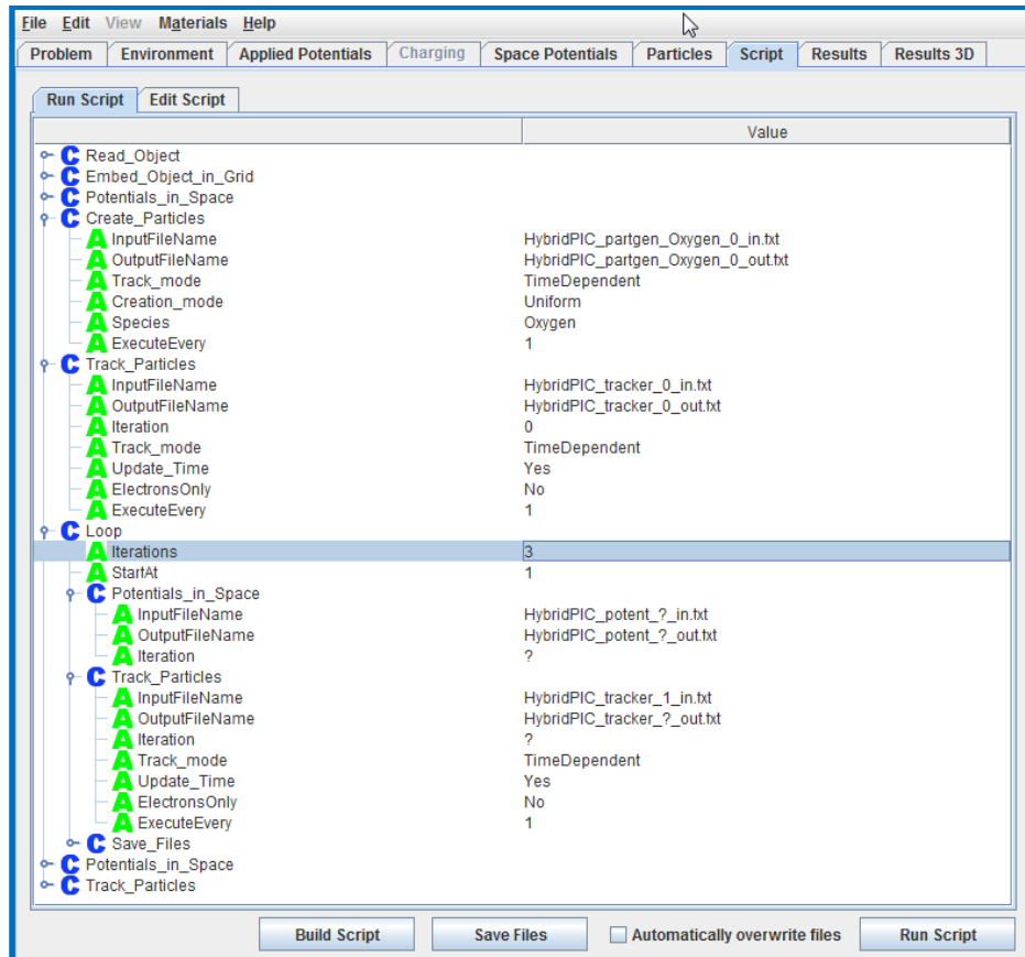
Figure 136. Script for the “Dynamic” Example Showing Four Iterations
