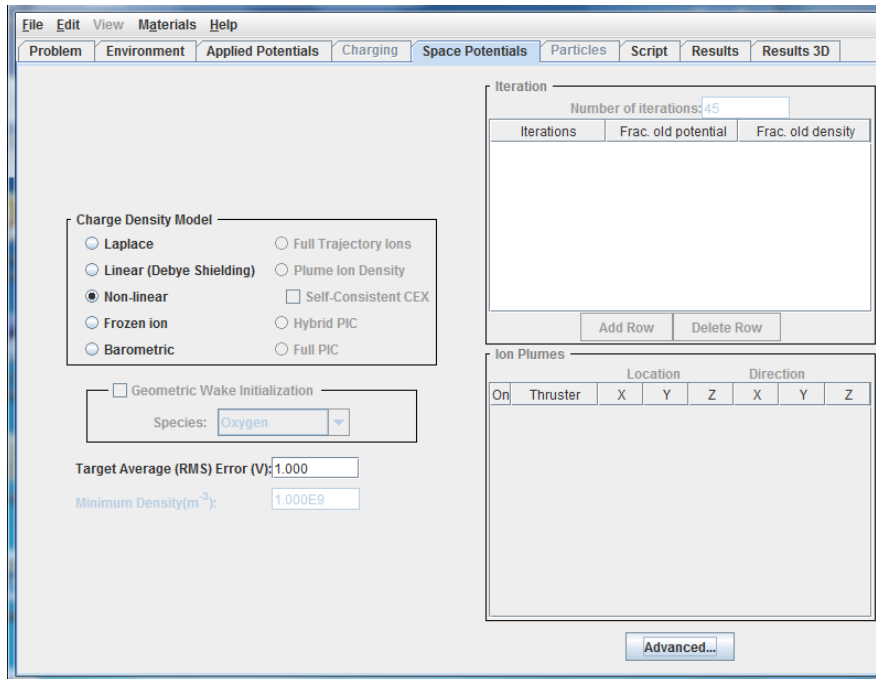
Figure 73. Space Potentials Tab for the “Bipolar” Example
