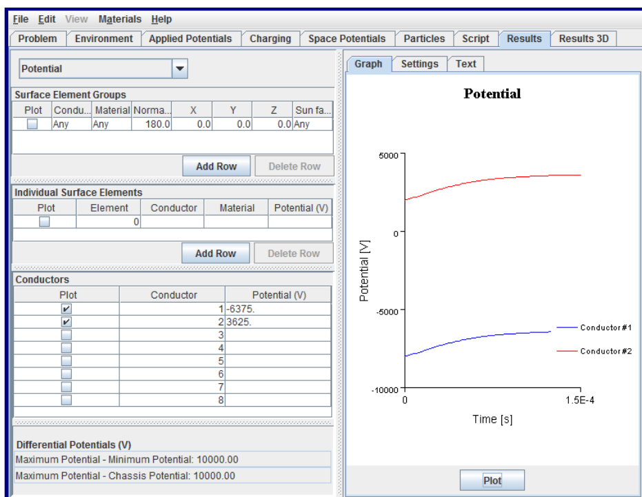
Figure 92. Results Tab Showing Evolution of Conductor Potentials Toward Current Balance for Case 3 of the “Bipolar” Example
