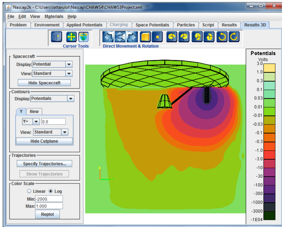
Figure 124. Potential Distribution in the WSF Wake for Case 4 of the “CHAWS” Example
