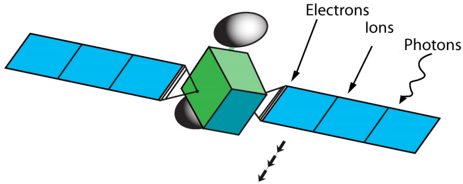
Figure 18. High Negative Potentials Can Result from the Accumulation of Charge on Spacecraft Surfaces
