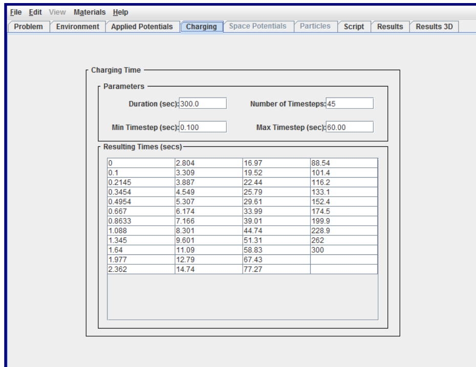
Figure 51. Charging Tab for the “GeoCharging” Example
