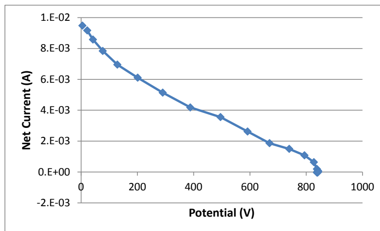
Figure 159. Net Current versus Potential for the Emitter Problem.
