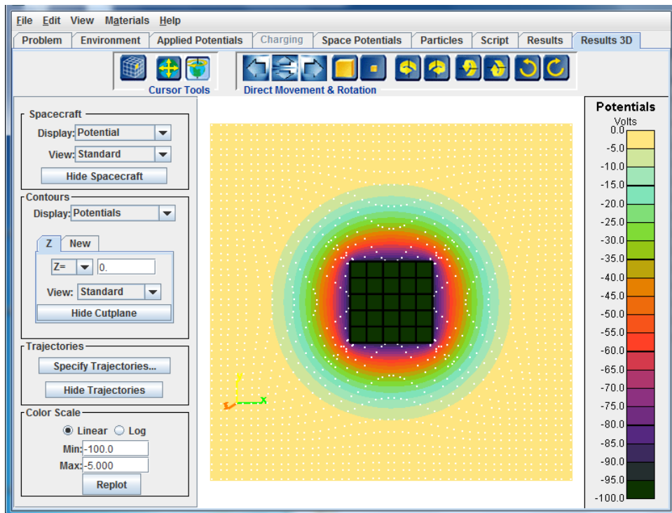
Figure 141. Particle Distribution for Case 3 of the “Dynamic” Example at t=10 \mu s
