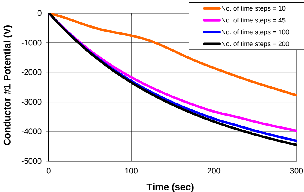
Figure 58. Sensitivity of Results on Choice of Number of Timesteps in the Charging Calculation of Case 1 of the “GeoCharging” Example
