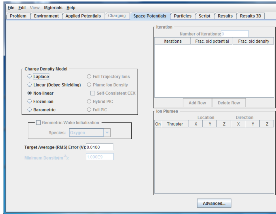
Figure 101. Space Potentials Tab for Case 1 of the “CHAWS” Example
