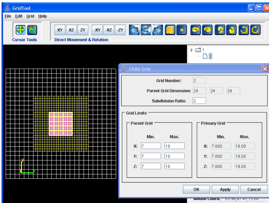
Figure 127. Grid Definition for the “Dynamic” Example. Top: Primary Grid Definition. Bottom: Child Grid Definition
