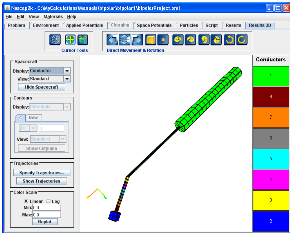
Figure 63. Object Constructed for the Study of Current Collection from a Bipolar Sheath in a Low-Earth-Orbit Environment. Top: Object Materials. Bottom: Object Conductors
