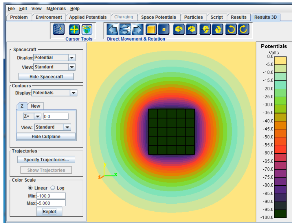
Figure 143. Steady-state Potential Profile for Comparison with Transient Results for the “Dynamic” Example
