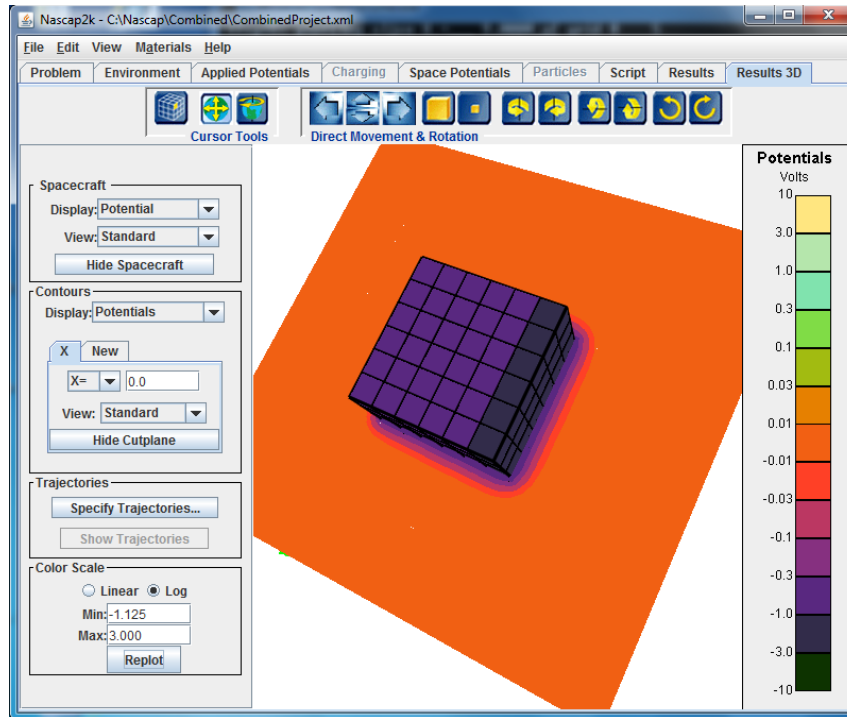
Figure 193. Expanded View of “Lower” part of Figure 192, Showing that the Potentials Have Been Correctly Calculated and Plotted
