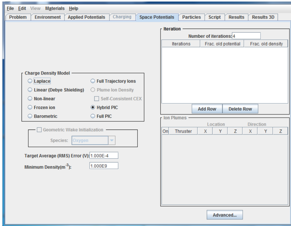
Figure 134. Space Potentials Tab Depicting “Hybrid PIC” Choice for Case 3 of the “Dynamic” Example
