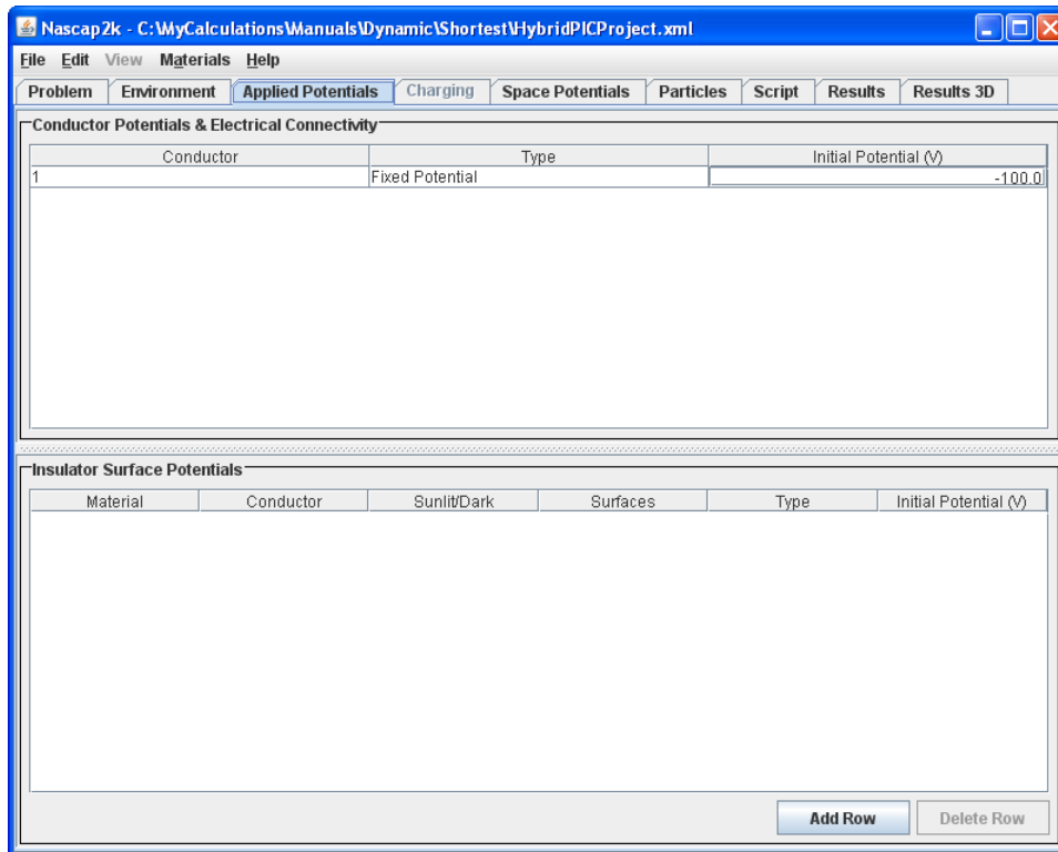
Figure 129. Applied Potentials Tab for the “Dynamic” Example
