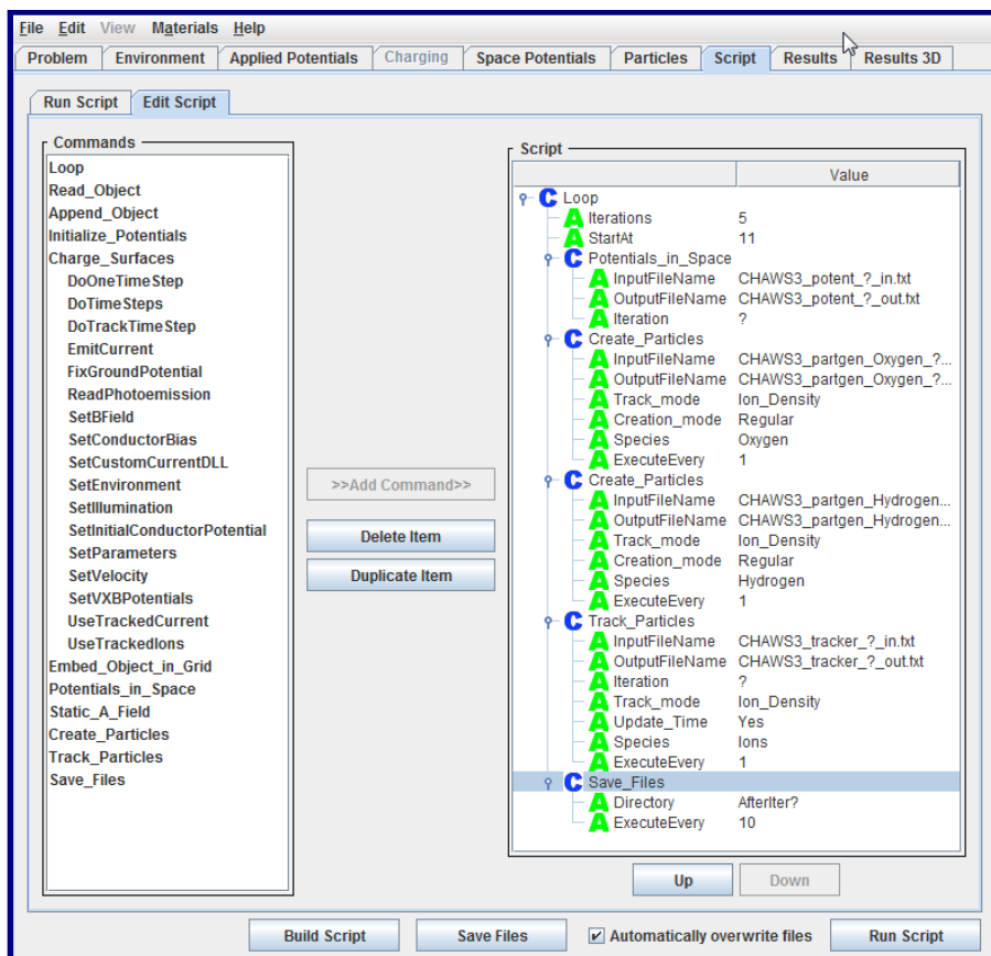
Figure 123. Script Used in Case 4 of the “CHAWS” Example
