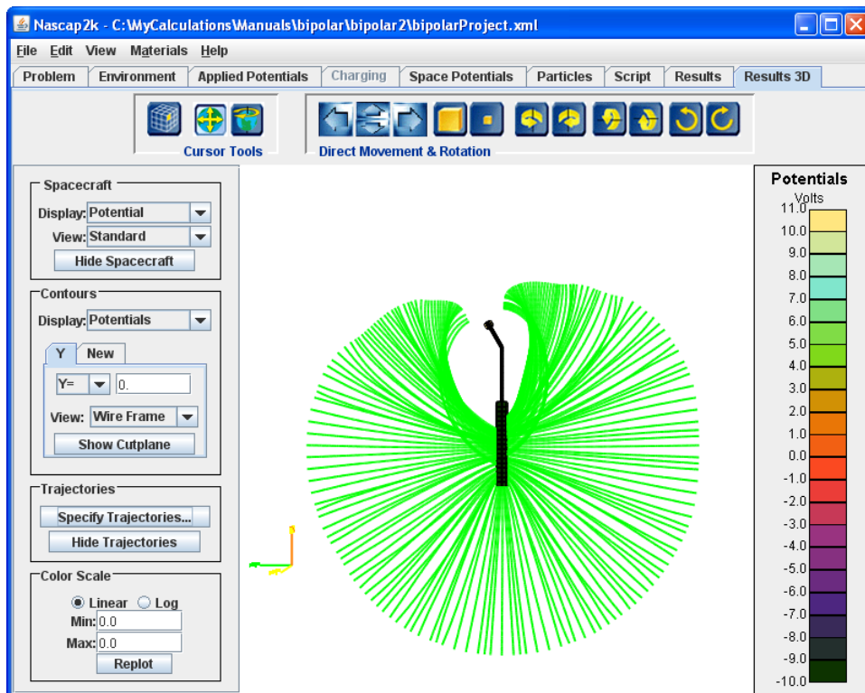
Figure 86. Oxygen Ion Trajectories for Case 2 of the “Bipolar” Example
