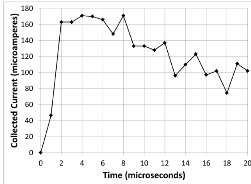
Figure 142. Ion Collection (Current) by Gold-plated Cube as a Function of Time for Case 3 of the “Dynamic” Example
