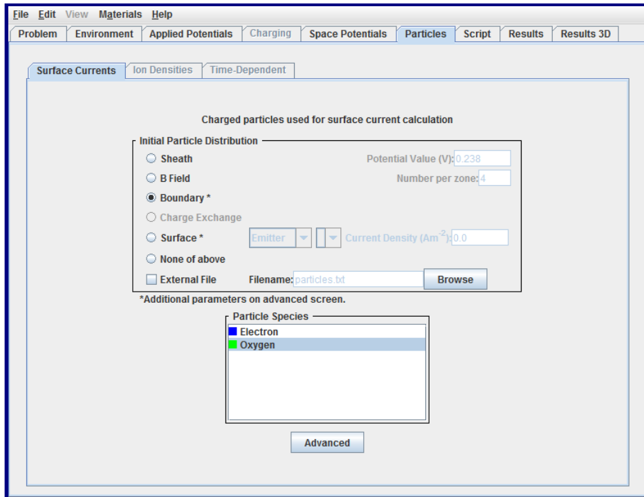
Figure 108. Surface Currents Subtab for Case 2 of the “CHAWS” Example
