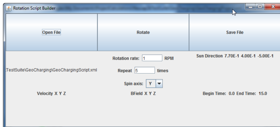
Figure 178. Rotator Script Building Tool Specifying that a Rotation Rate of 1 Rotation per Minute about the Y-axis is to be Applied to the Script in the File GeoChargingScript.xml for five Repeats of the Time Period Specified in the DoTimeSteps Subcommand
