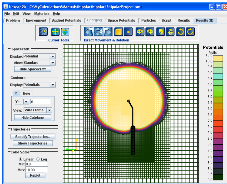
Figure 80. Potential Distribution Showing Sheath Edge on Mesh for Case 1 of the “Bipolar” Example
