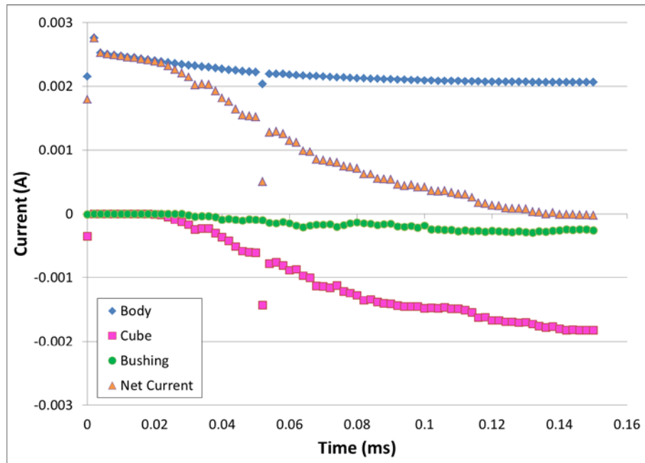
Figure 93. Current Collection by Conductors as a Function of Time for Case 3 of the “Bipolar” Example
