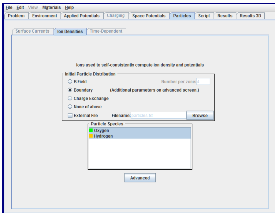
Figure 122. Ion Densities Subtab for Case 4 of the “CHAWS” Example
