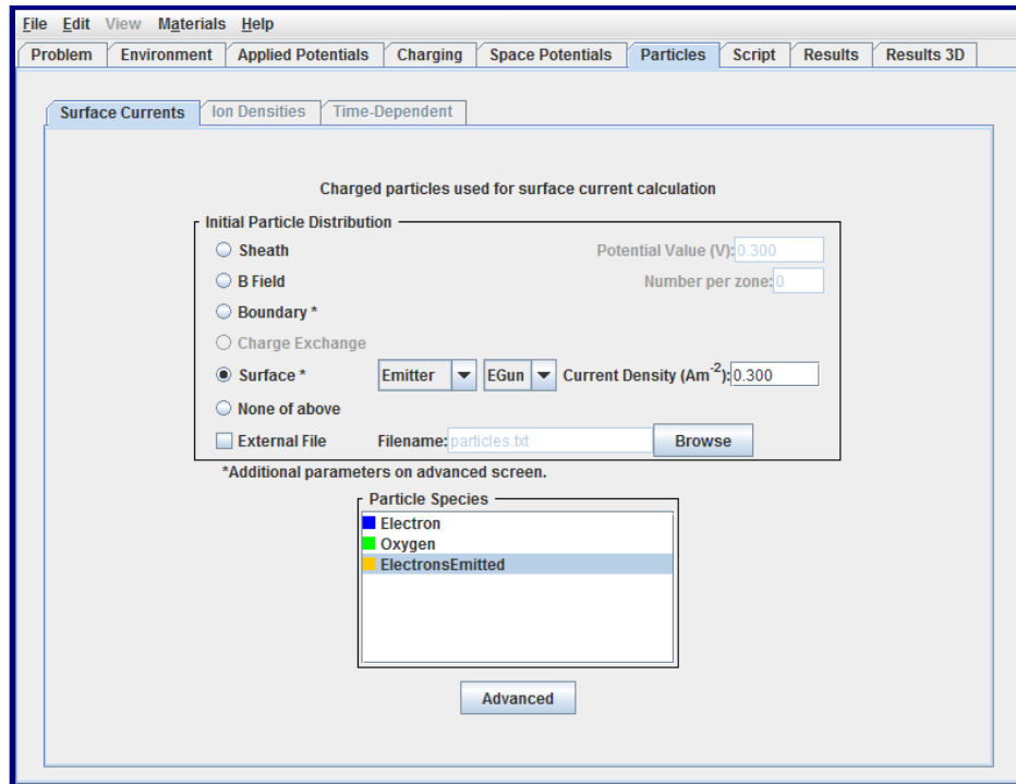
Figure 154. Particles Tab Specification for Emitter Electrons.
