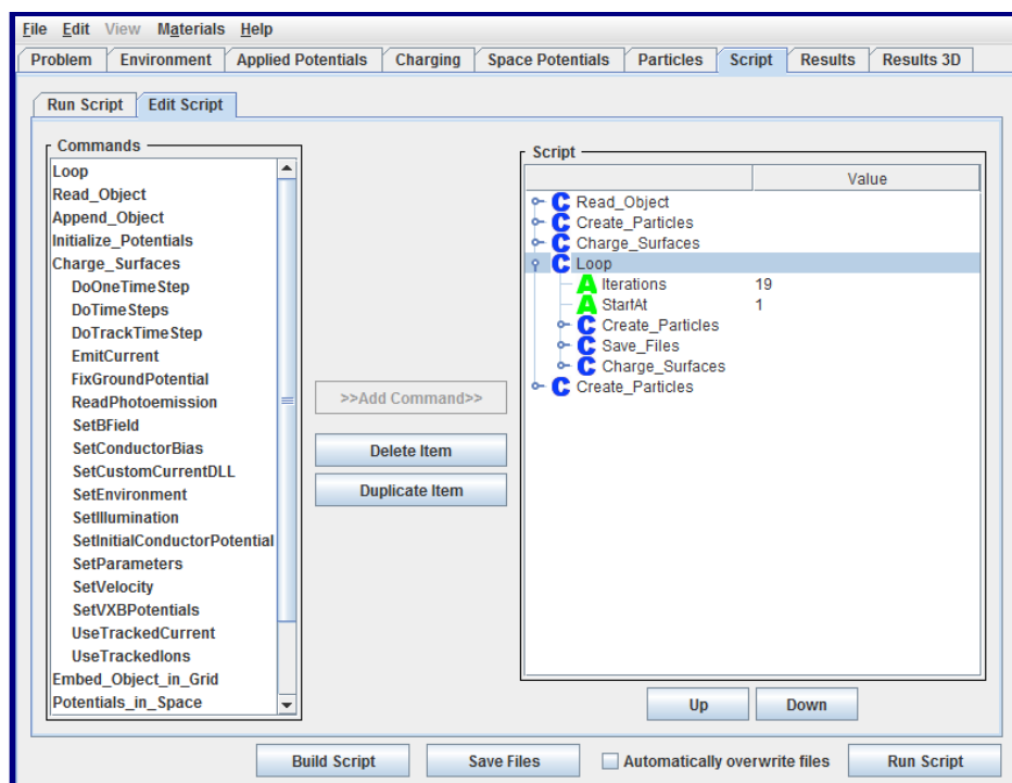
Figure 155. Edited Script Used to Write Input Files for Creating Macroparticles to Represent those Originating at the Emitter
