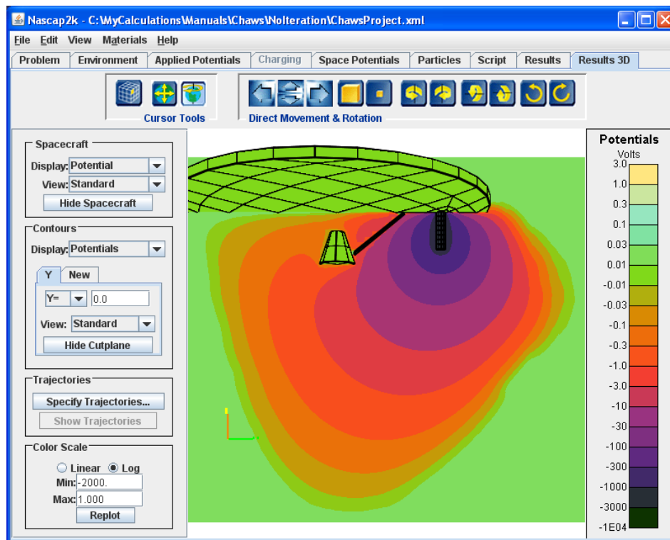
Figure 110. Potential Distribution for Case 2 of the “CHAWS” Example
