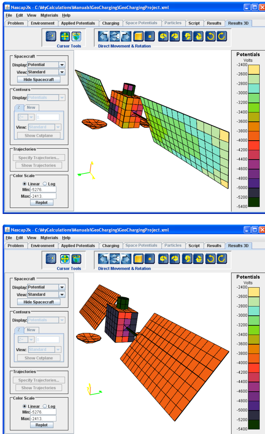
Figure 59. Results 3D Tab for Case 1 of “GeoCharging” Showing Spacecraft Potentials of Sunlit (Top) and Dark (Bottom) Surface Elements
