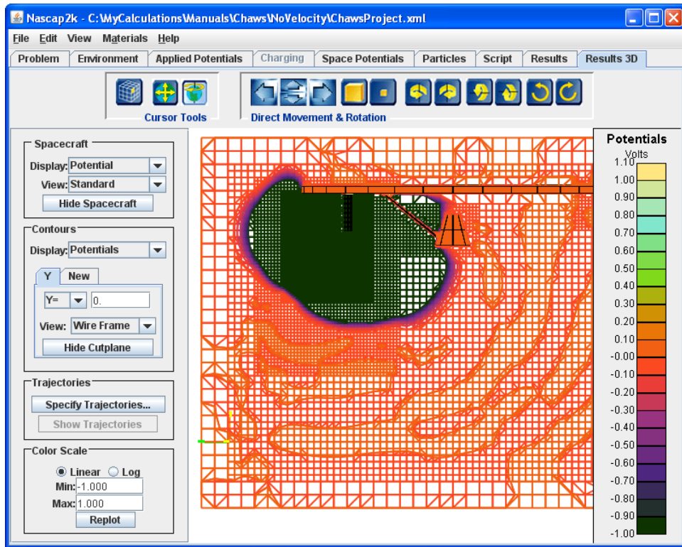
Figure 102. Location of Sheath Edge Potential for Case 1 of the “CHAWS” Example
