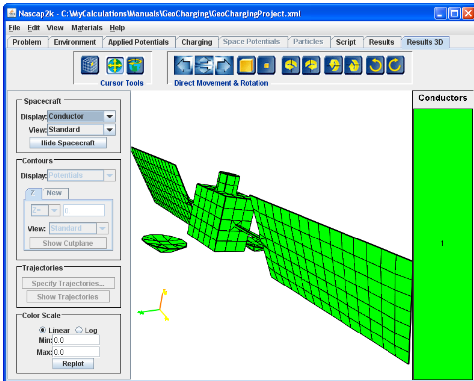
Figure 47. Spacecraft Model Used in the “GeoCharging” Example Showing Material (Top) and Conductor (Bottom) Definition
