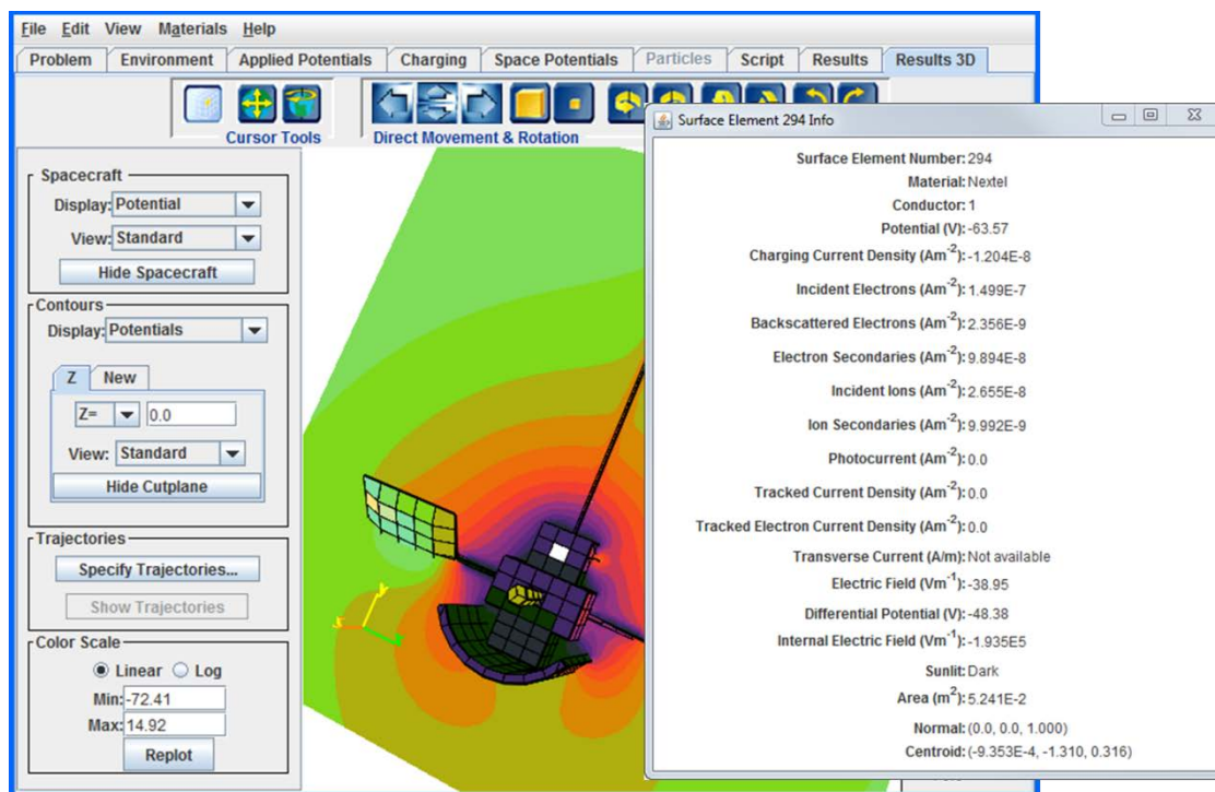
Figure 40. Results 3D tab: Displaying Potentials on a Plane through the Center of the Box, Together with Results for a Selected Surface Element
