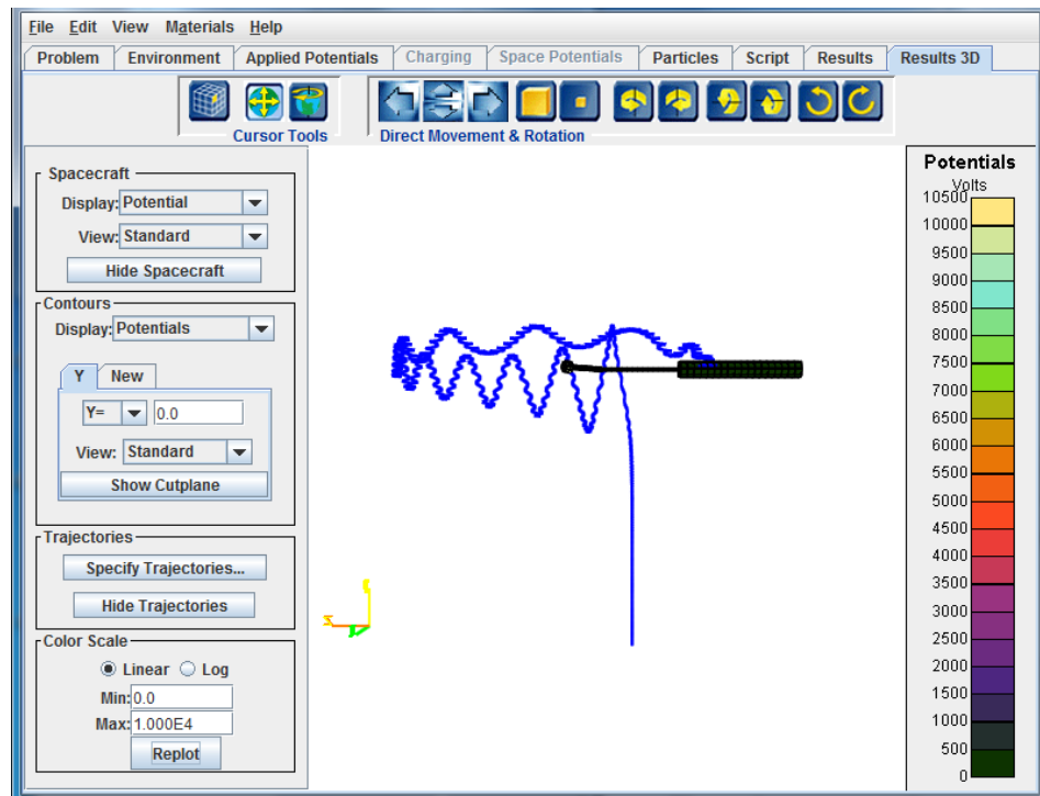
Figure 83. Electron Trajectories Around the Positively Biased Cube when B_x=0 , B_y=0.4 G, B_z=0 for Case 1 of the “Bipolar” Example (Bottom is rotated view of top)
