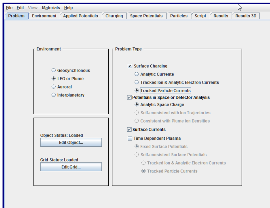
Figure 87. Problem Tab for Case 3 of the “Bipolar” Example
