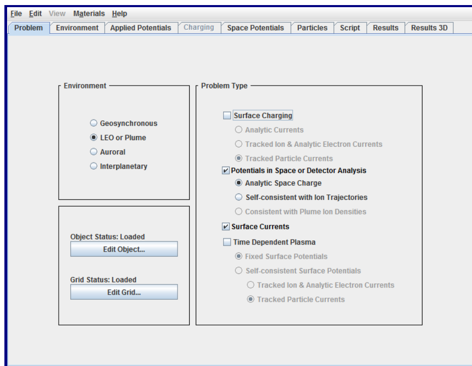
Figure 98. Problem Tab for Case 1 of the “CHAWS” Example
