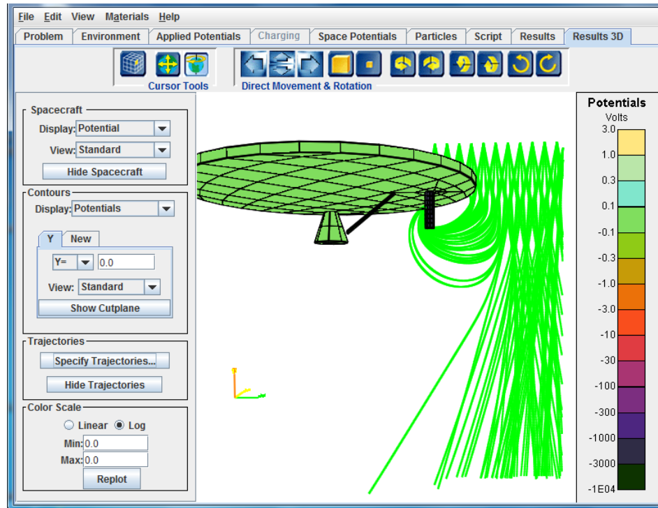
Figure 119. Trajectories for Case 3 of the “CHAWS” Example
