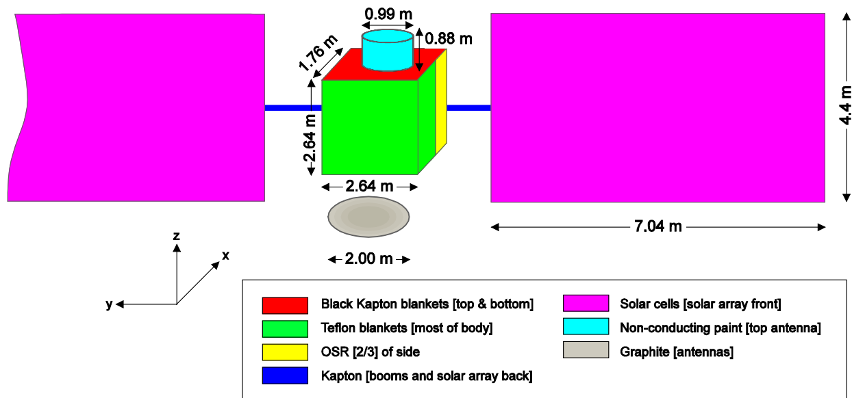
Figure 46. Illustrative Spacecraft for Sample Charging Calculation Using Nascap-2k
