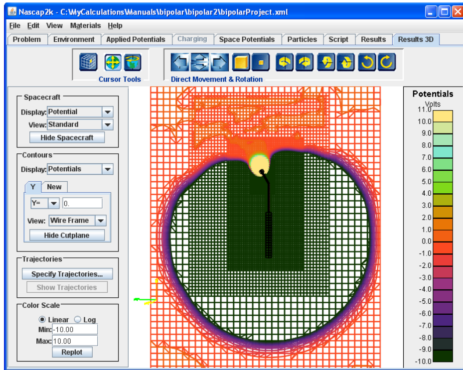
Figure 85. Potential Distribution Showing Ion and Electron Sheath Edges on the Mesh for Case 2 of the “Bipolar” Example
