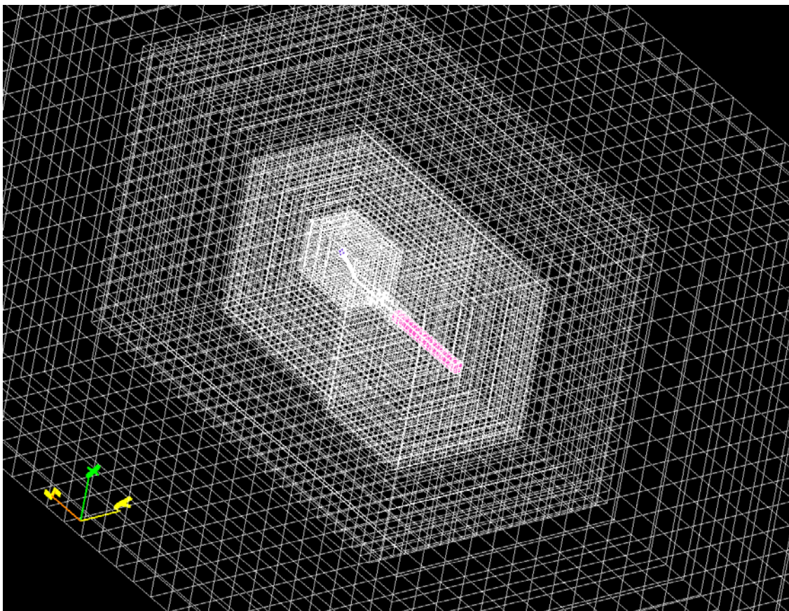
Figure 69. Grid Arrangement Showing All Six Grid Levels and Embedded Object for the “Bipolar” Example
