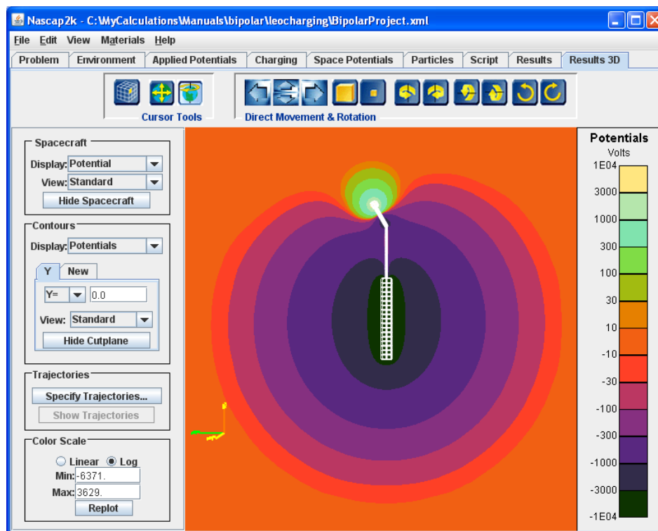
Figure 94. Potential Distribution at Equilibrium (~Zero Net Current) in the “Bipolar” Example
