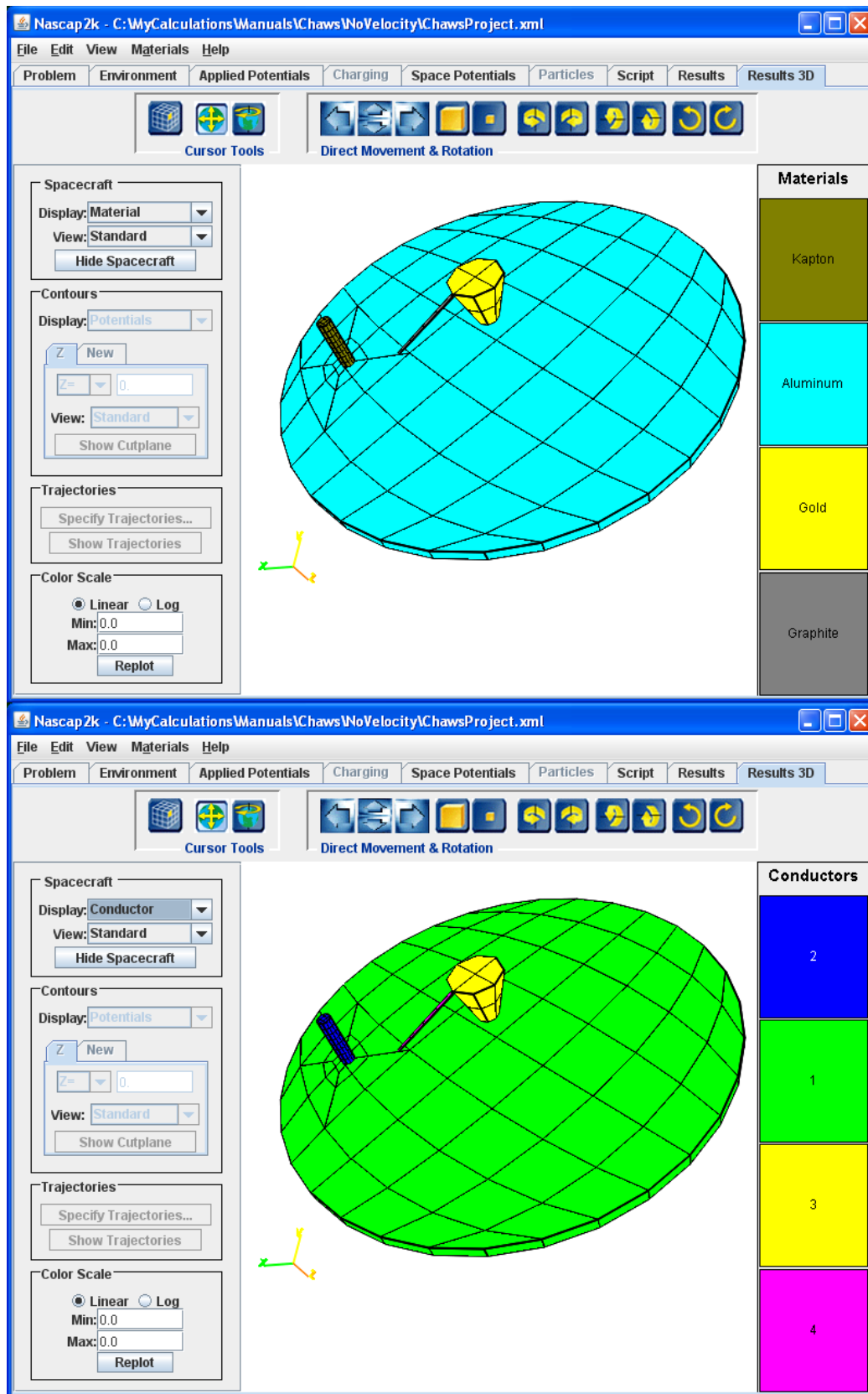
Figure 96. WSF Object. Top: Materials; Bottom: Conductors
