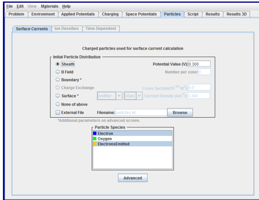
Figure 156. Particles Tab Specification for Sheath Electrons
