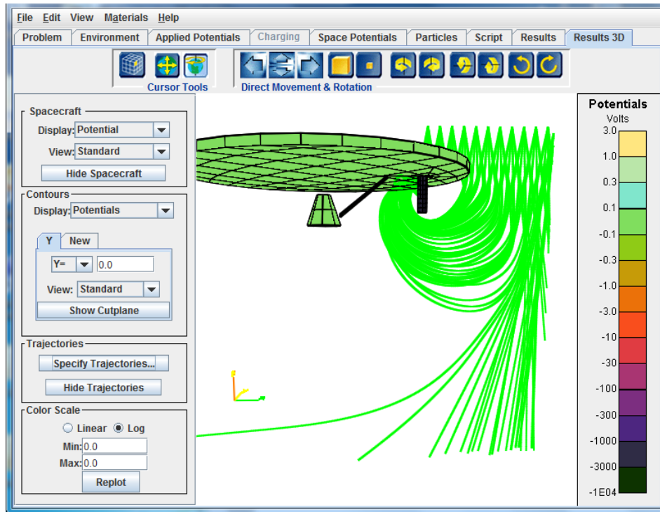
Figure 111. Ion Trajectories for Case 2 of the “CHAWS” Example
