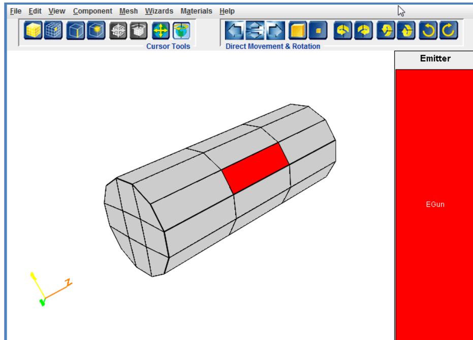
Figure 151. Aluminum Cylinder Showing Emitter Surface Element
