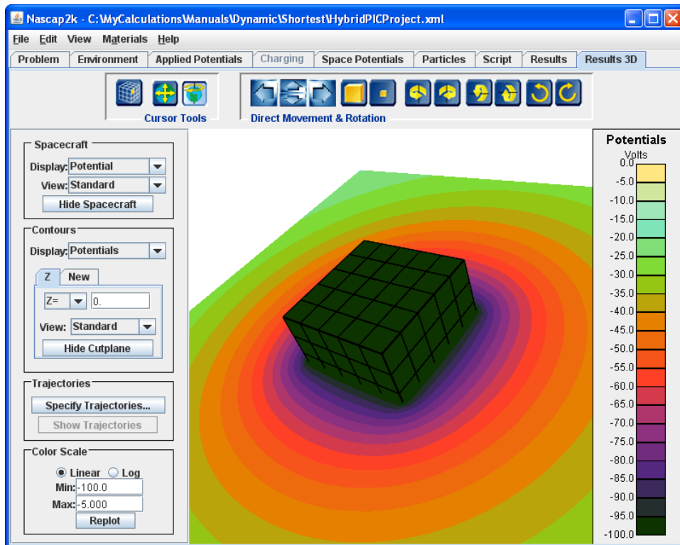
Figure 131. Results 3D Tab Showing Laplacian Space Potential Distribution
