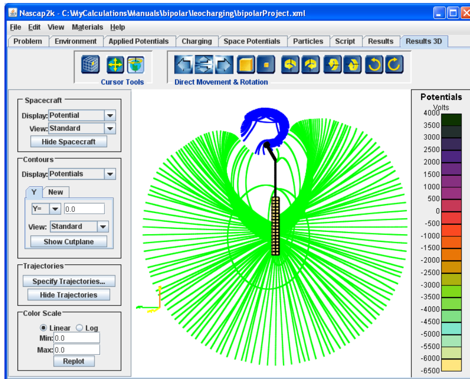
Figure 95. Selected Ion and Electron Trajectories at Equilibrium in the “Bipolar” Example
