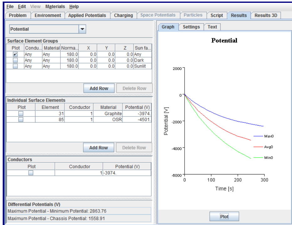
Figure 37. Results Tab: Plotting Minimum, Maximum, and Average Values of Elements with Specified Conductors and/or Materials
