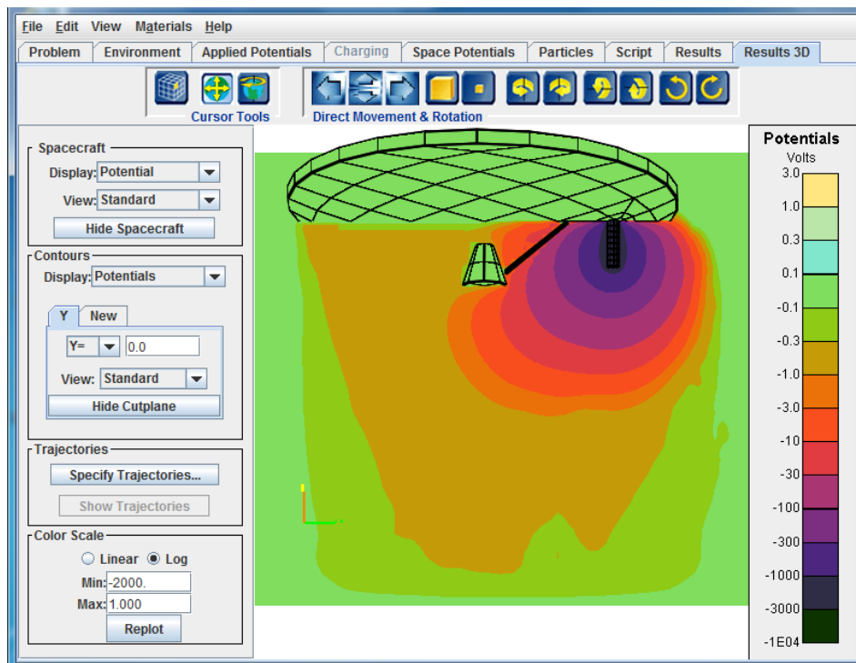
Figure 118. Potential in the Wake of WSF for Case 3 of the “CHAWS” Example
