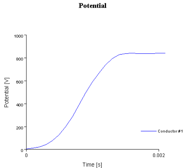
Figure 158. Potential versus Time for the Emitter Example.
