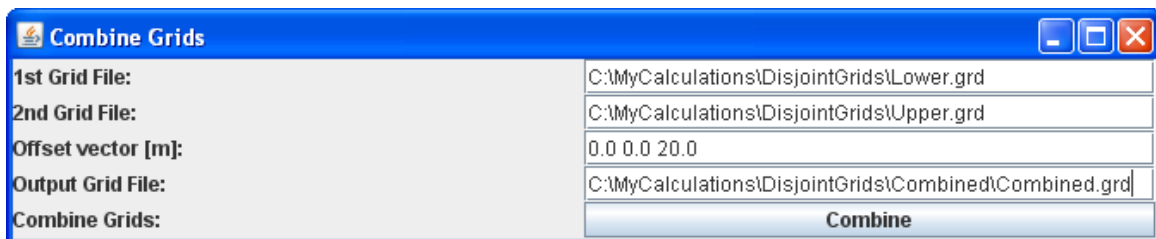
Figure 186. The CombineGrids User Interface
