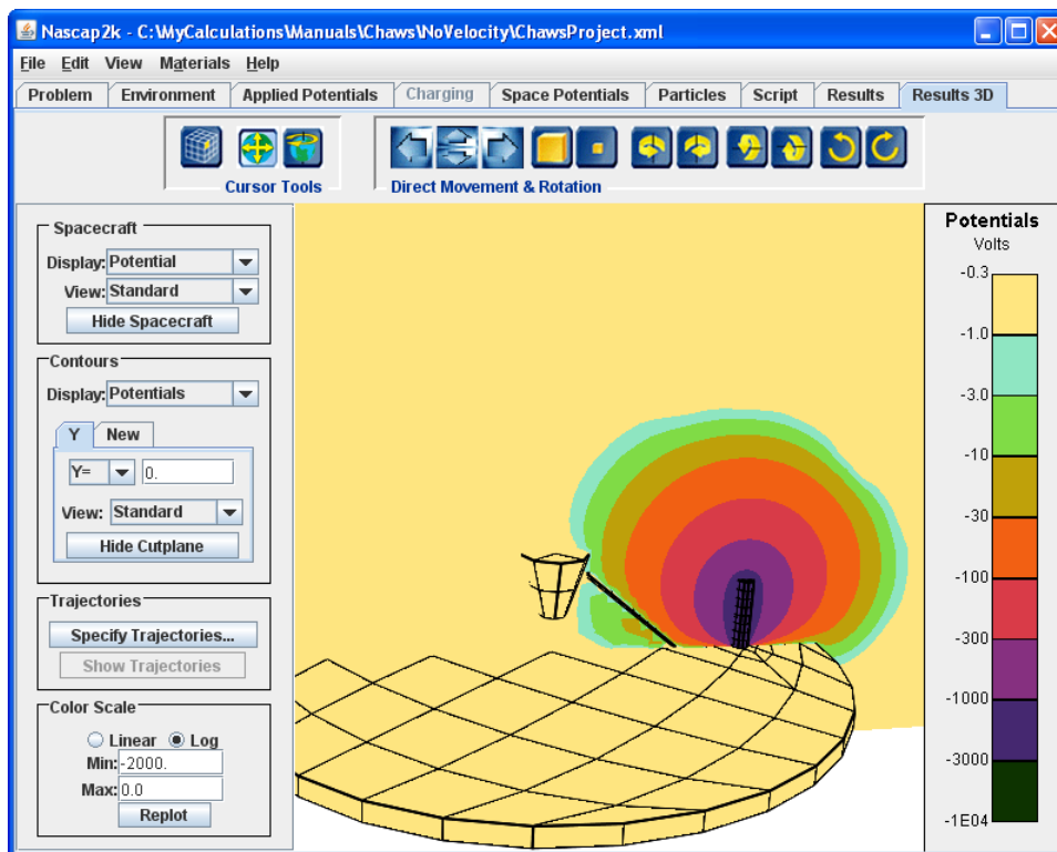
Figure 105. Potential Profile for Case 1 of the “CHAWS” Example
