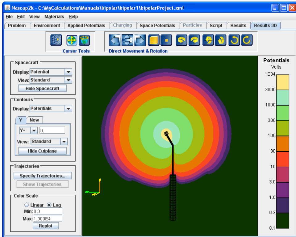
Figure 76. Distribution of the Electric Potential on a Y=0 Cut Plane for Case 1 of the “Bipolar” Example
