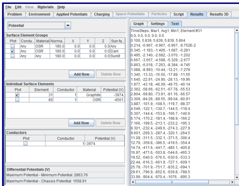
Figure 39. Text Output in the Results Tab
