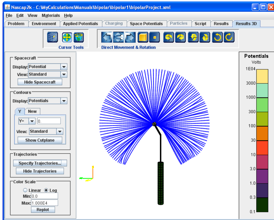
Figure 78. Electron Trajectories for Case 1 of the “Bipolar” Example
