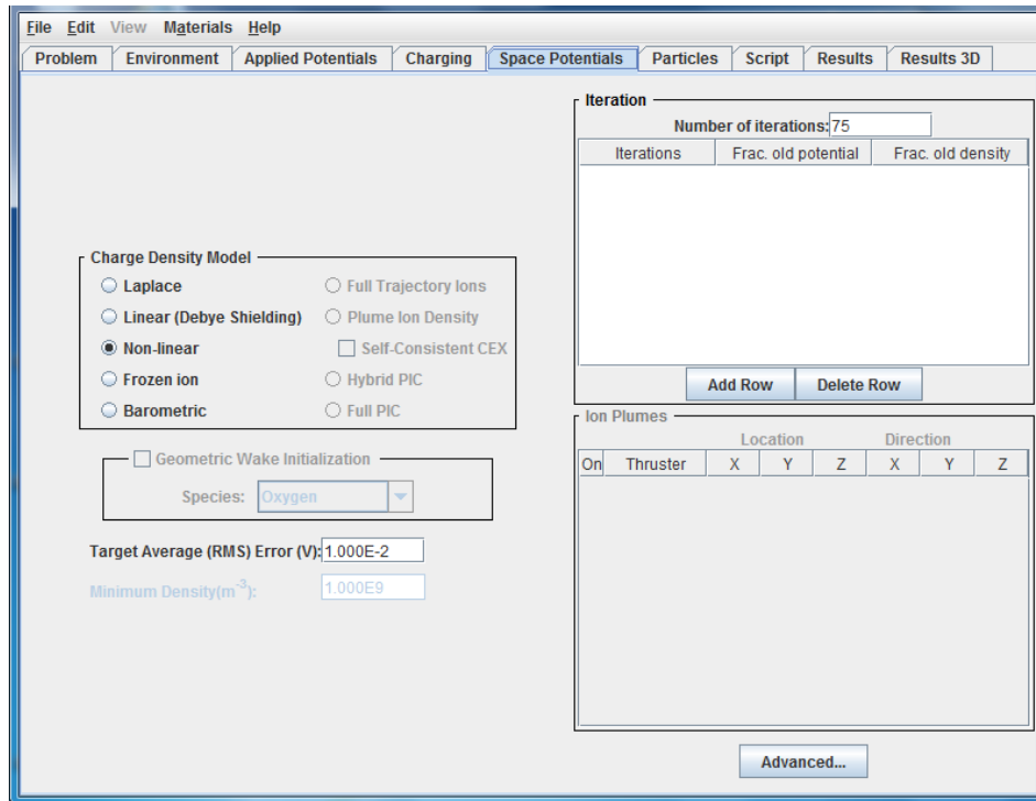
Figure 90. Space Potentials Tab Showing Number of Iterations for Case 3 of the “Bipolar” Example
