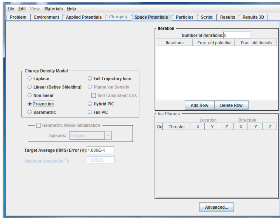
Figure 132. Space Potentials Tab for Case 2 of the “Dynamic” Example
