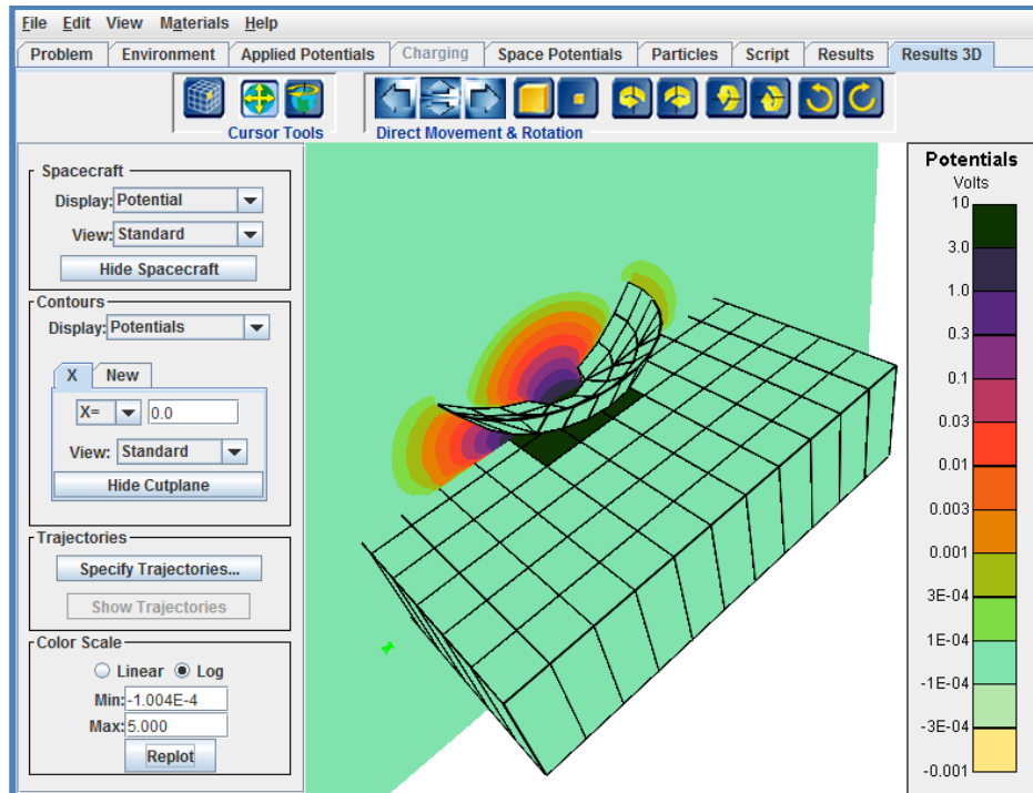
Figure 149. Results3D tab Showing Bowing Out of Potentials Through the Collimator
