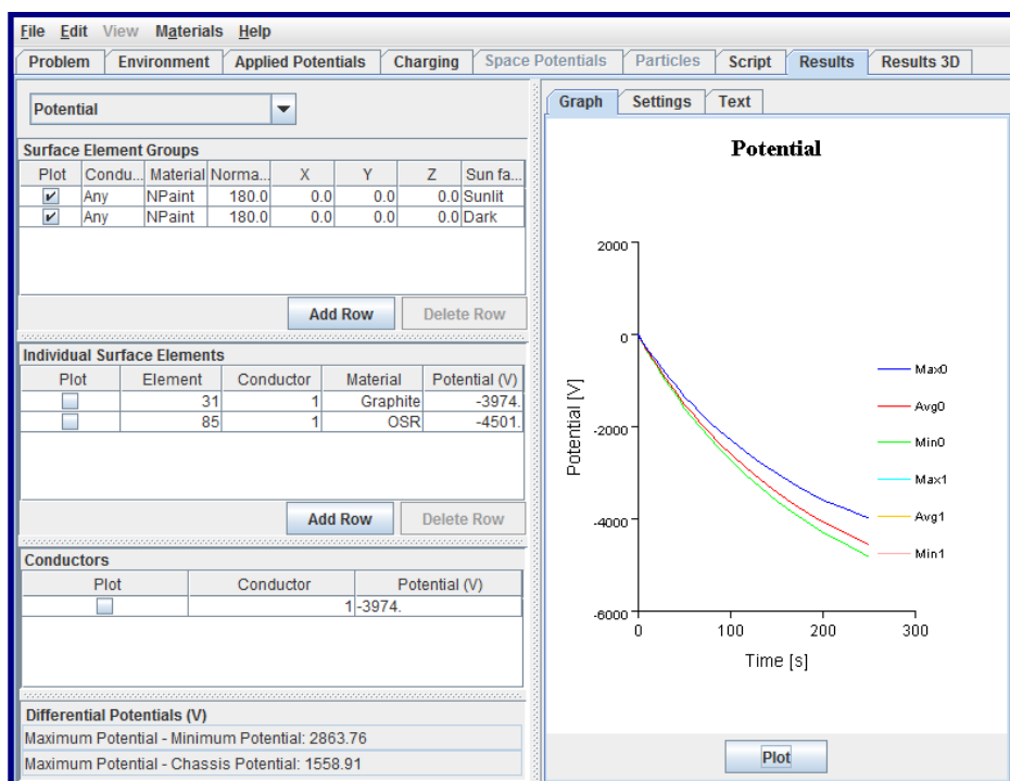
Figure 54. Results Tab for Case 1 of the “GeoCharging” Example Comparing Evolution of Potential Between Sunlit and Dark Surface Elements on the Cylindrical Antenna
