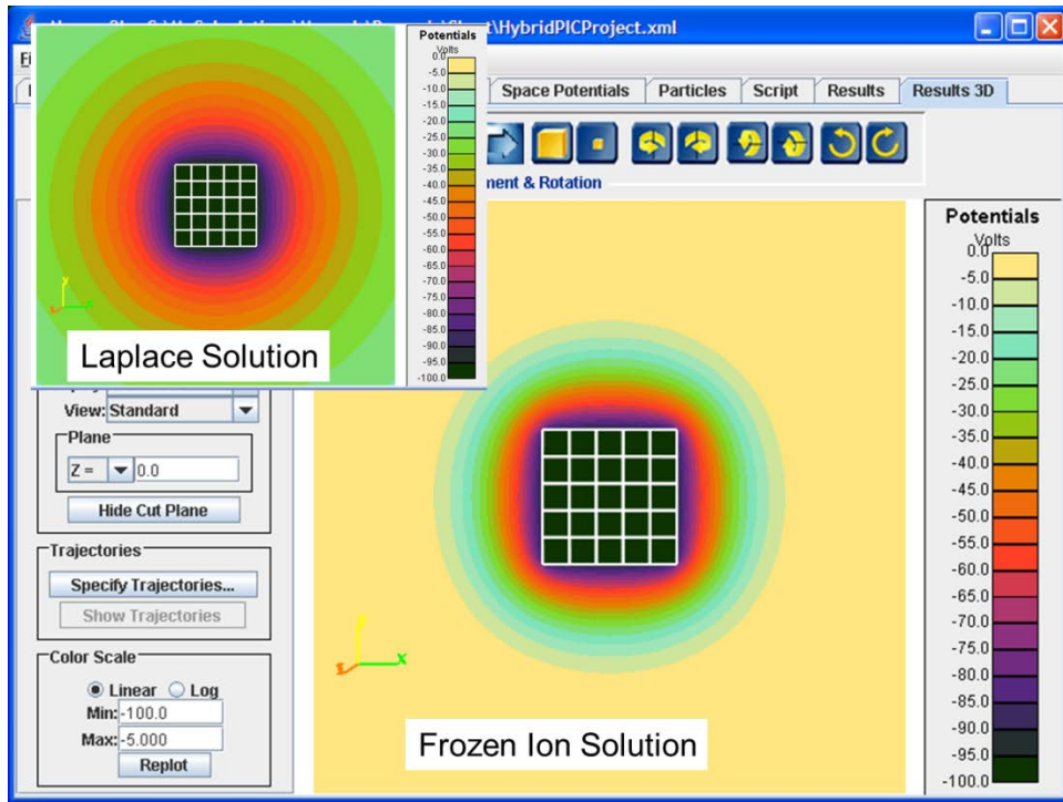
Figure 133. Results from Case 2 of the “Dynamic” Example Compared with Laplacian Solution (Upper Left)
