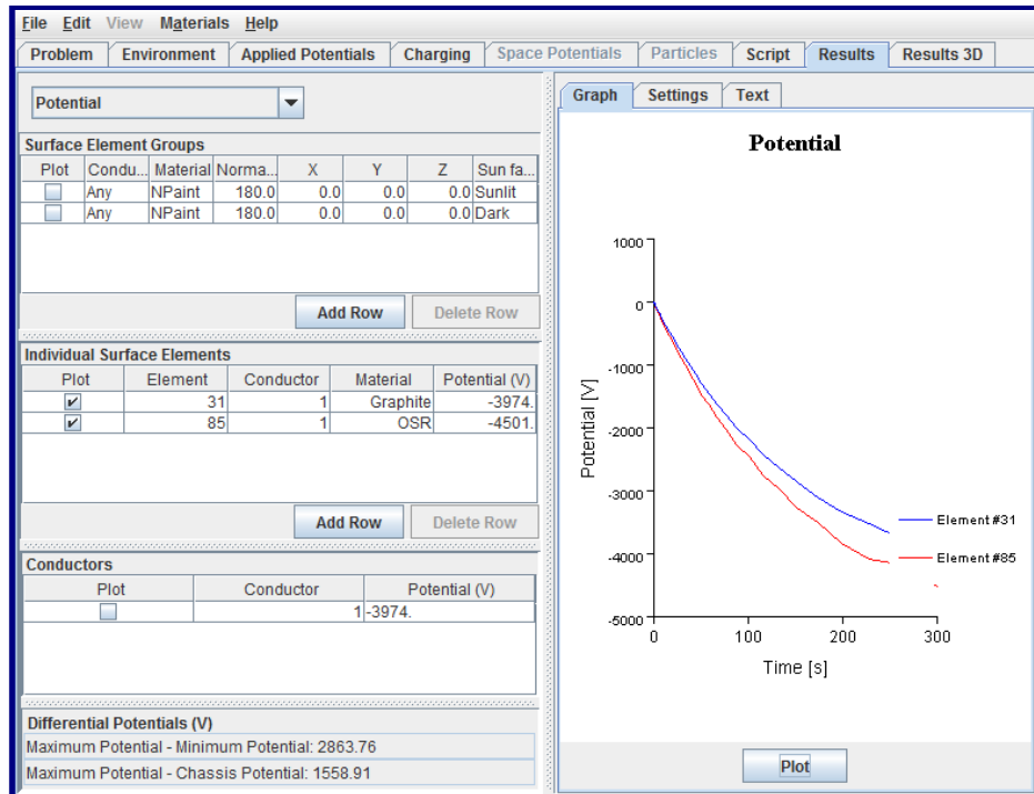
Figure 55. Results Tab for Case 1 of the “GeoCharging” Example Comparing Evolution of Potential for Different Surface Elements
