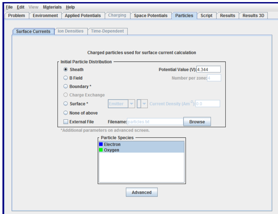
Figure 91. Surface Currents Subtab for Case 3 of the “Bipolar” Example
