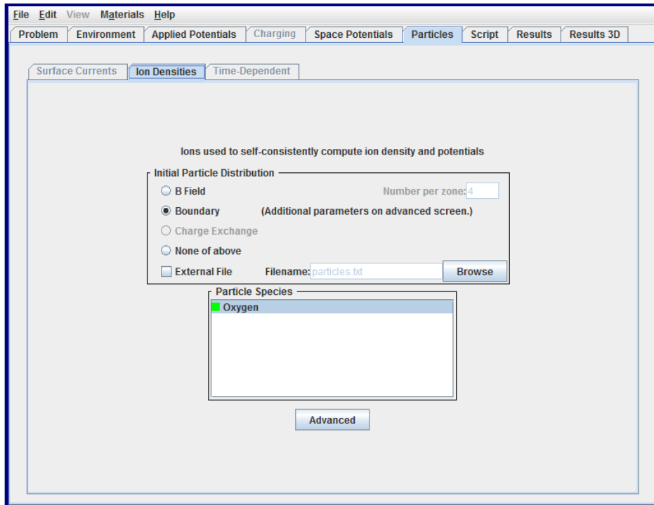
Figure 29. Ion Densities Subtab for Generation and Tracking of Particles for Potentials that are “Self-Consistent with Ion Trajectories”
