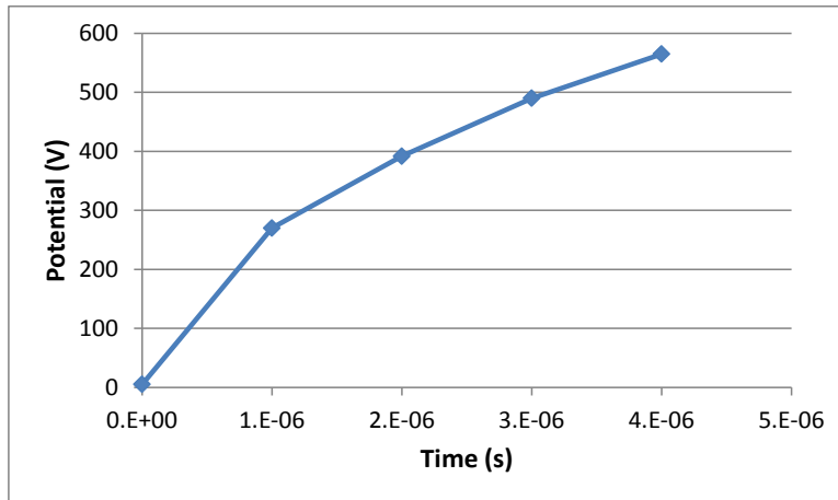
Figure 160. Charging Dynamics with the Stabilizing Current Derivatives Set to Zero.
