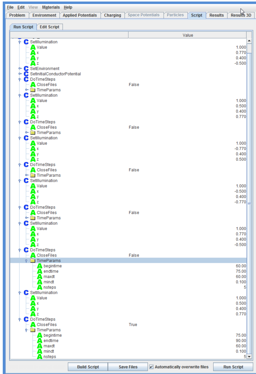
Figure 181. Script Generated by Rotator after Loading into Nascap-2k User Interface
