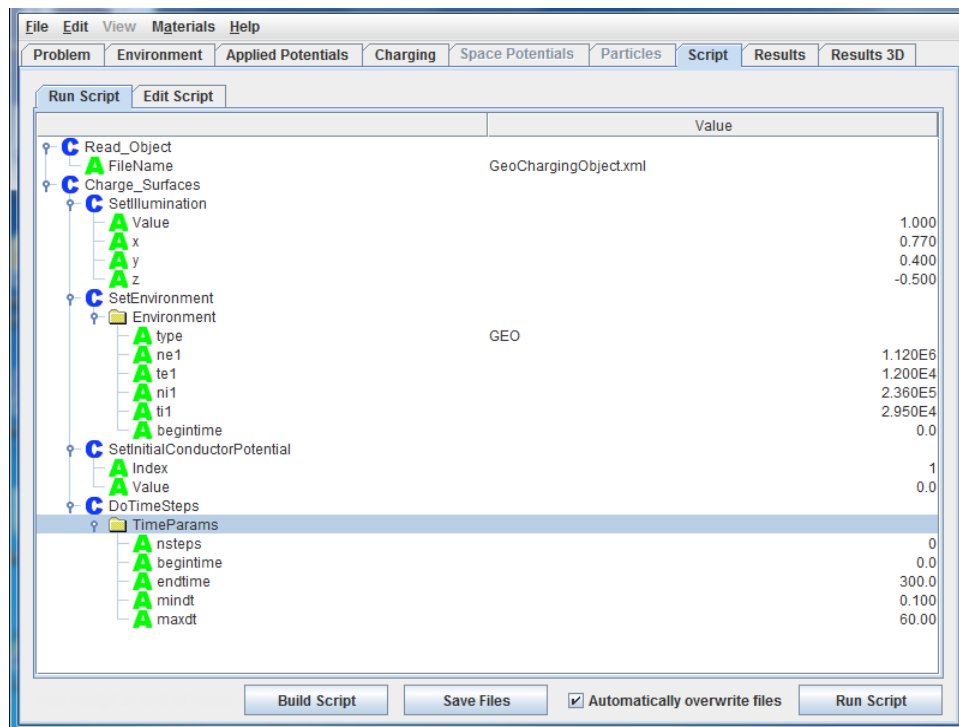
Figure 35. Run Script Subtab for a Typical Geosynchronous Charging Problem with Computation of Potentials about Spacecraft
