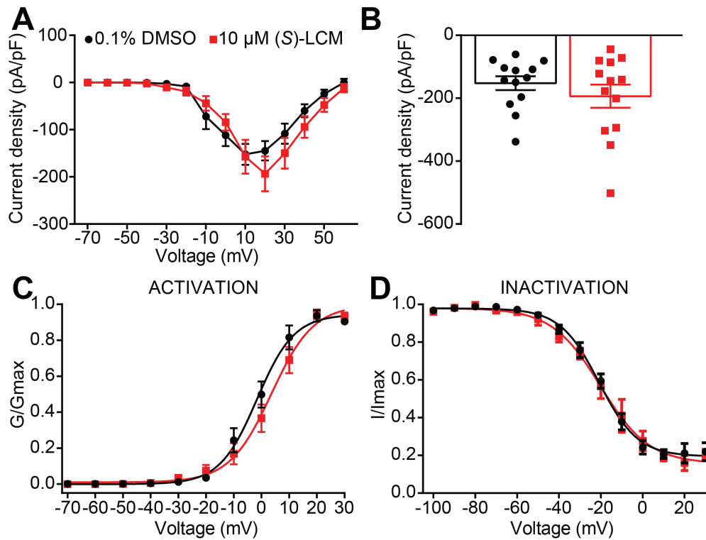
Figure 3: Low concentration of (S)-LCM has no effect on \text{Ca}^{2+} currents in adult rat trigeminal ganglion (TG) neurons. (A) Mean IV curve of current density normalized to the cell capacitance (pA/pF) for each voltage step tested in adult TG neurons treated with 10 \mu\text{M} (S)-LCM or vehicle. (B) Bar graph with scatter plot of peak \text{Ca}^{2+} current density at 10mV in adult TG neurons treated with 10 \mu\text{M} (S)-LCM or vehicle. (C) Activation and (D) inactivation properties of the recorded \text{Ca}^{2+} currents for the indicated conditions in adult TG neurons. In all conditions no difference was found between vehicle and 10 \mu\text{M} (S)-LCM treated cells (Mann-Whitney test). Asterisks indicate statistical significance compared with control cells ( p < 0.05 , 1-way analysis of variance with Dunnett's post hoc analysis).
