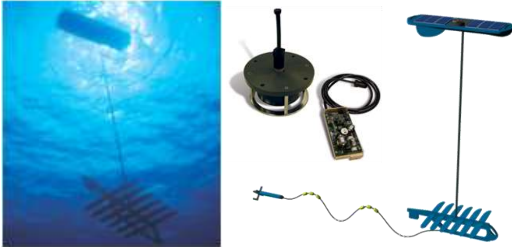
Figure 72. The Wave Glider USV (left) converts vertical sea surface motion into forward thrust. It captures solar energy to power on-board navigation, sensing and communications. Project MISSION has integrated an acoustic modem (electroacoustic transducer and electronics board shown) with a tow body compliantly attached to the lower body of the Wave Glider (right). The resulting “gatekeeper” station-keeping gateway node provides the critical communications interface between the underwater Seaweb network domain and the space-borne Iridium satellite communications domain.
