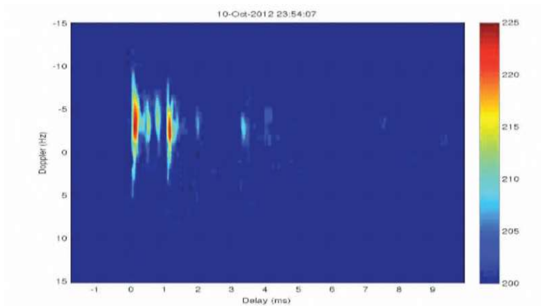
Figure 76. Instantaneous channel response observed at MISSION 2012 is represented by the channel scattering function. The transmitted signal is spread in time by multipath and scattering. The received delay is represented by the x-axis of the channel scattering function. The transmitted signal also experiences Doppler spread, represented by the y-axis, largely imparted by the moving sea surface. This example exhibits 2 dominant multipaths and significant Doppler spread. MISSION data recorded in Singapore Strait exhibit time-varying channel scattering functions that impair communications in terms of energy spread and inter-symbol interference. The underwater acoustic channel must be well understood in the design of channel-tolerant or channel-adaptive modulation.
