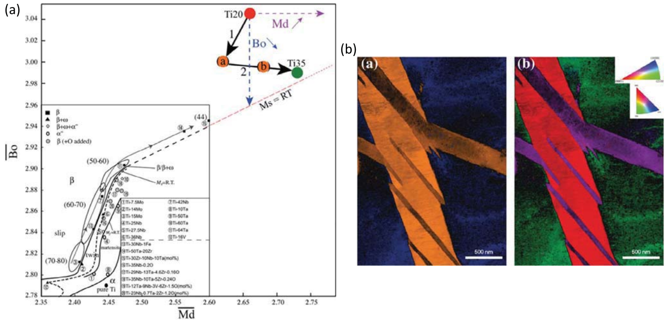
Fig. 5. (a) Bo-Md map used for conventional Ti-based alloys (bottom left) extrapolated to concentrated alloys (top right) [89]. The dashed line corresponds to the formation of martensite (Ms) from the bcc \beta phase. Starting from the equimolar HfNbTaTiZr composition, the coupled reduction of Ta and Nb contents and the increase of Hf, Nb and Ti ones lead to the definition of a non-equiatomic HfNbTaTiZr composition close to the martensite appearance zone; (b) Presence of stress induced \alpha' (hcp) martensite in the initial \beta (bcc) phase after deformation. Phase mapping (left; bcc: blue; hexagonal: orange) and orientation mapping (right) (from [86]).
