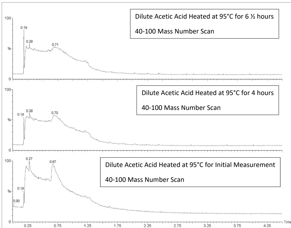
Figure 23: Dilute Acetic Acid Solutions Heated to 95°C for 6 ½ hrs (top), 4 hrs (middle), and the Initial Measurement (bottom) Chromatograms.
