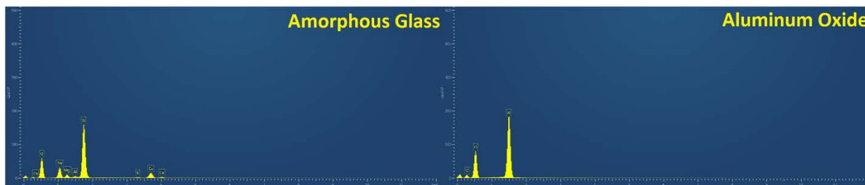
Figure 69: EDS Scan Results from Glass/Ceramic Substrate Materials
