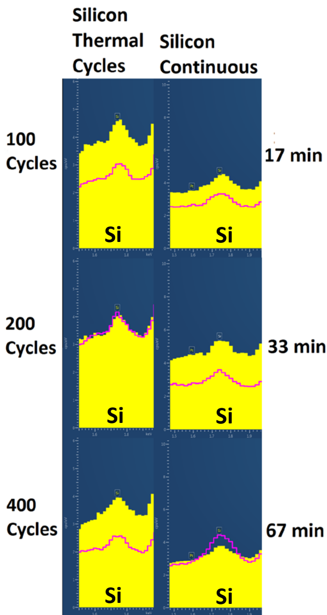
Figure 60: EDS Data for Silicon Peaks Located on the Platinum Sputter Coated PEM Material Samples Applied with a 0.8V Electrical Bias Applied using Cycles (left column) and Applied Continuously (right column). Electrical Bias Cycles were Applied for 100 (top left), 200 (middle left) and 400 (bottom left) Time, while the Continuous Applied Bias was Applied for 17 min (top right), 33 min (middle right) and 67 min (bottom right). All Samples were in Contact with 5 vol% Acetic Acid Solvent at Room Temperature.
