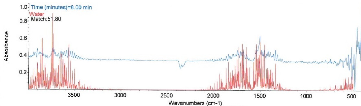
Figure 21: Cell 31 FTIR Scan Raw Data and Database Results at 8.00min (267°C)
