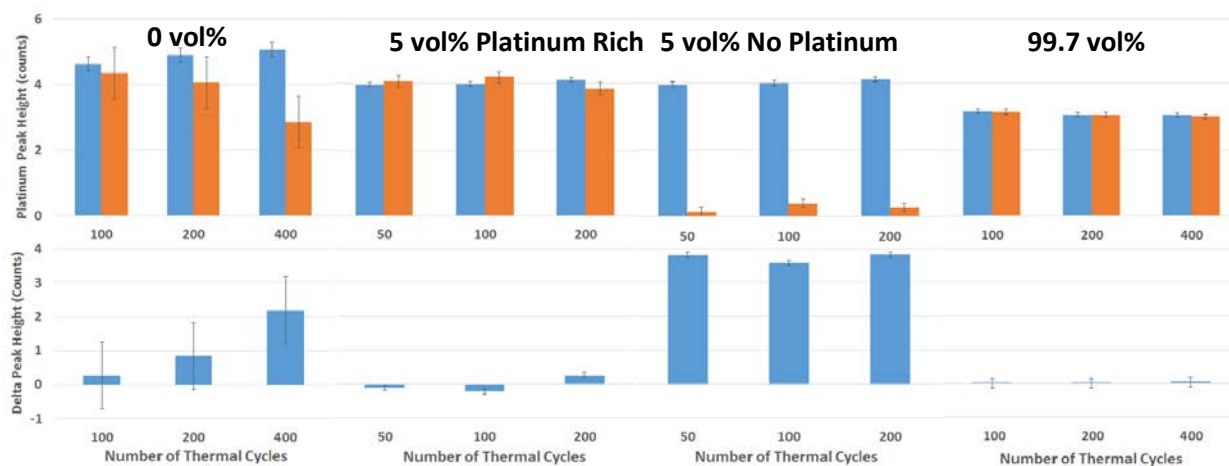
Figure 42: Before Cycling (blue bars, top row) and After Cycling (orange bars, top row) Platinum Peak Comparison for Electrical Bias Effects using 15.5V in 0 vol% Acetic Acid (left column), 5 vol% Acetic Acid Platinum Rich (2 nd from left column), 5 vol% Acetic Acid no Platinum (2 nd from right column) and 99.7 vol% Acetic Acid (right column) which was Extracted from Figure 36, Figure 38 and Figure 40, Respectively. Bottom Row Shows Delta Values between Before and After.
