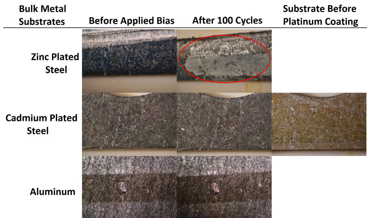
Figure 63: Optical Microscopy Images of Platinum Sputter Coated onto Various Bulk Metal Substrate Materials. Images of the Platinum Coating are Shown Before (left column) and After (middle column) the Electrical Bias was Applied. Images of Substrate Materials before the Platinum Sputter Coating was Applied are Shown in the Right Column. Materials used were: Zinc Plated Steel (top row), Cadmium Plated Steel (middle row) and Aluminum (bottom row). Electrical Bias was Applied for 100 Cycles using 15.5V and 20 mA in Contact with 5 vol% Acetic Acid.
