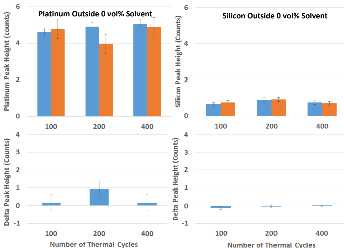
Figure 41: Before Cycling (blue bars, top row) and After Cycling (orange bars, top row) Comparison for 15.5V Electrical Bias Effects Outside Solvent Interaction Area for 100, 200 and 400 Cycles. Changes in Platinum (left column) and Silicon (right column) Values are Shown from EDS Data in Figure 36. Bottom Row Shows Delta Values between Before and After.
