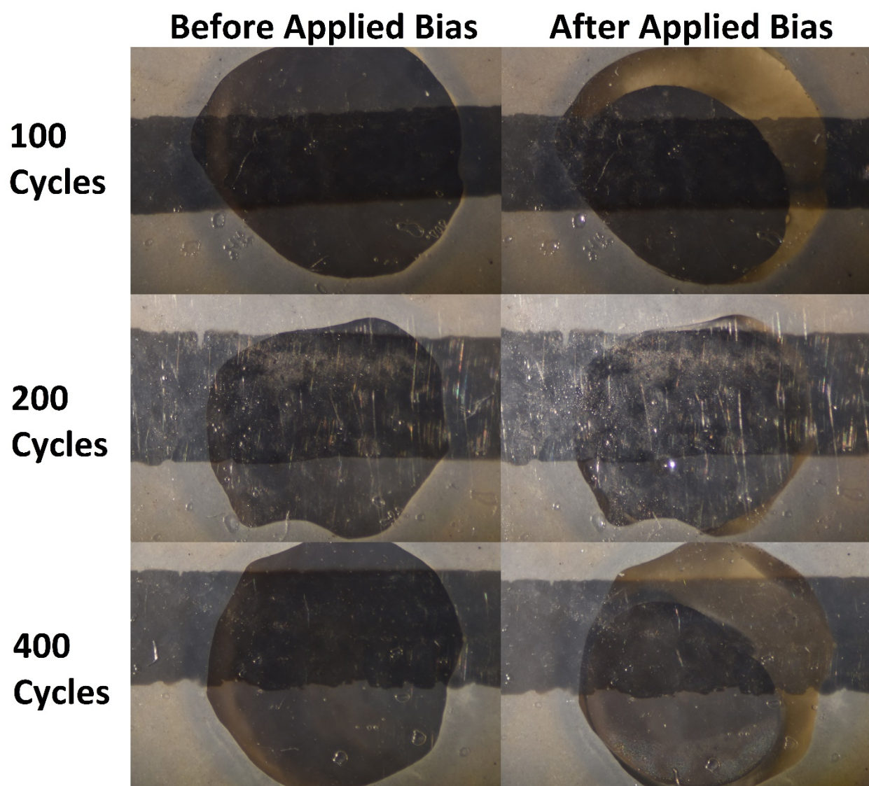
Figure 45: Optical Microscopy Images of Platinum Sputter Coated on PEM Material Samples Before (left column) and After (right column) on Samples with a 0.8V Electrical Bias Applied for 100 (top row), 200 (middle row) and 400 (bottom row) Cycles in Contact with 5 vol% Acetic Acid Solvent at Room Temperature.
