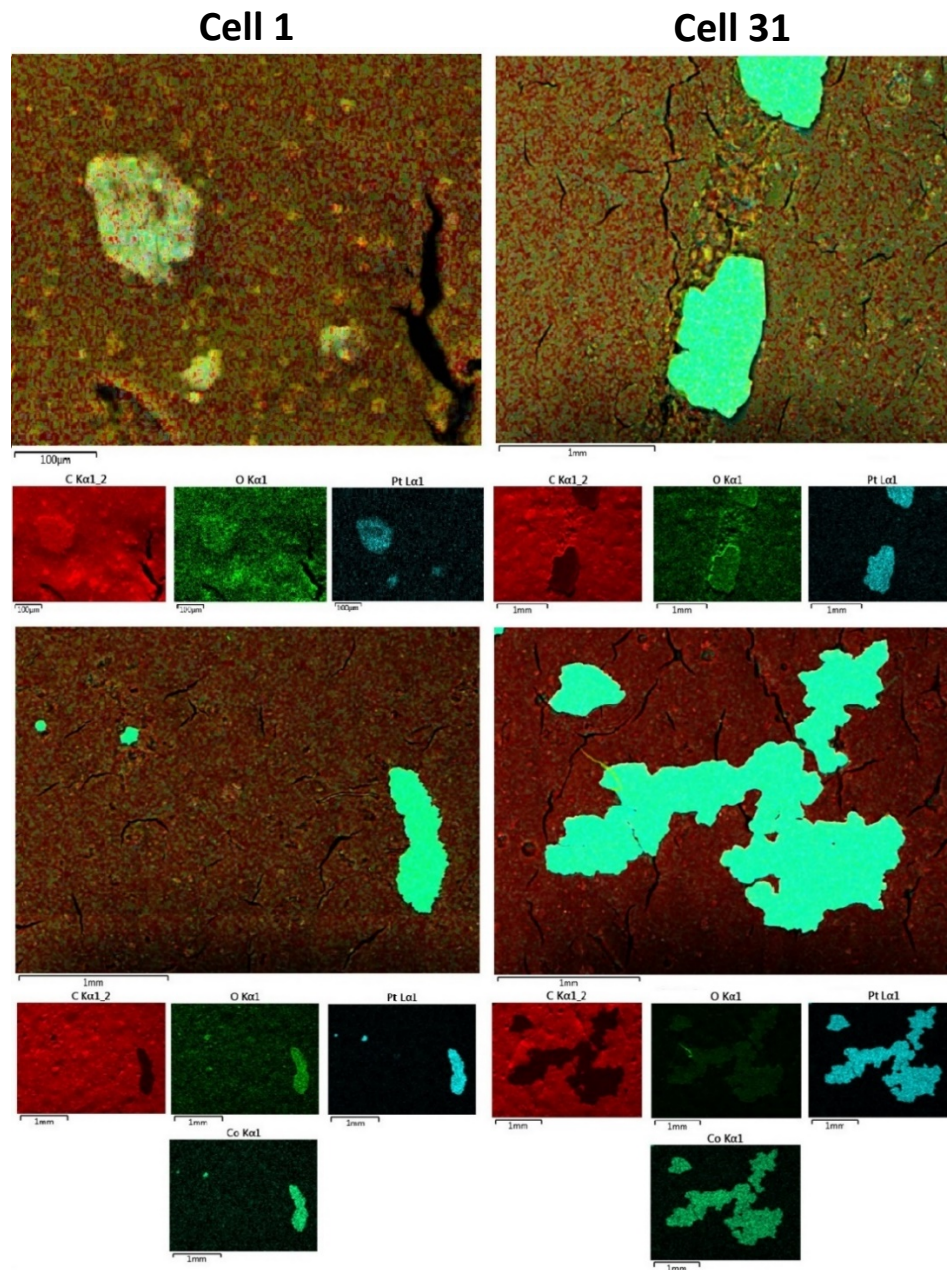
Figure 25: Cell 1 Cathode (top left)/Anode (bottom left) and Cell 31 Cathode (top right)/Anode (bottom right) Energy Dispersive Spectroscopy Platinum Electrocatalyst Elemental Map
