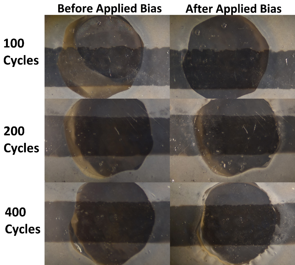
Figure 39: Optical Microscopy Images of Platinum Sputter Coated PEM Material Samples Before (left column) and After (right column) on Samples with a 15.5V Electrical Bias Applied for 100 (top row), 200 (middle row) and 400 (bottom row) Cycles in Contact with 99.7 vol% Acetic Acid Solvent at Room Temperature.
