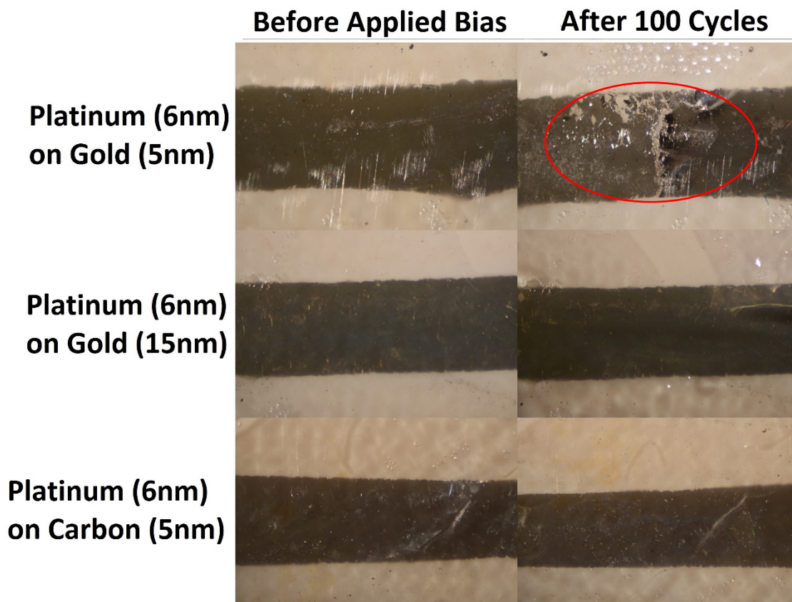
Figure 67: Optical Microscopy Images of Platinum/Gold and Platinum/Carbon Sputtered Coated on to PEM Material Substrates Before (left column) and After (right column) a 15.5V Electrical Bias was Applied for 100 Cycles in Contact with 5 vol% Acetic Acid. Gold was Applied at 5nm (top row) and 15nm (middle row) Thicknesses. Carbon was Applied at 5nm (bottom row) Thickness. Platinum was Applied at 6nm for all Experiments.
