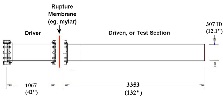
Figure F-1: Schematic of a Gas Driven Shock Tube.
