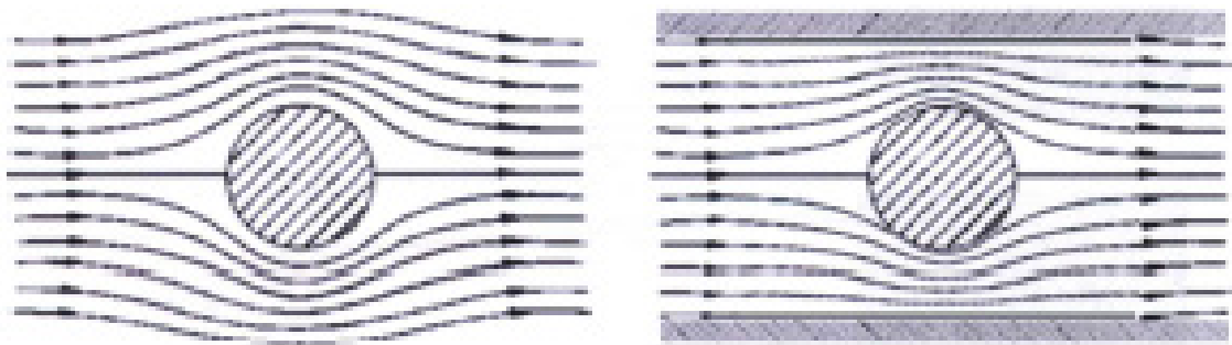
Figure F-7: Simulation Showing How Flow Field can be Perturbed by Blocking a Large Portion of the Tube with the Test Subject (from Dyn-FX Consulting Ltd.).
