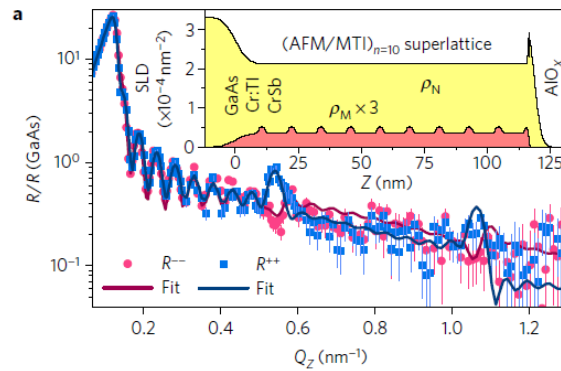
Figure 4 Polarized neutron reflectivities (at 20 K with a 700mT in-plane field) normalized to the GaAs substrates for the spin-polarized R^{++} and R^{--} channels of an (\text{AFM/MTI})_{n=10} . The insets show the
