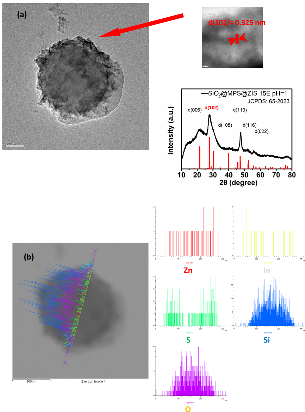
Figure 8. (a)lattice analysis and XRD pattern (b)line scan of \text{SiO}_2@\text{MPS}@\text{ZIS} synthesized in ethanol solution.
