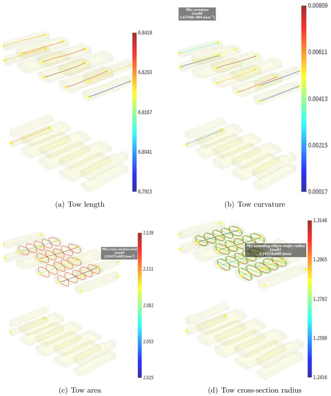
Figure G.6: Warp Carbon tows characterization.
