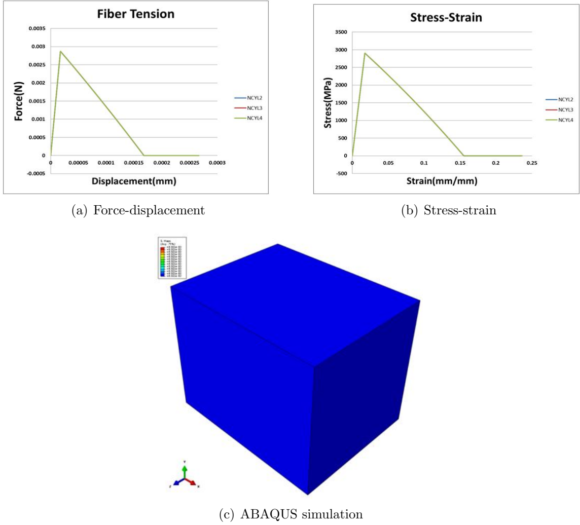
Figure 3.20: Fiber tension (1).
