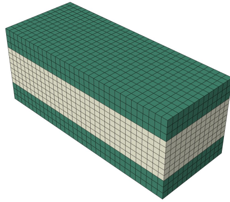
(a) Mesh-1 (5577 elements).
