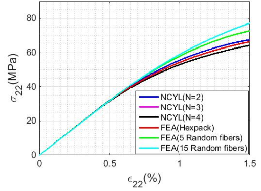
(b) Transverse normal stress versus strain response
