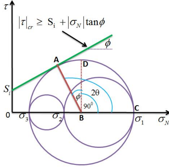
Figure 6.4: Mohr-Coulomb's criterion.
