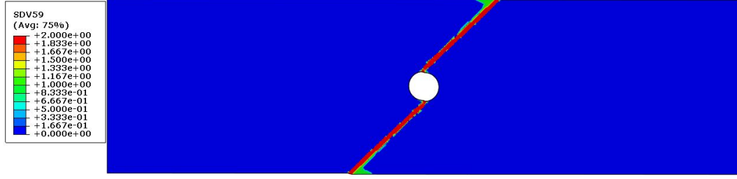
Figure 3.31: Matrix cracking captured in 45^\circ ply.
