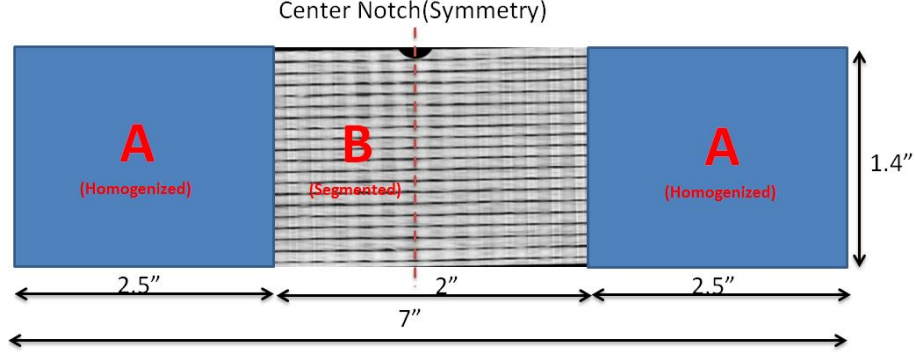
Figure 6.38: Geometric dimensions of the notched compression coupon.
