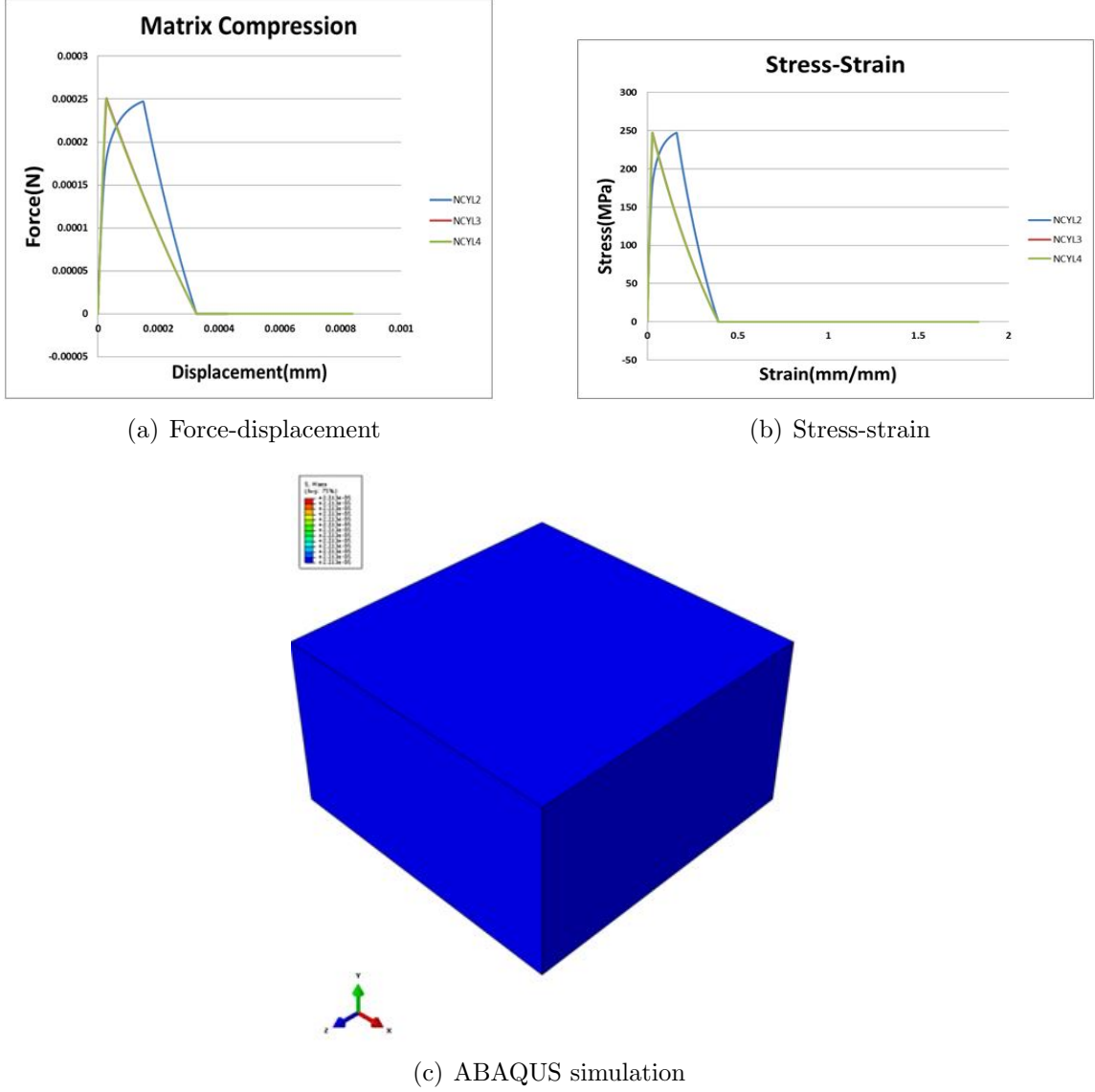
Figure 3.23: Matrix compression (2).
