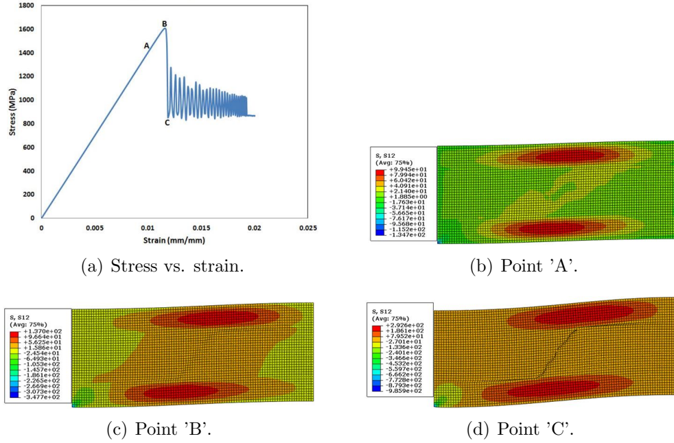
Figure 6.10: Progressive contour plots of shear stress.
