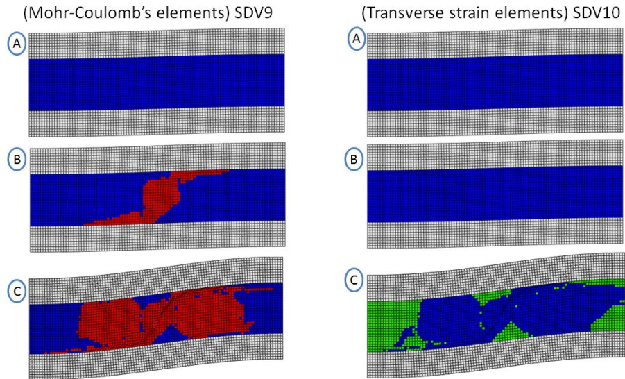
Figure 6.15: Progressive kinking-splitting plots for 0.1^\circ (Case-A).
