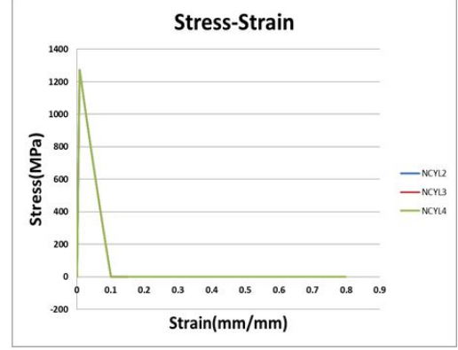
(b) Stress-strain
