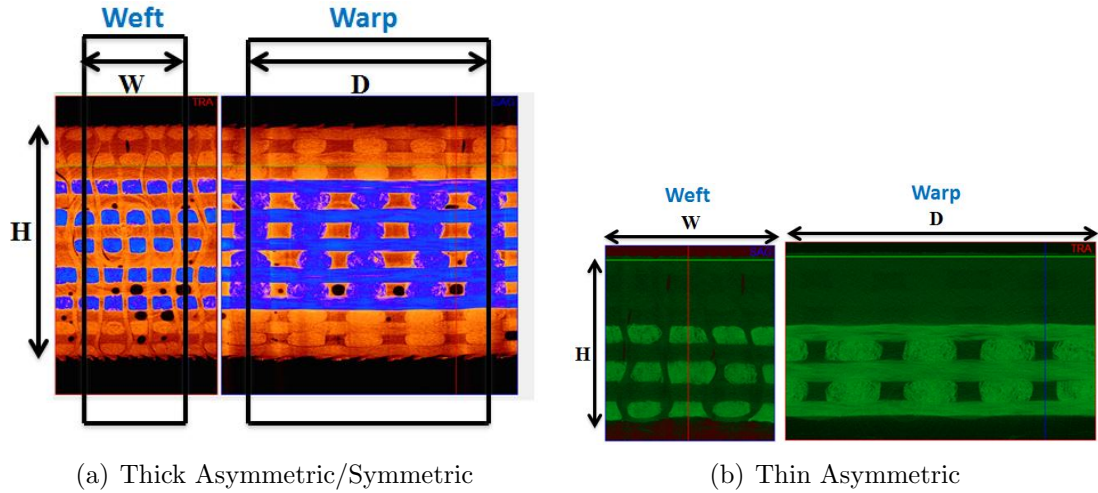
Figure 4.5: Micro-CT analysis to determine RVE.
