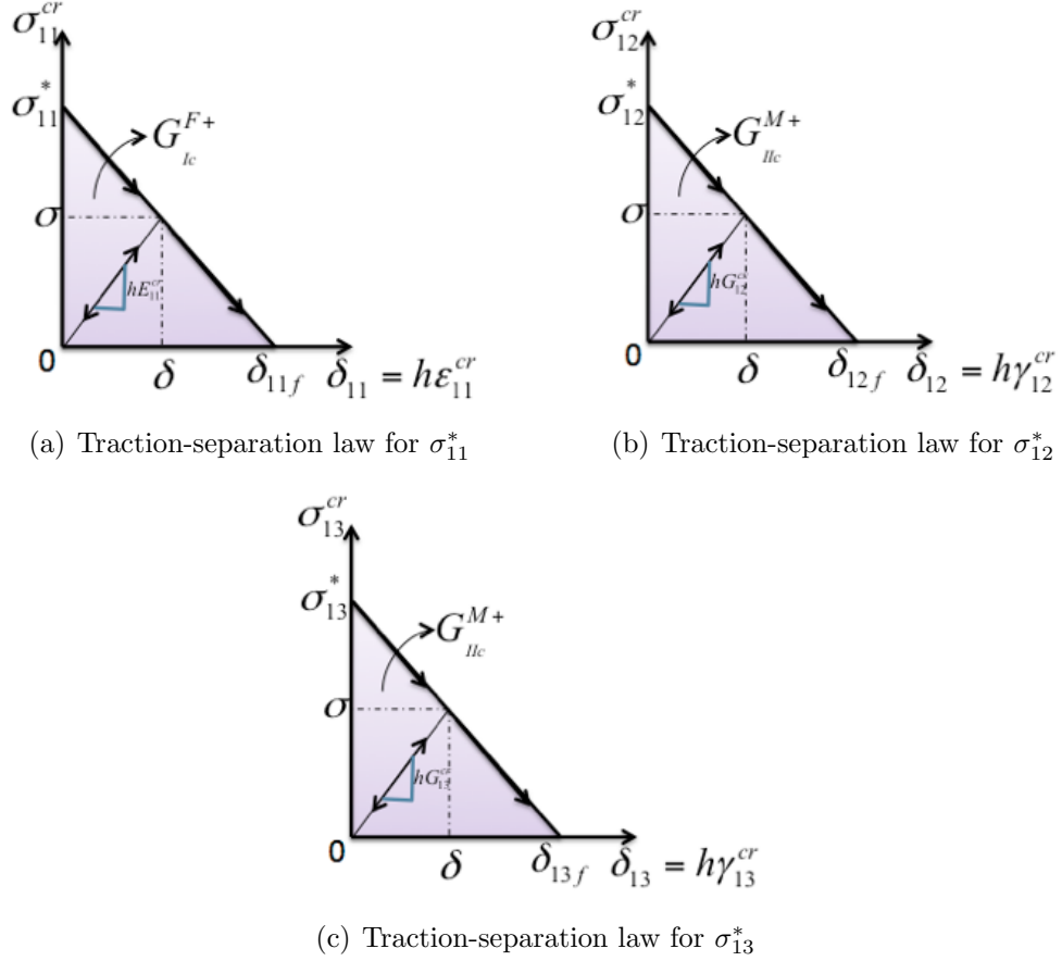
Figure 3.8: Traction-separation laws for fiber tensile failure.
