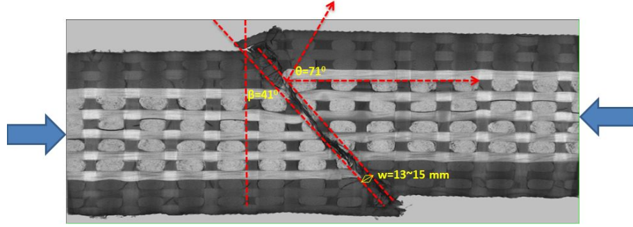
Figure 6.27: Measurement of kink band angle from Micro-CT study.
