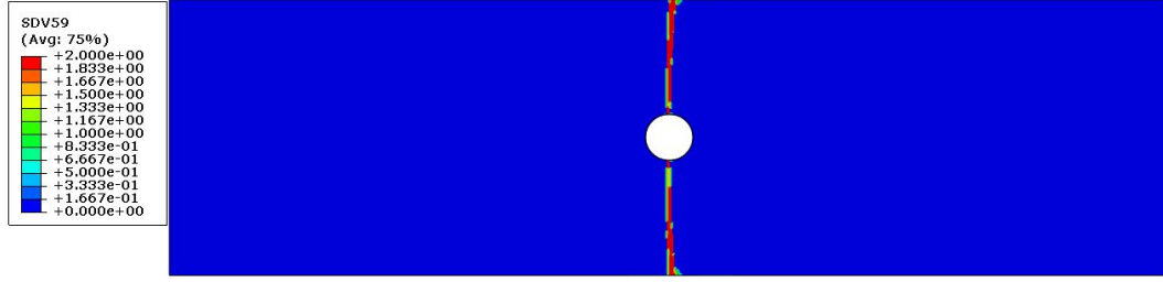
Figure 3.32: Matrix cracking captured in 90^\circ ply.
