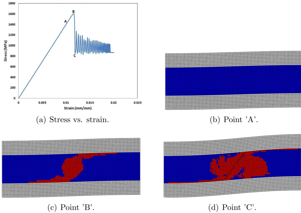
Figure 6.11: The cracked elements are shown in red.
