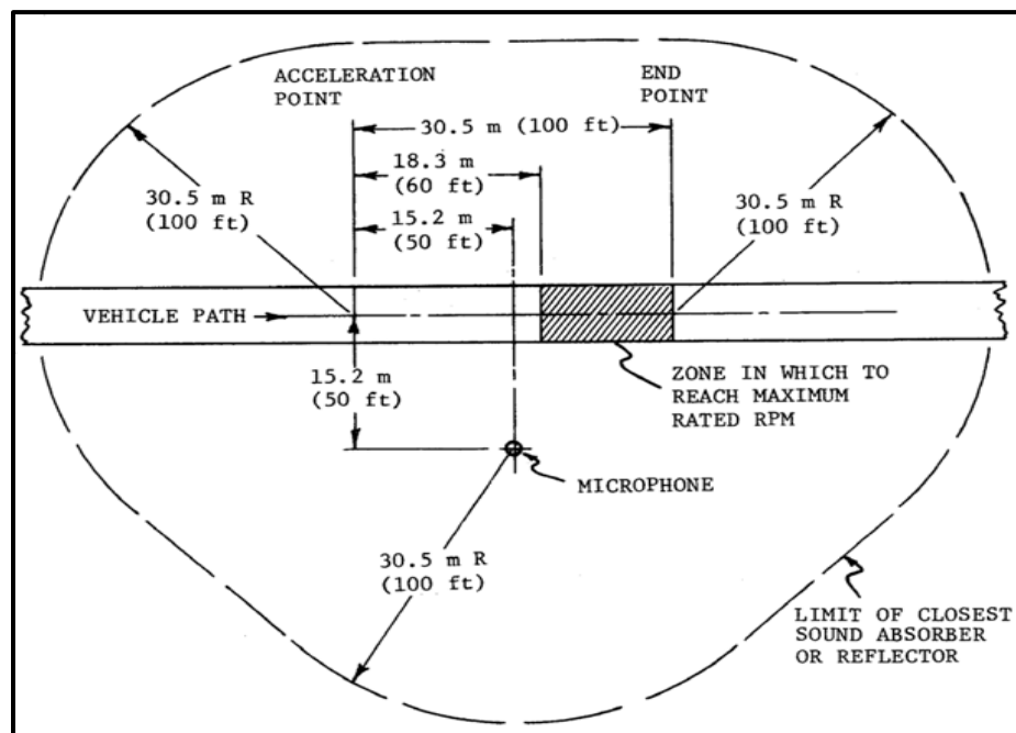
Figure 2. Motor vehicle drive-by noise test setup (SAE J366).
