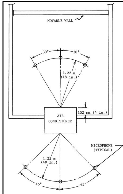
Figure 1. Air conditioner test setup.
