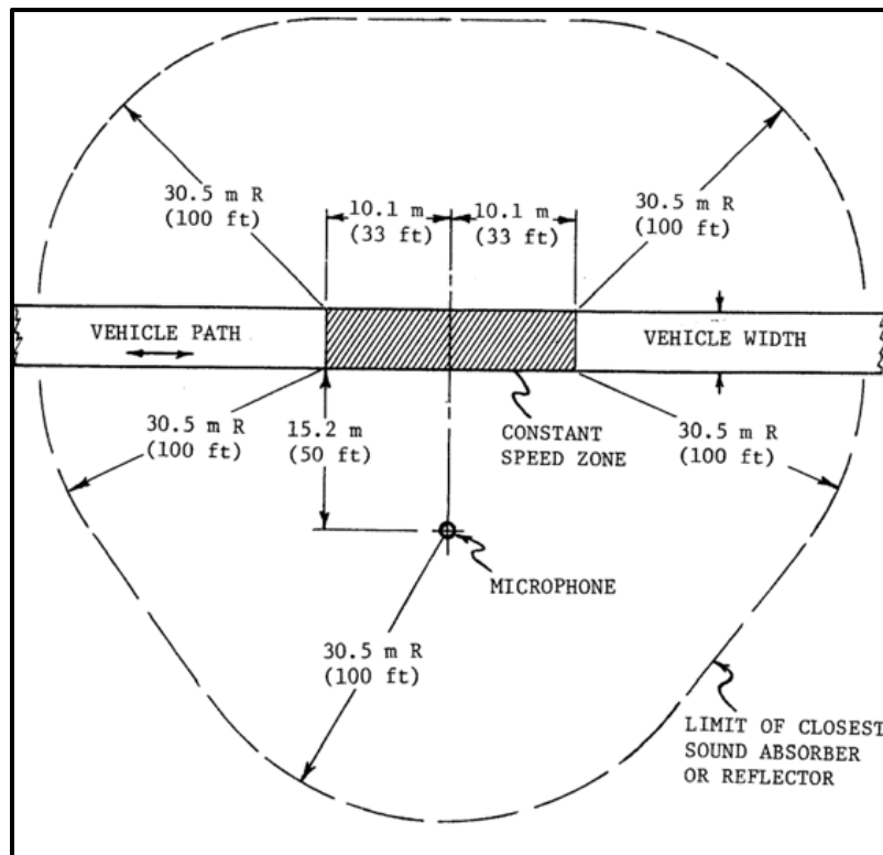
Figure 3. Powered mobile-construction-equipment drive-by noise test (SAE J88).
