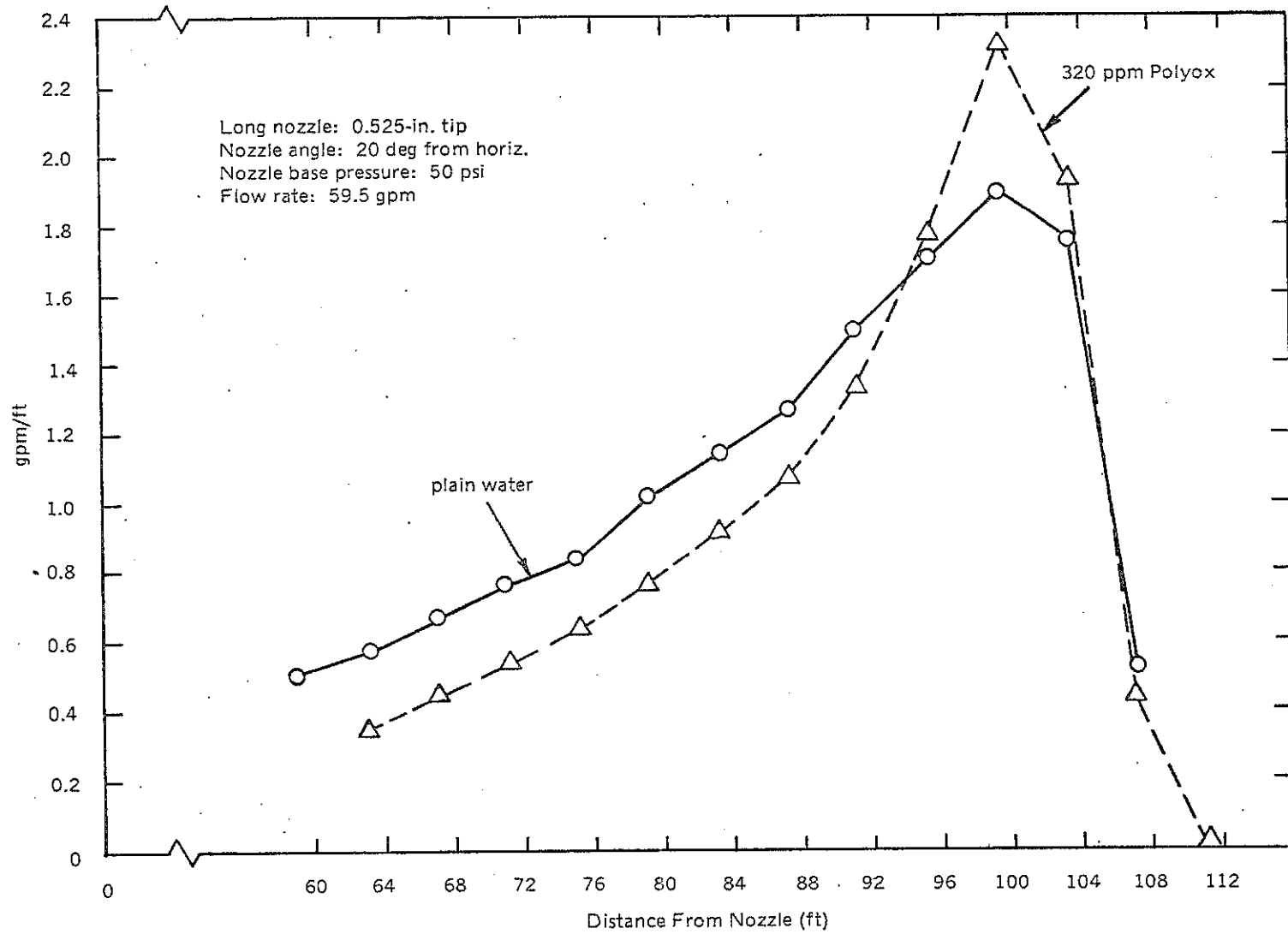
Delivery Pattern (gpm/ft of range) vs Distance From Nozzle
