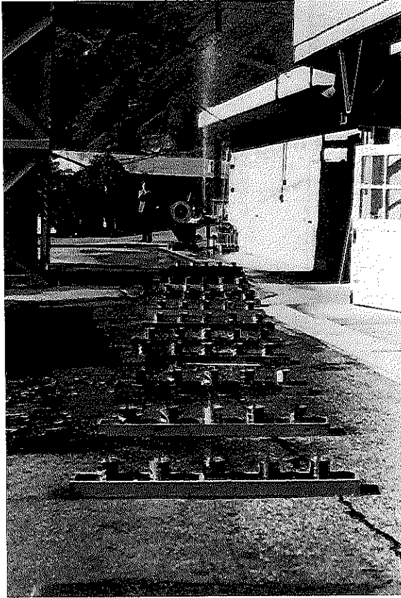
FIG. 6. Sampling Can Pattern. Five Cans per Row with 10-inch Spacing. Thirteen Rows with 4-foot Spacing Between Rows. (Left) Looking Upstream. (Right) Looking Downstream.
