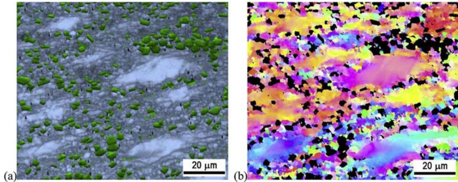
Fig. 11. EBSD images of \text{Re}_{10}\text{Nb}_{10}\text{Ti}_{10}\text{Zr}_{10} alloy after 55% compression deformation at 1000 °C: (a) Combination of image quality and phase maps (BCC matrix is light-blue and Laves precipitates are green); (b) inverse pole figure map of the BCC matrix (the secondary precipitates are black). (For interpretation of the references to color in this figure legend, the reader is referred to the Web version of this article.)
