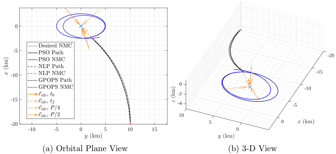
Figure 26. Problem B-2, All Model Solutions, Hard Sunlight Constraint, t_f = 1.5 hrs
