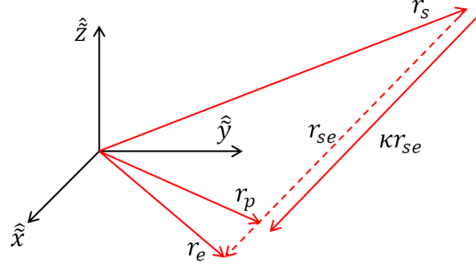
Figure 51. General Terminal Conditions for Obtaining the Sun Vector
